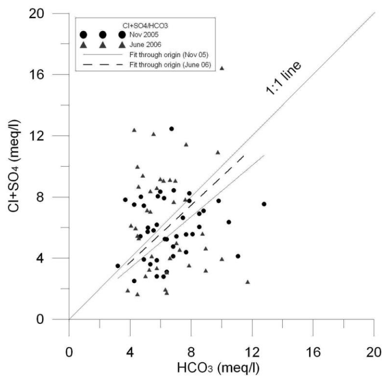
Fig.6.4 Relative abundances of HCO 3 and Cl+SO 4 .
