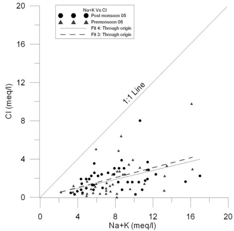
Fig.6.5 Showing bonding affinity between Alkalis and Cl.
