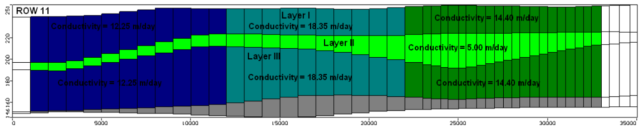
Fig.4.6a Hydrogeological cross section along row 11 showing three layer system.
