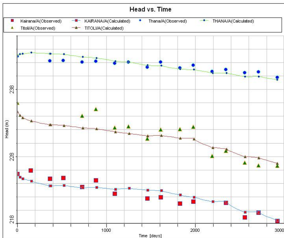
Fig.4.10a Observed and simulated heads at Kairana, Titoli and Thanabhawan.
