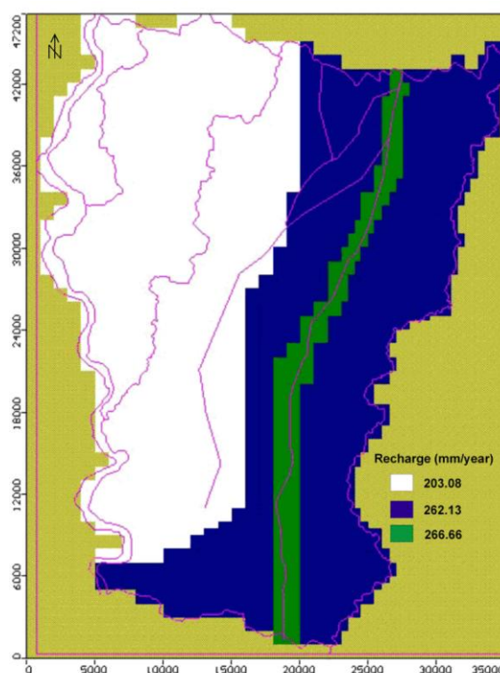
Fig.4.2 Zone wise recharge distribution in Yamuna-Krishni model.
