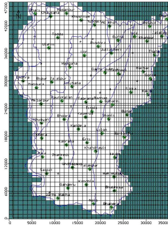
Fig.4.5 Grid pattern and location of observation wells in Yamuna-Krishni sub-basin.
