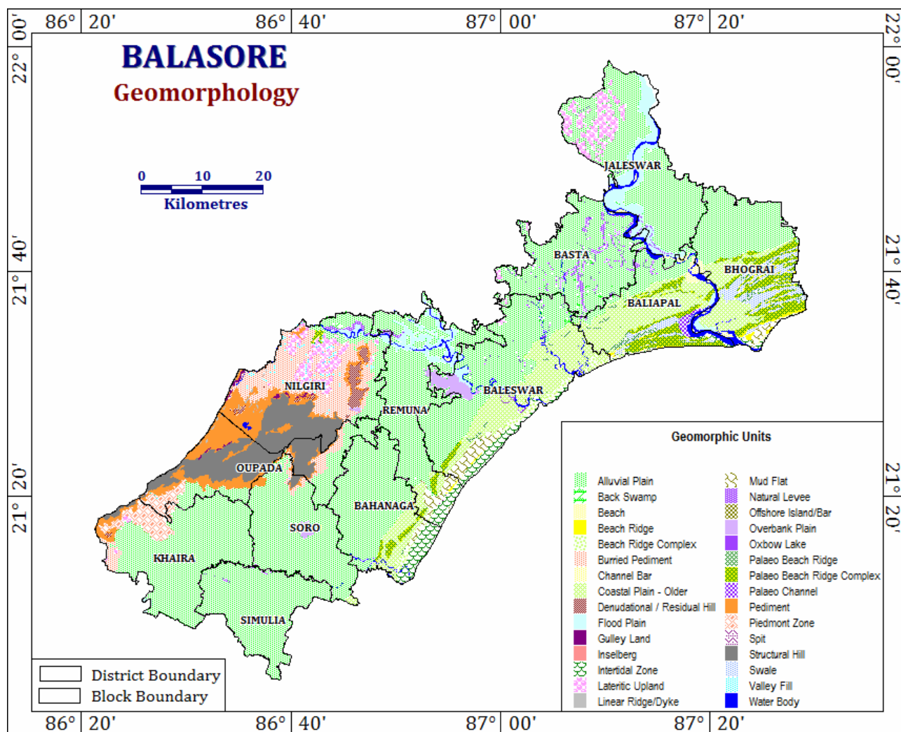
Figure – 3.3 : Geomorphological map of Balasore District, Odisha
