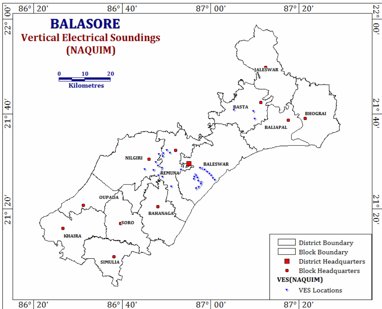
Figure – 5.2 a : NAQUIM VES Locations in Balasore District, Odisha
