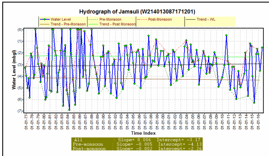
Figure – 5.1.6 c : Hydrograph of Jamsuli(Baliapal Block)
