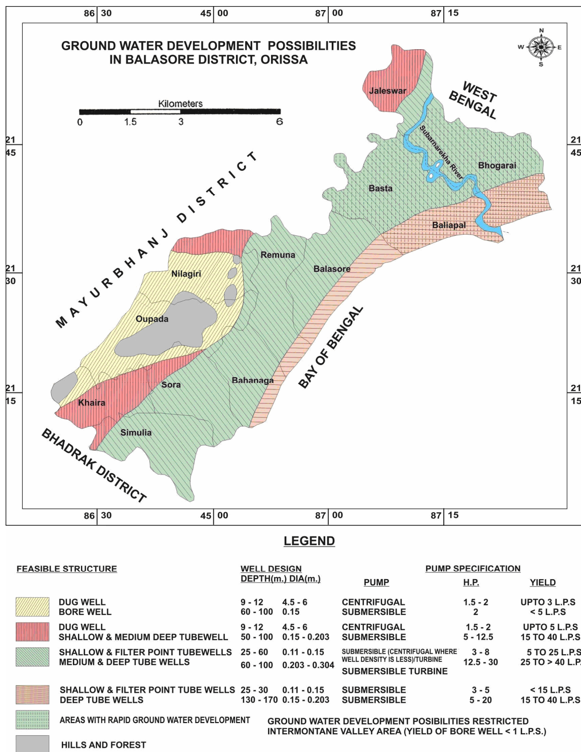
Figure 7.1 c: Ground Water Development Possibility in Balasore District, Odisha
