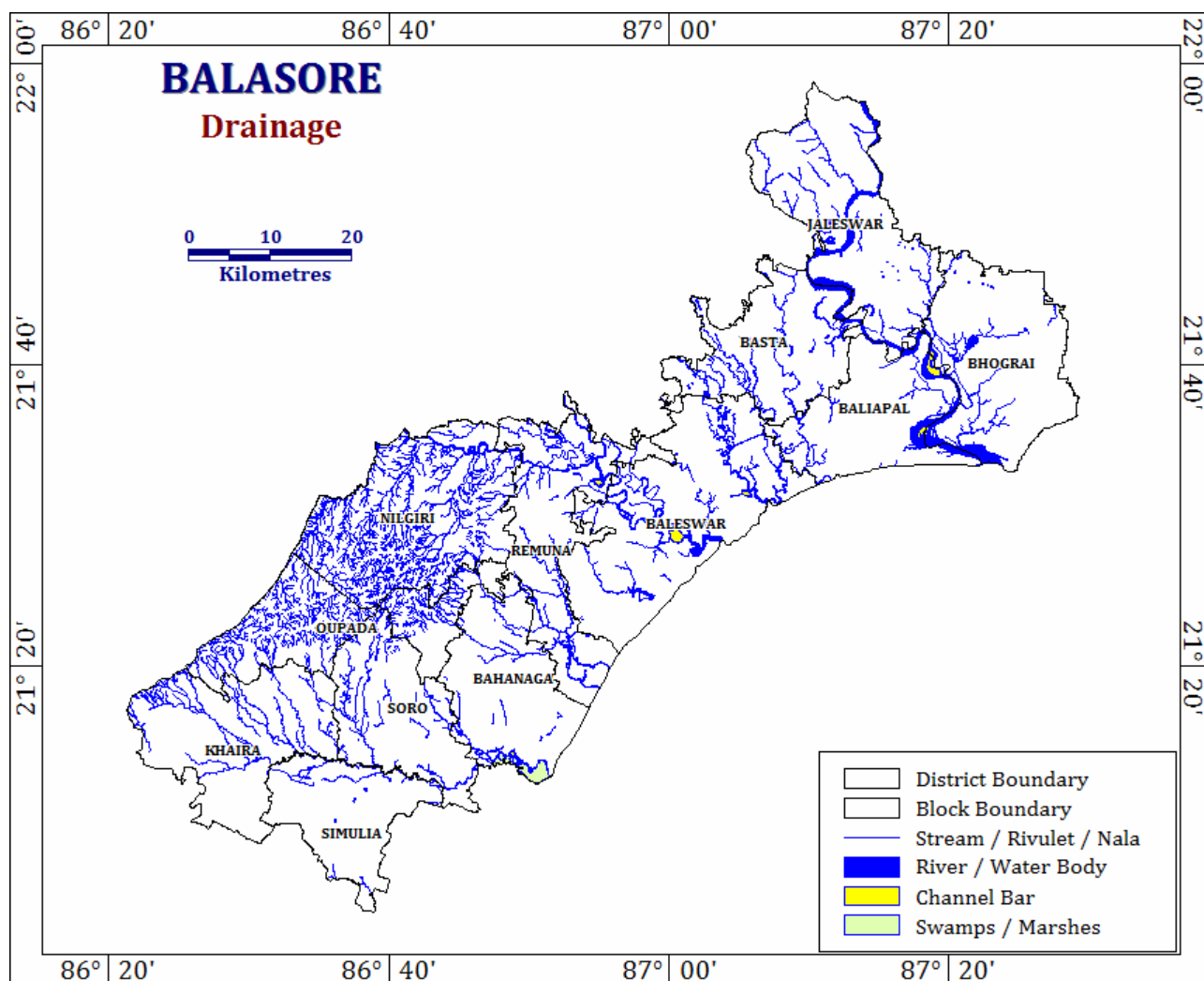
Figure – 3.2 : Drainage Map of Balasore District, Odisha
