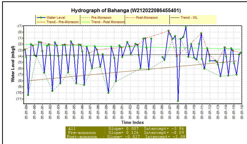
Figure – 5.1.6 a: Hydrograph of Bahanaga(Bahanaga Block)
