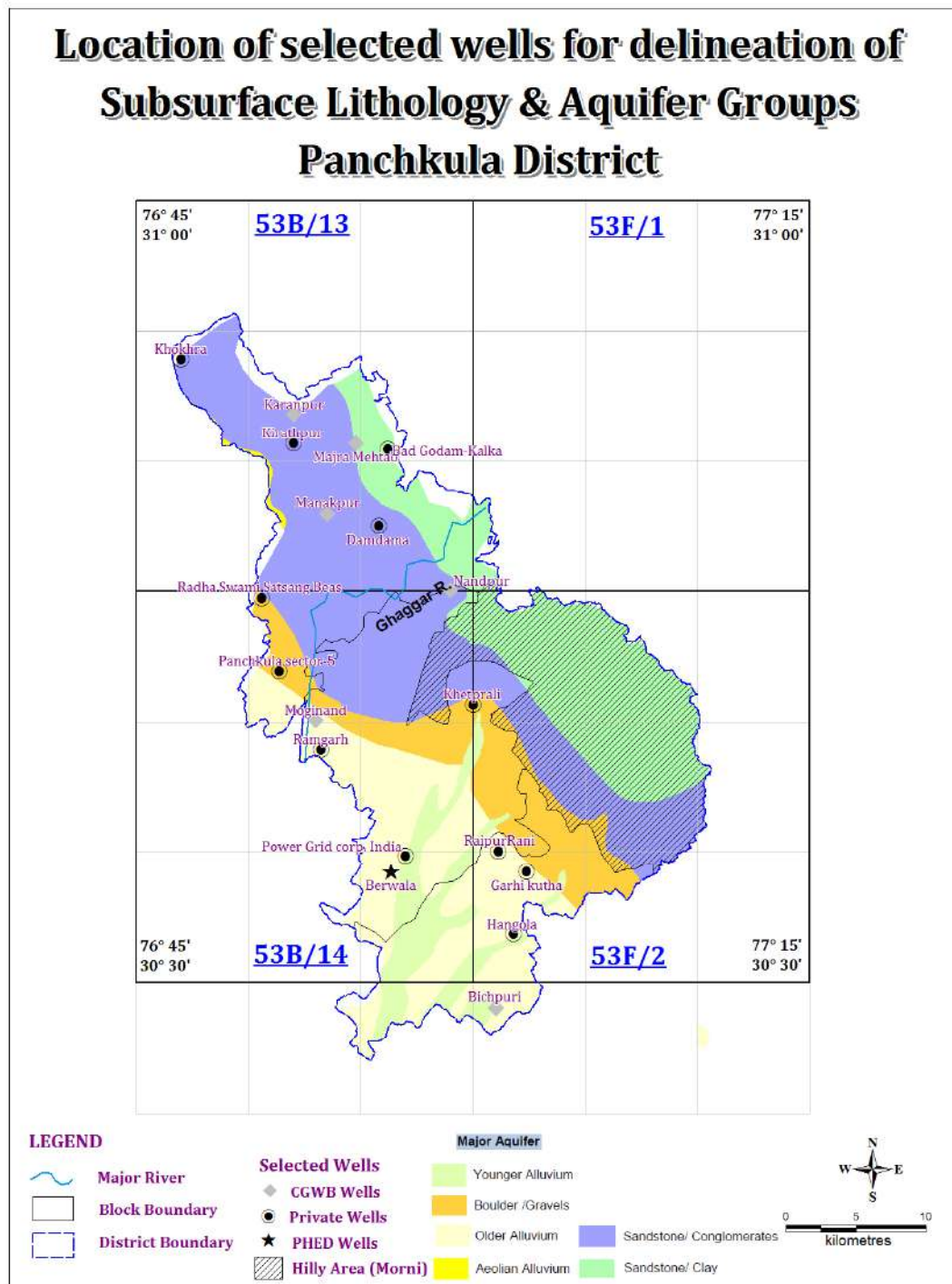
Fig 11: Validated Exploration Data of Panchkula District
