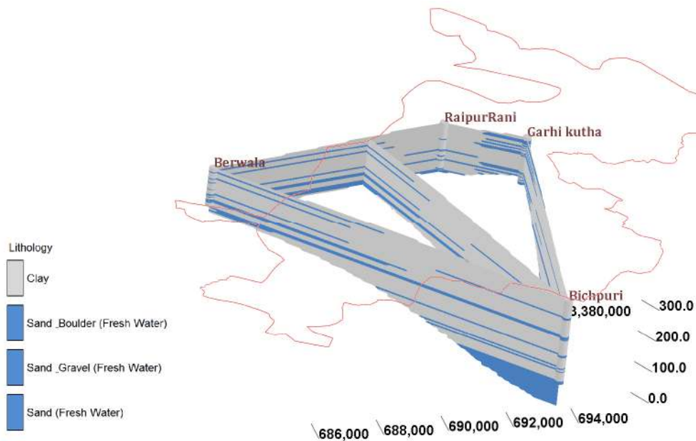
3D Lithology Fence
