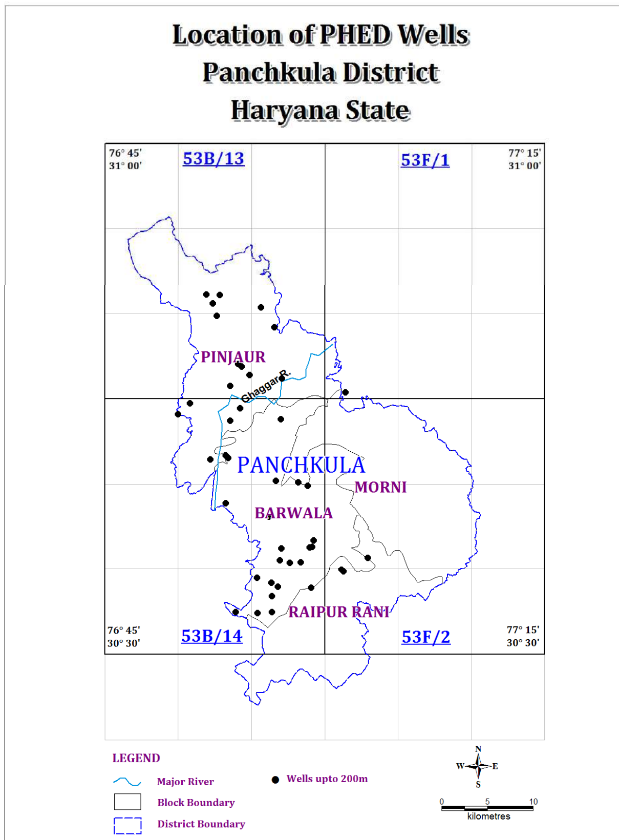
Fig 9: Location of PHED wells
