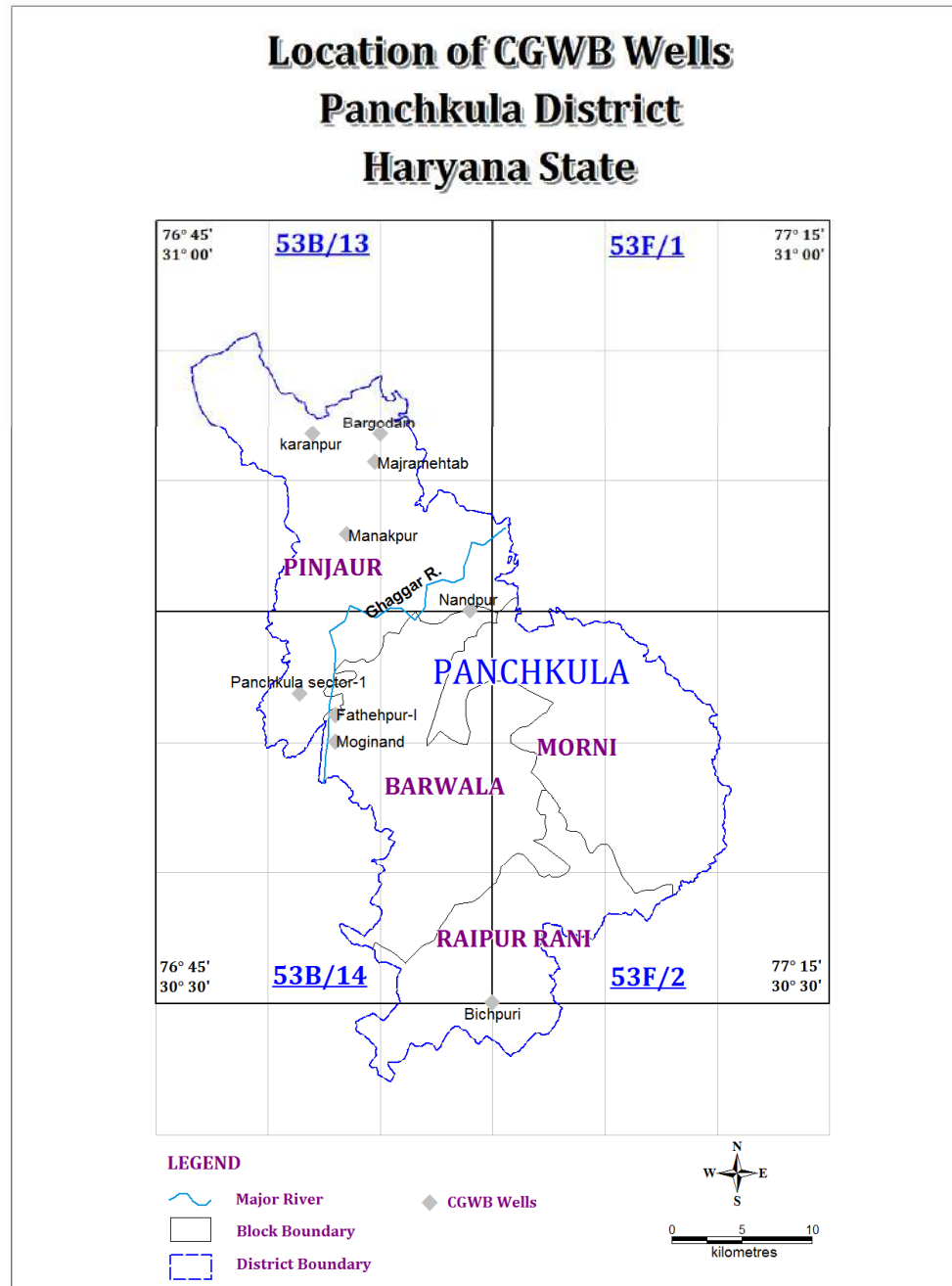
Fig 8: Location of CGWB wells
