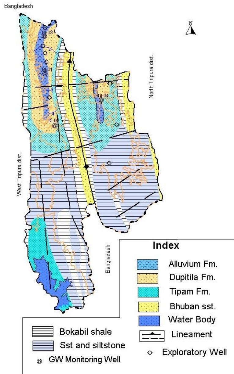
Fig 6: Hydrogeology, Dhalai district
