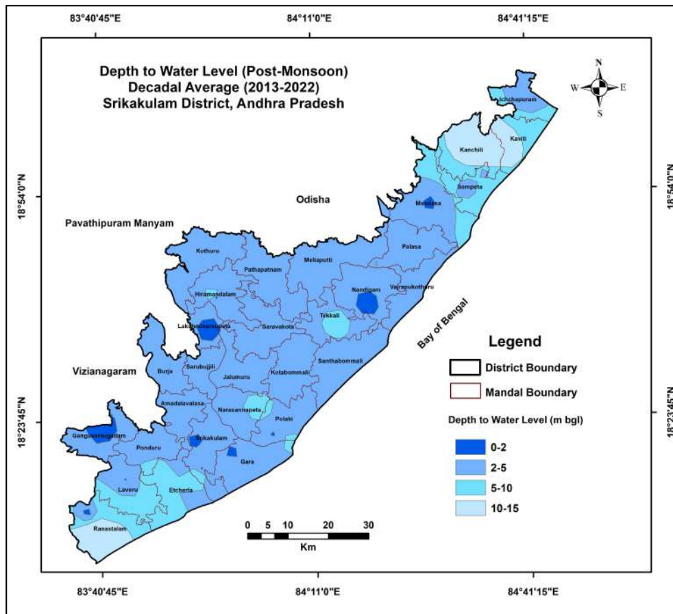
Fig.2.6: Depth to water levels Post-monsoon (Decadal Average).
