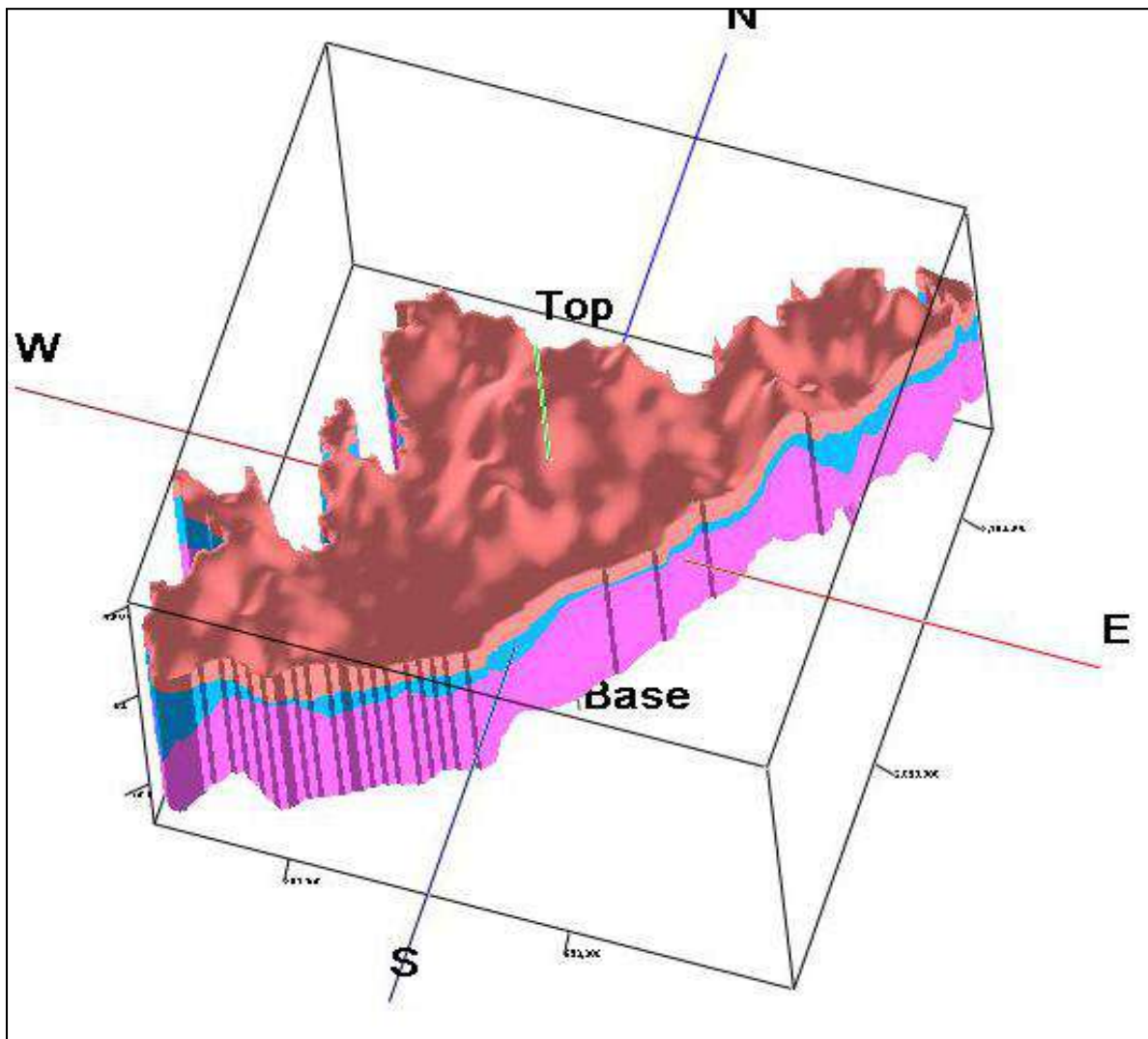
Fig.-3.1: 3D Aquifer Disposition of Srikakulam District.
