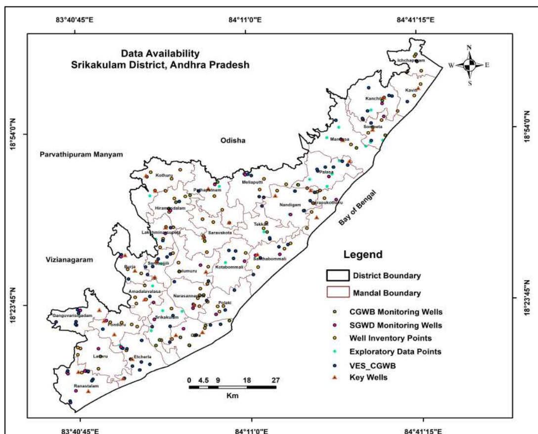
Fig. 2.1: Hydrogeological data availability.
