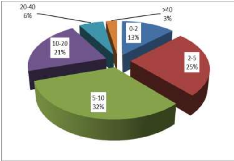
Fig.7.3: Percentage of wells in different depth ranges of DTW-August 2019
