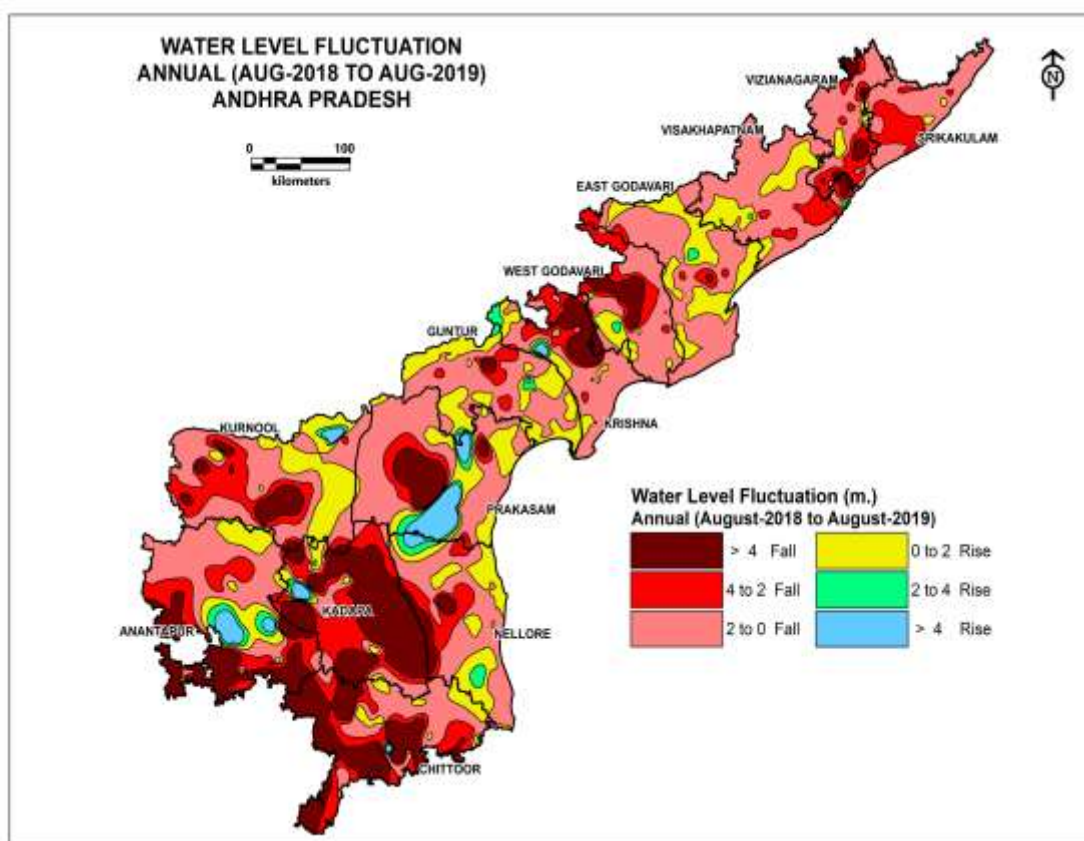
Fig. 7.15: Water Level Fluctuations (August 2018 from August 2019)
