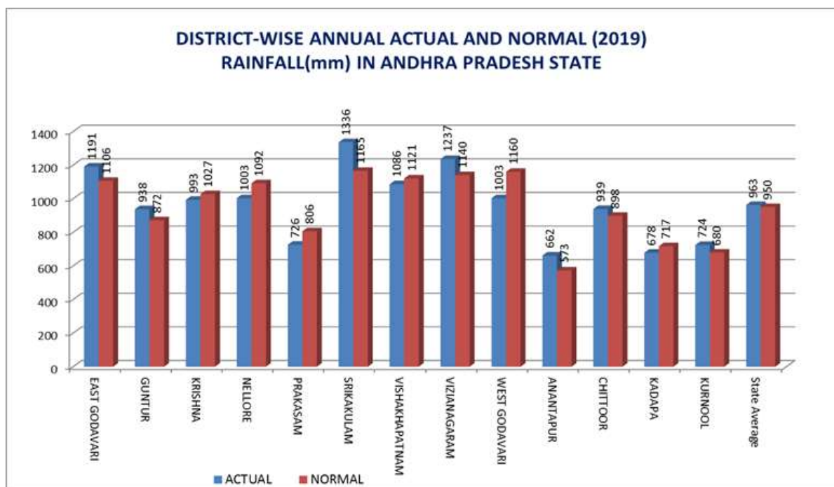
Fig.3.1: District-wise Annual Actual and Normal (2019) rainfall.
