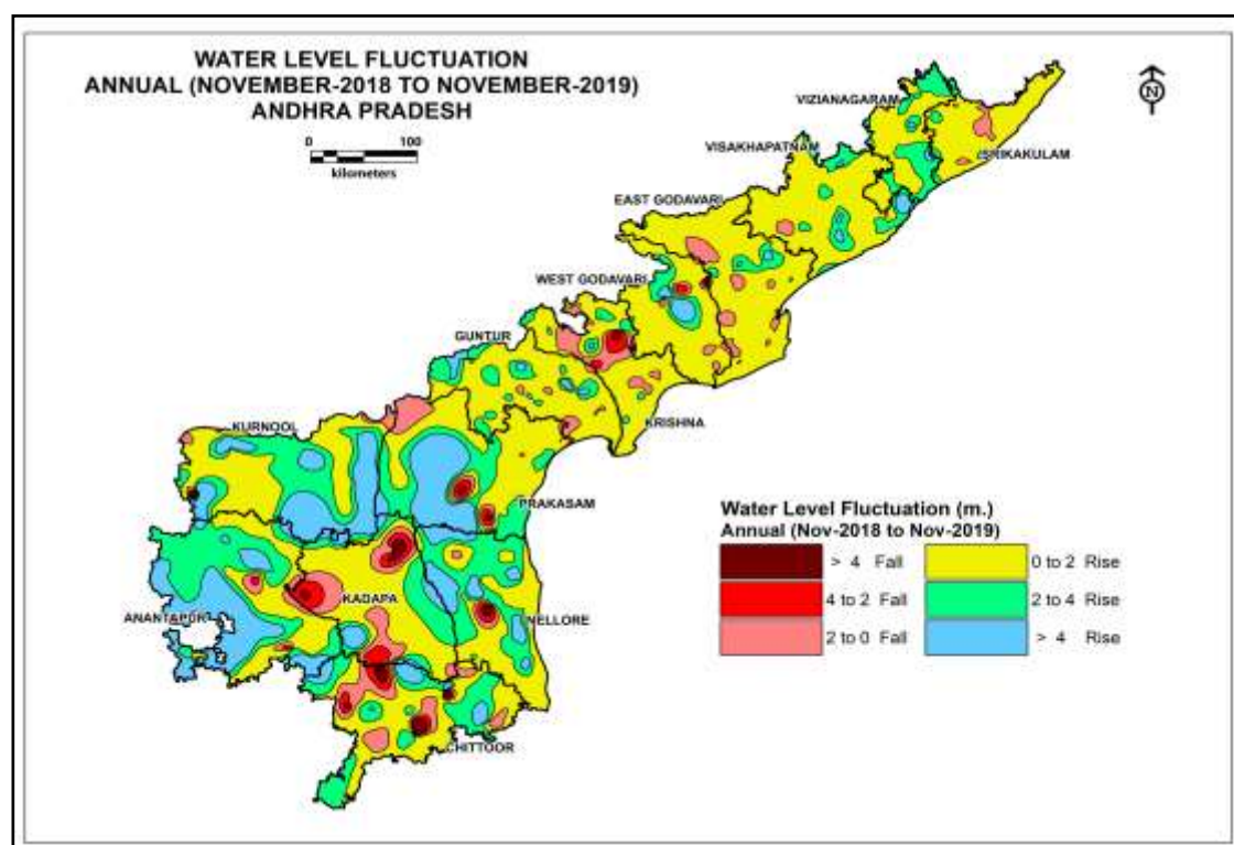
Fig.7.16 : Water Level Fluctuations (November 2019 from November 2018)
