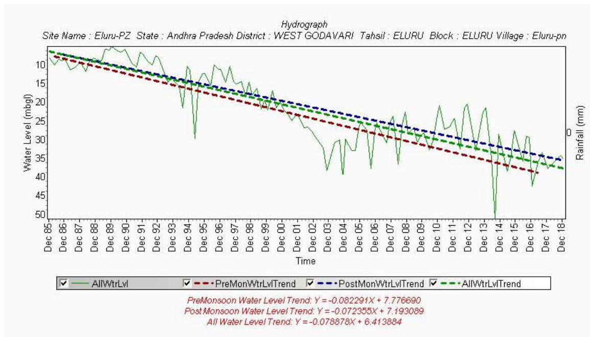
Fig.7.24 (7.24a to 7.24z): Representative Hydrographs from Andhra Pradesh State.
