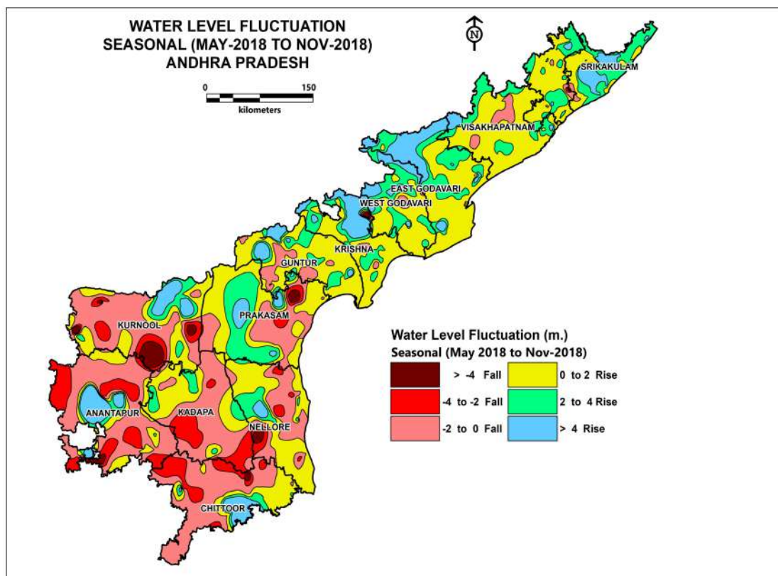
Fig 7.12 Water Level Fluctuation (Nov, 2018 from May, 2018)
