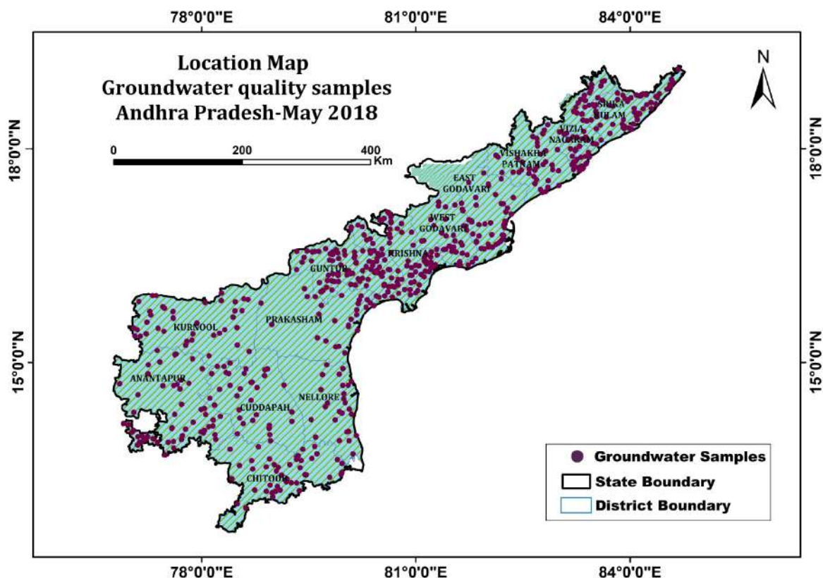
Fig.8.1: Location of Ground water sample sites in Andhra Pradesh
