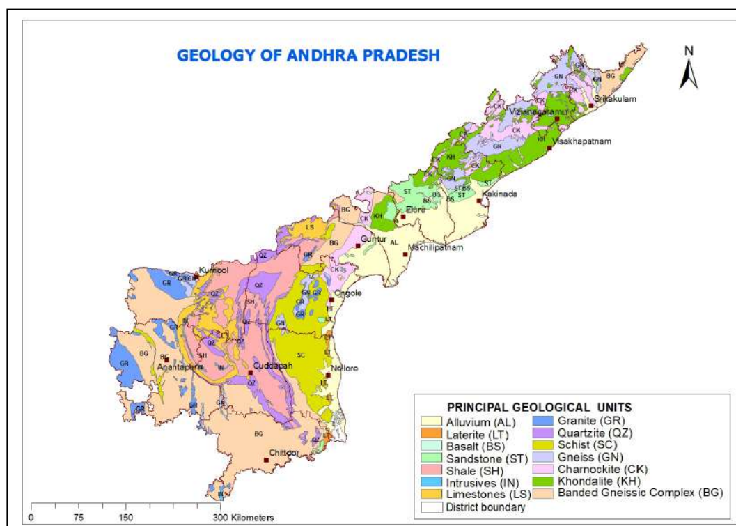
Fig.4.1: Geology of Andhra Pradesh State
