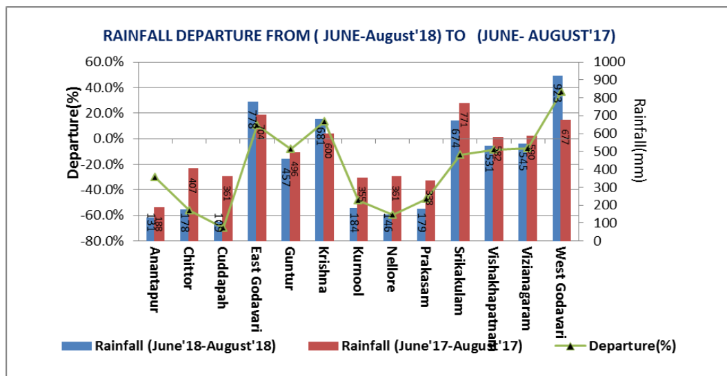
Fig.3.5: Rainfall Departure (June, 2018-Aug,2018 from June, 2017-Aug,2017).
