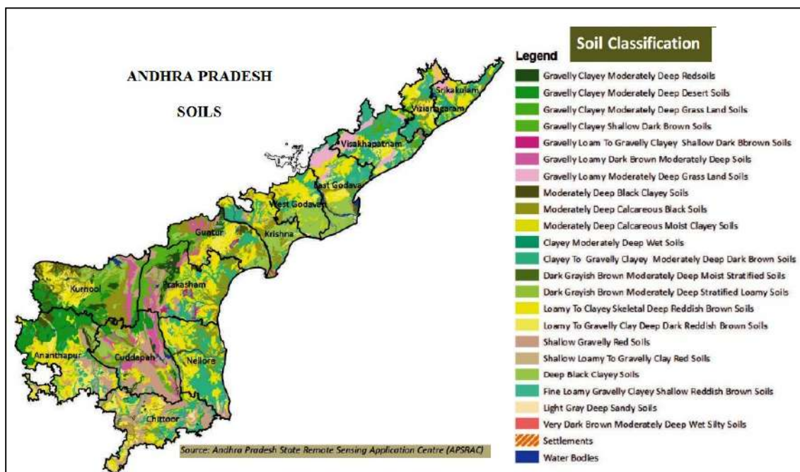
Fig.2.3: Soil Map of Andhra Pradesh (after APSRA-2014).
