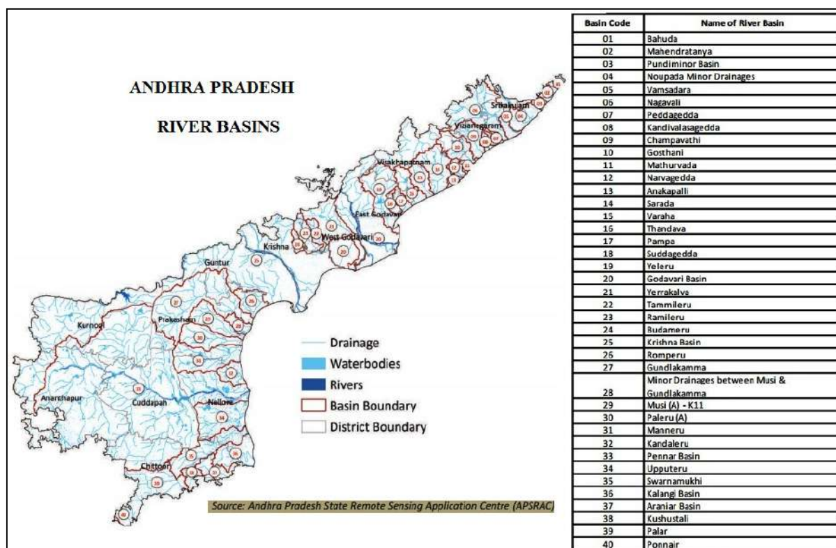
Fig.2.2: Drainage and River sub-basin map of Andhra Pradesh State. (After APRAC-2014).
