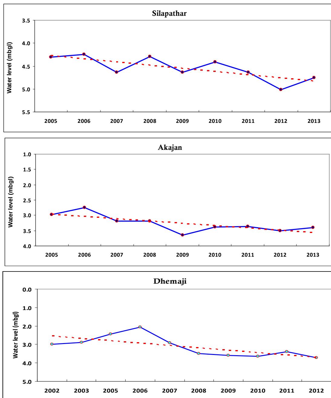
Fig.3.8: Pre-monsoon Hydrograph of GWMS wells
