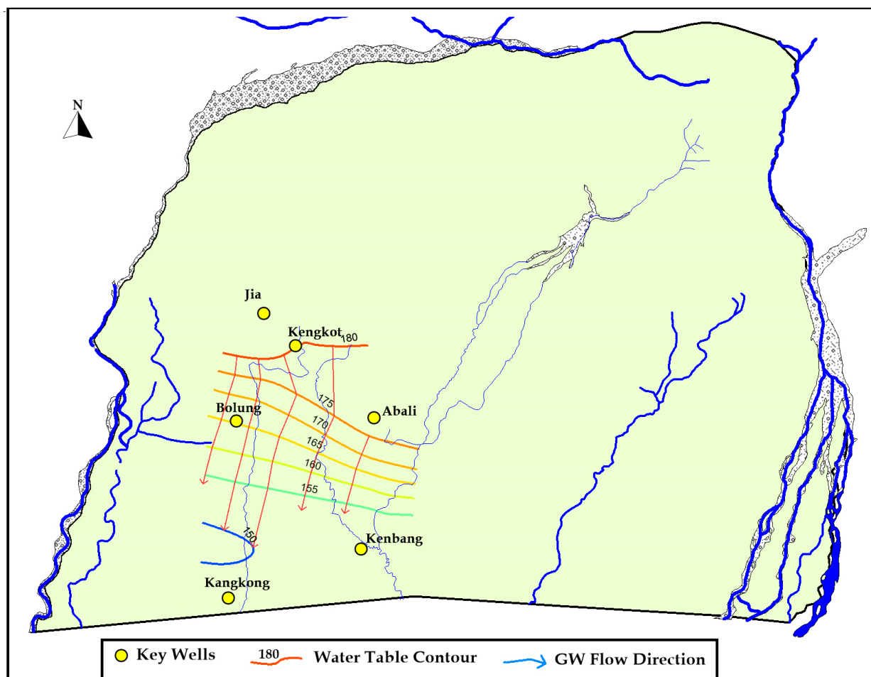
Fig. 3.41: Hydrogeological Map of the study area.
