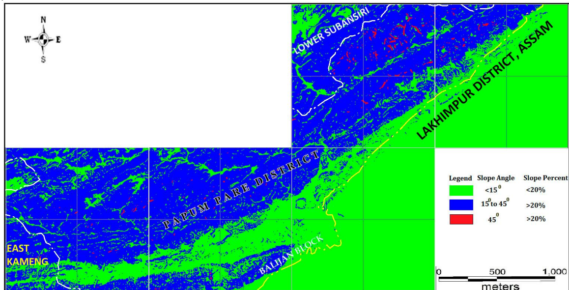
Fig. 4.1: Slope map showing recharge worthy area of the study area with less than 20% slope. The computation of ground water resources available in the district has been done using GEC 1997 methodology.
