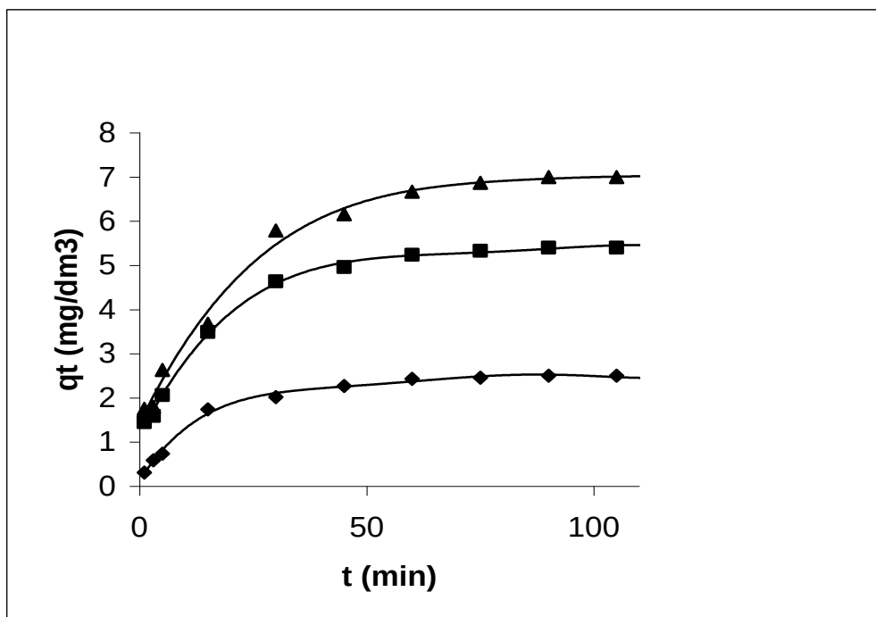
Fig.6: Kinetic data for fluoride adsorption on IZHO at 303 ( \pm 2 )K and pH 6.8 ( \pm 0.1 ) Initial fluoride concentration (mg/dm³) used: \blacklozenge 5.0, \blacksquare 12.5 and \blacktriangle 25.0
