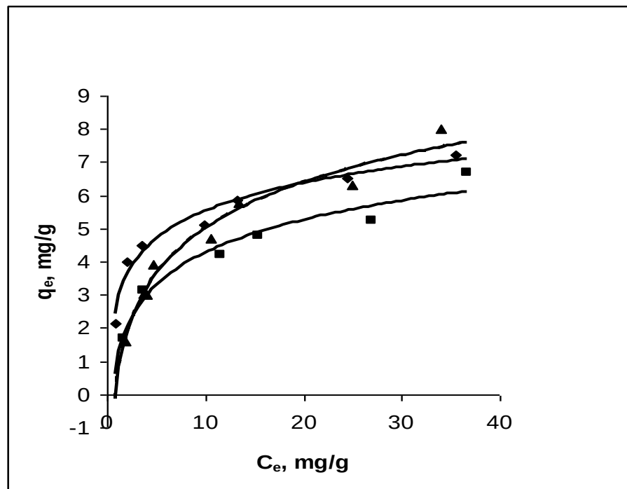
Fig.5b: The equilibrium isotherm data of fluoride sorption at final pH 6.8( \pm 0.2 ) and at 293( \pm 2 )°K by ◆ HZFO, ■ HFO and ▲ HZO.
