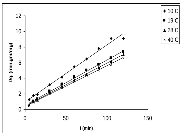
Fig.8a: The pseudo-second order kinetic plot for fluoride adsorption onto iron(III)-aluminum(III) mixed oxide at different temperatures. Initial fluoride concentration: 50.0 mg L -1 , pH: 6.9 ( \pm 0.2 ).
