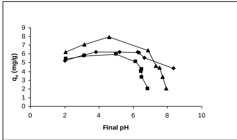
Fig. 4: The plot of fluoride sorption data versus final solution pH at 303 ( \pm 2 ) °K by \blacklozenge HZFO, \blacksquare HFO and \blacktriangle HZO. Initial Fluoride load used was 10.0 mg/g hydrous oxide.
