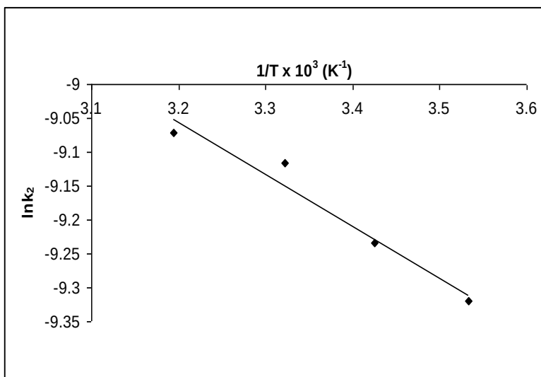
Fig. 9: The plot of \ln k_2 versus 1/T for an initial fluoride concentration of 50.0 mg L -1 and pH 6.9 (±0.2).
