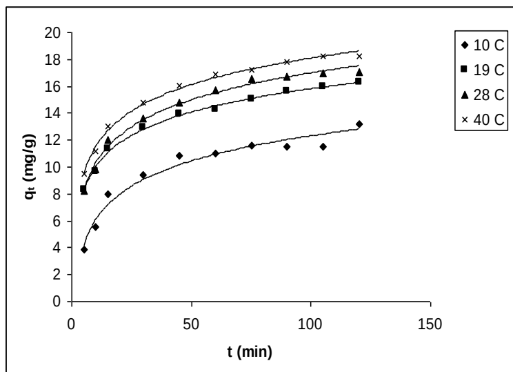
Fig.8: The plot of adsorption capacity, q_t (mg.g -1 ) versus time, t (min) at different temperatures. The initial fluoride concentration: 50.0 mg L -1 , pH: 6.9 ( \pm 0.2 ).
