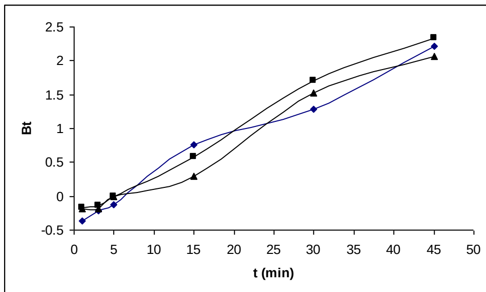
Fig. 11: Boyd kinetic plots on the adsorption of fluoride on IZHO at pH 6.8 ( \pm 0.1 ) and at 303( \pm 2 ) K. Initial fluoride concentration ( \text{mg/dm}^3 ) used: \blacklozenge 5.0, \blacksquare 12.5 and \blacktriangle 25.0.
