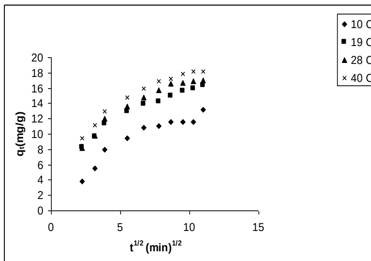
Fig.8b: Intra-particle diffusion plot for fluoride adsorption onto iron(III)-aluminum(III) mixed oxide at different temperatures. Initial fluoride concentration: 50.0 mg L -1 , pH: 6.9 (±0.2).
