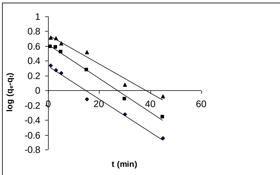
Fig. 7: Pseudo-first order kinetic plot for fluoride adsorption data on IZHO at 303 ( \pm 2) K and at pH 6.8 ( \pm 0.1). Initial fluoride concentration ( \text{mg}/\text{dm}^3 ) used: \blacklozenge 5.0, \blacksquare 12.5 and \blacktriangle 25.0.
