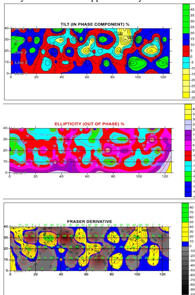
Fig.6: Contour Maps generated based on Parallel VLF Profiles at Ghorad, Chandrabhaga Watershed (WGKKC-2)
