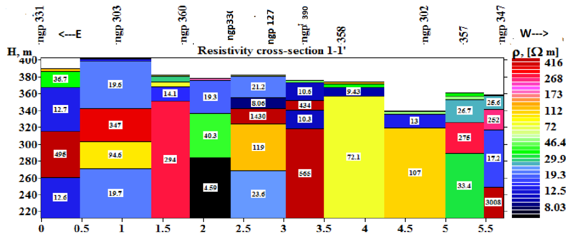
Fig.8: Resistivity Cross Sections along Section 1-1' based on VES Results, Chandrabhaga Watershed (WGKKC-2)
