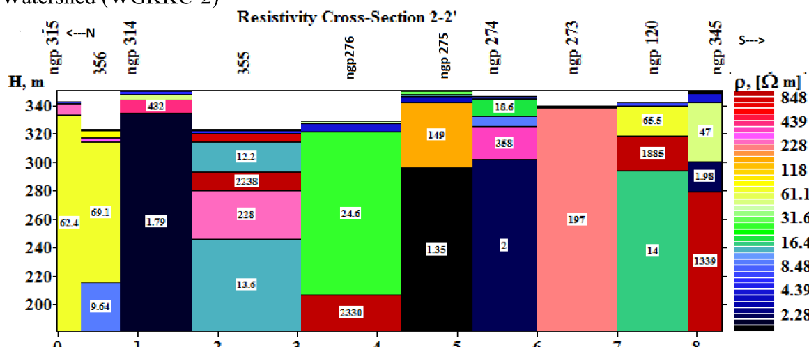
Fig.9: Resistivity Cross Sections along Section 2-2', based on VES Results, Chandrabhaga Watershed (WGKKC-2)
