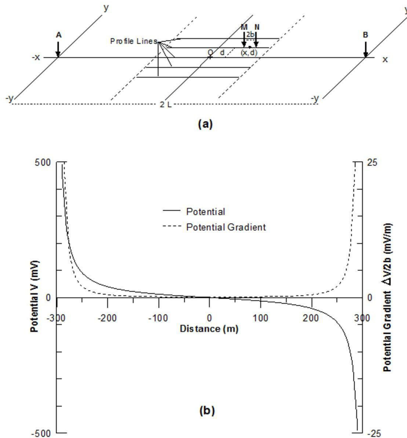
Figure 2: (a) General lay-out of gradient measurement of the potential field where AB = current electrodes and MN = potential electrodes, and (b) distribution of potential and gradient of potential along the line at the surface of homogeneous earth for d=0 , I=1000 mA, and \rho = 31.4 ohm-m
