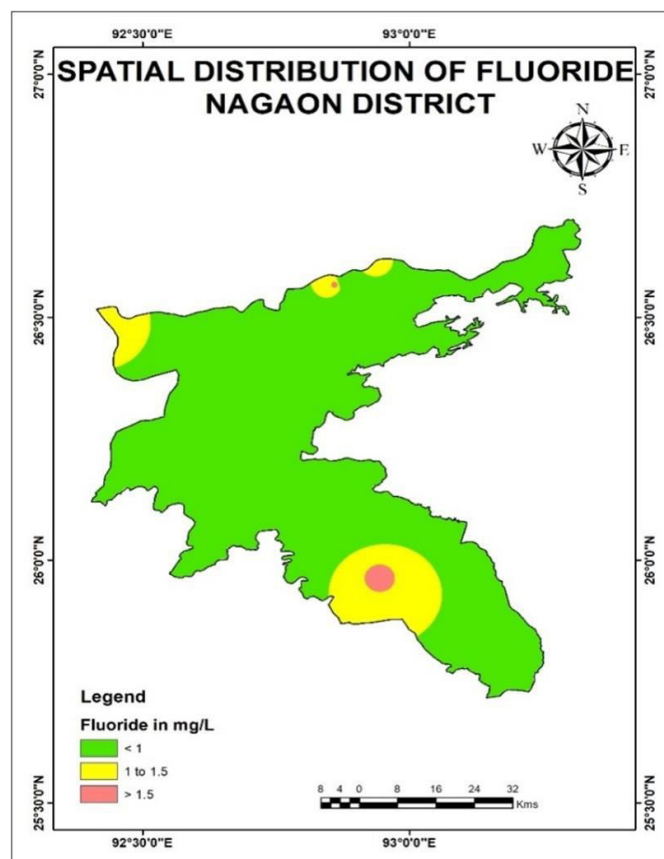
Fig. 3-Spatial distribution of Fluoride in Nagaon district
