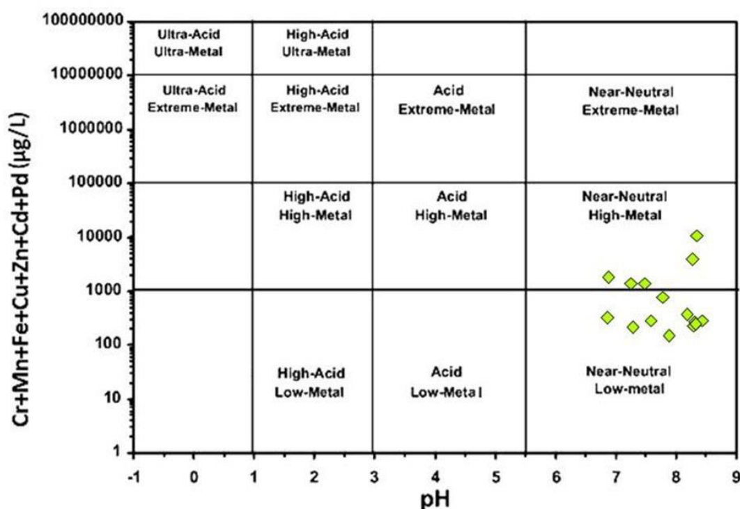
Fig. 8 Plot of metal load and pH of water samples.
