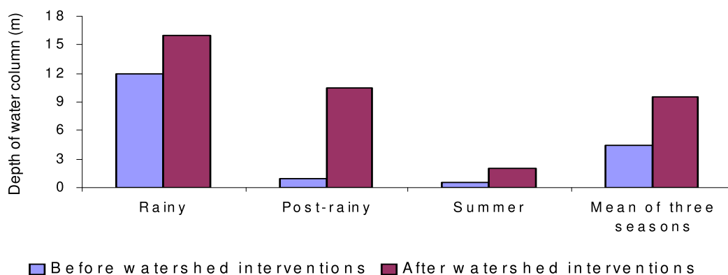
Figure 6. Effect of watershed intervention on water column in open wells, Bundi watershed, Rajasthan (Source: Pathak et al. 2007).
