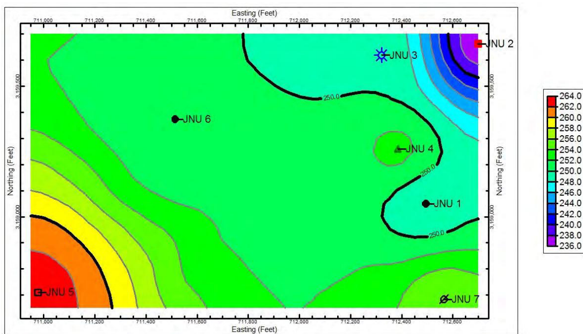
Figure.6.Elevation contours of the sites within study area selected for drilling indicate that elevation naturally increases towards south-west region. Towards eastern and north-eastern parts of study area elevation decreases sharply.
