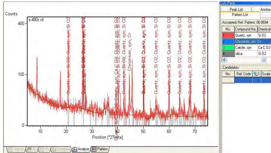
Figure.10.Mineral composition in JNU at 82 m bgl
