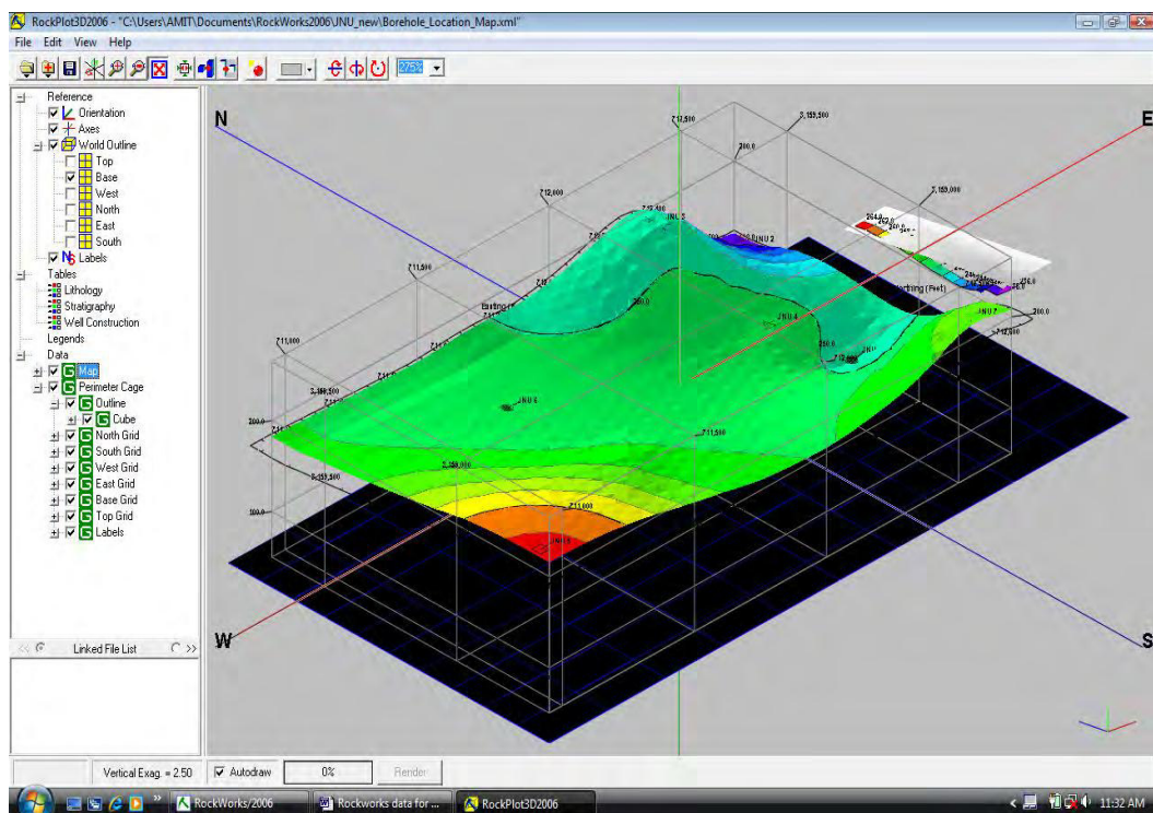
Figure.5.Rockware modelling of elevation contour in NCR area.
