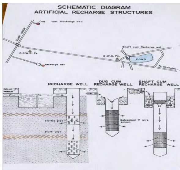
Fig-5. Schematic Diagramme of Artificial Recharge structure
