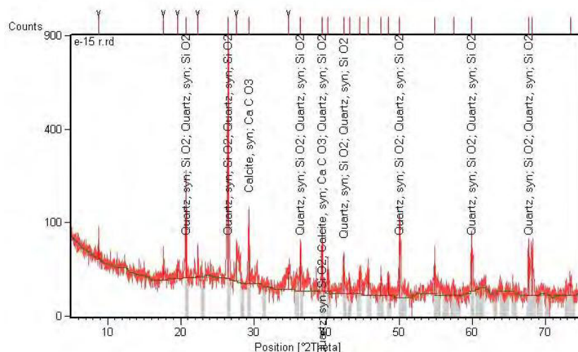
The presence of different mineral studied in thin section under the petrological microscope, ICPAES and X-Ray diffraction confirms the presence of zoned pegmatite in this area. Groundwater quantity and quality in this area is dependent on grade of metamorphism i.e. pegmatisation and its structural anomaly. Presence of Barium Feldspar forms a weak zone through which the fractures have been developed down to 4.57 to
