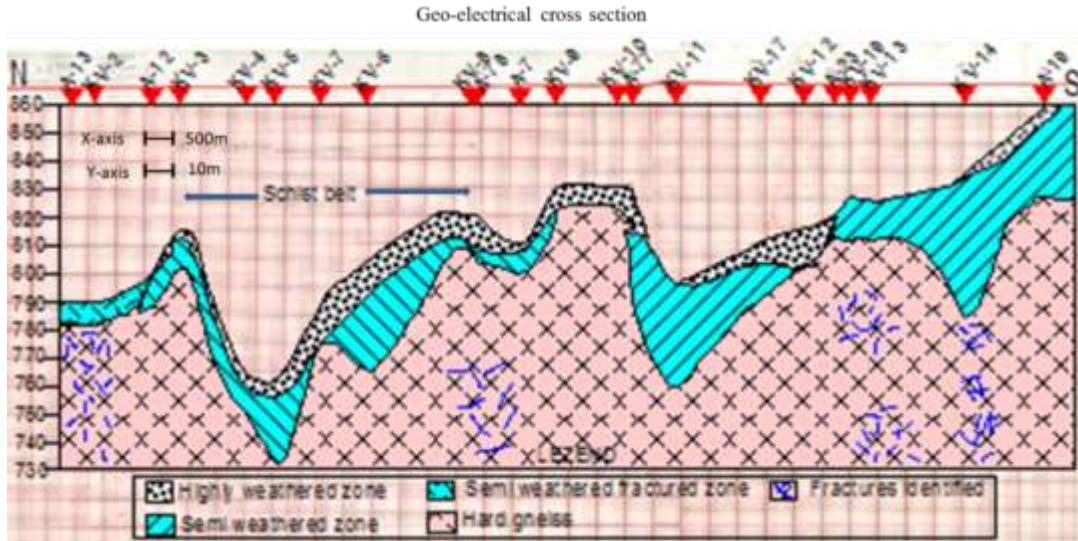
Fig. 3.27: Geo-electrical section along Huli-Tiptur road (Database NGRI & CGWB)
