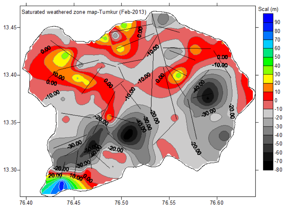
Fig. 3.34: Saturated zone thickness map (Data base NGRI & CGWB) Gradient Resistivity Profile (GRP)
