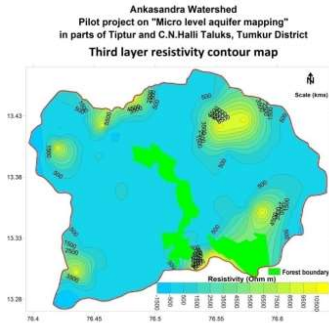
Fig. 3.24: Third layer resistivity map
