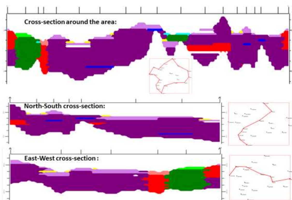
Fig. 5.14: Lithology cross-sections
