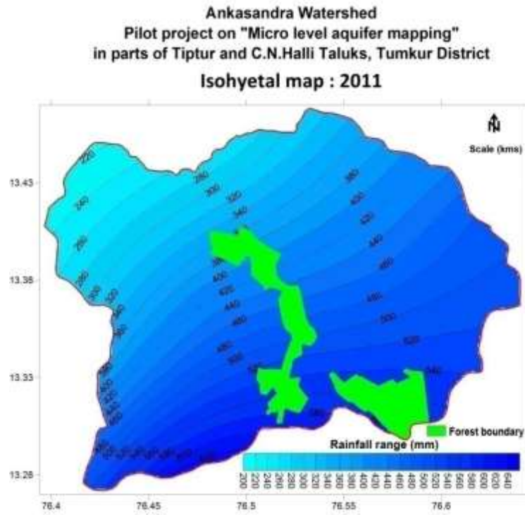
Fig. 3.2: Isohyets (2011)
