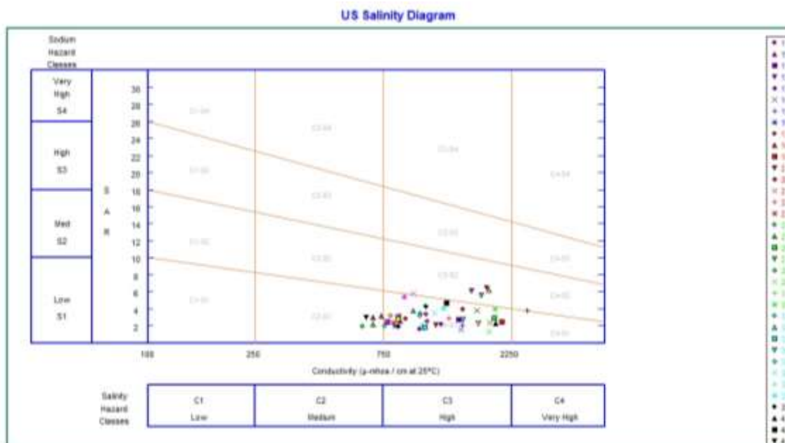
Fig. 3.70: Classification of irrigation water quality with respect to Salinity hazard and Sodium hazard (USSL diagram)
