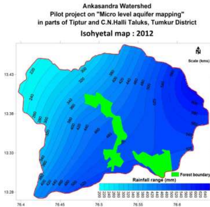
Fig. 3.3: Isohyets (2012)
