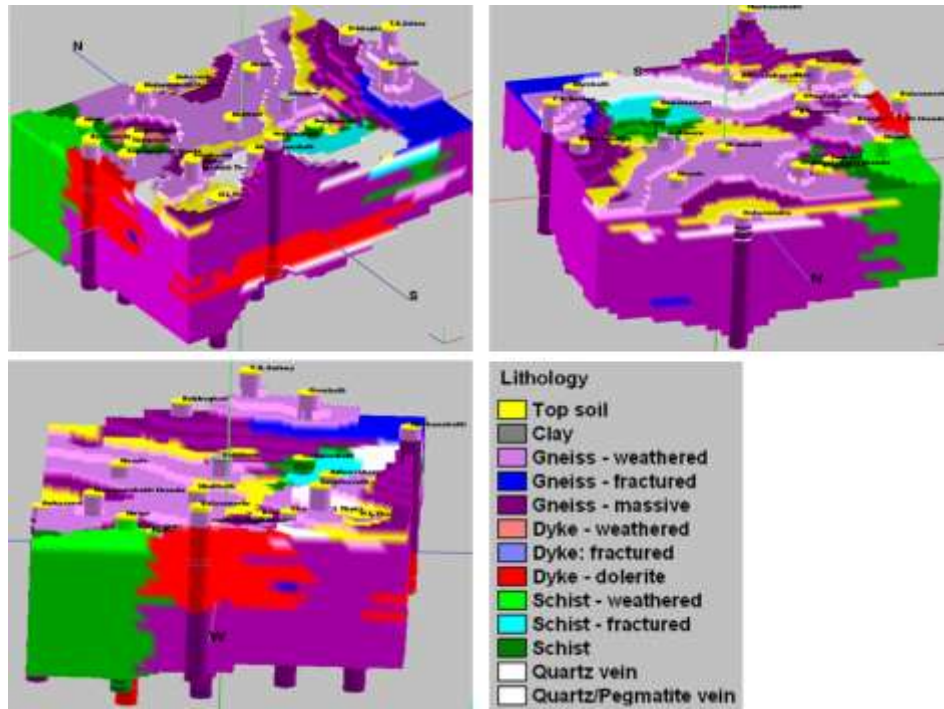
Fig. 5.11: 3D-lithology models
