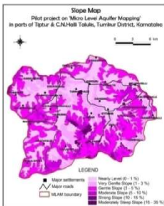
Fig. 3.12: Slope map
