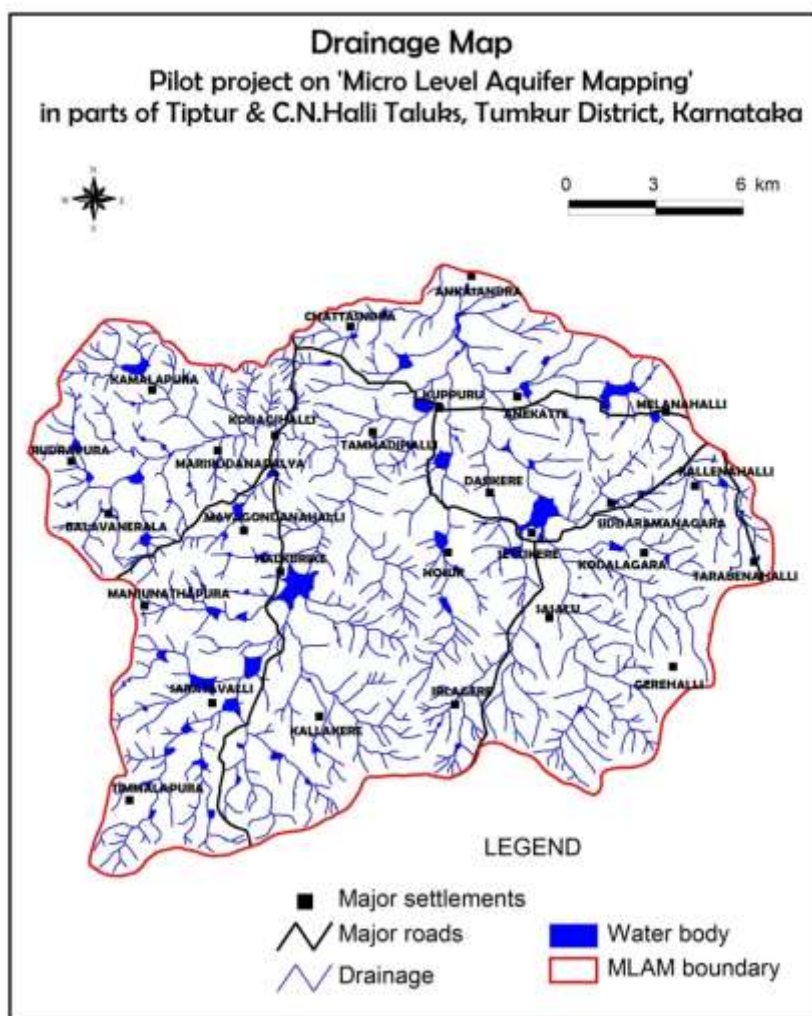
Fig. 3.9: Drainage map
