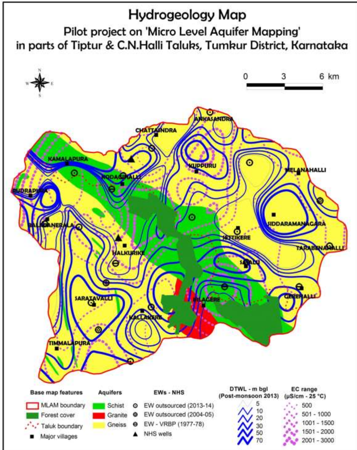
Fig. 3.45: Hydrogeology map
