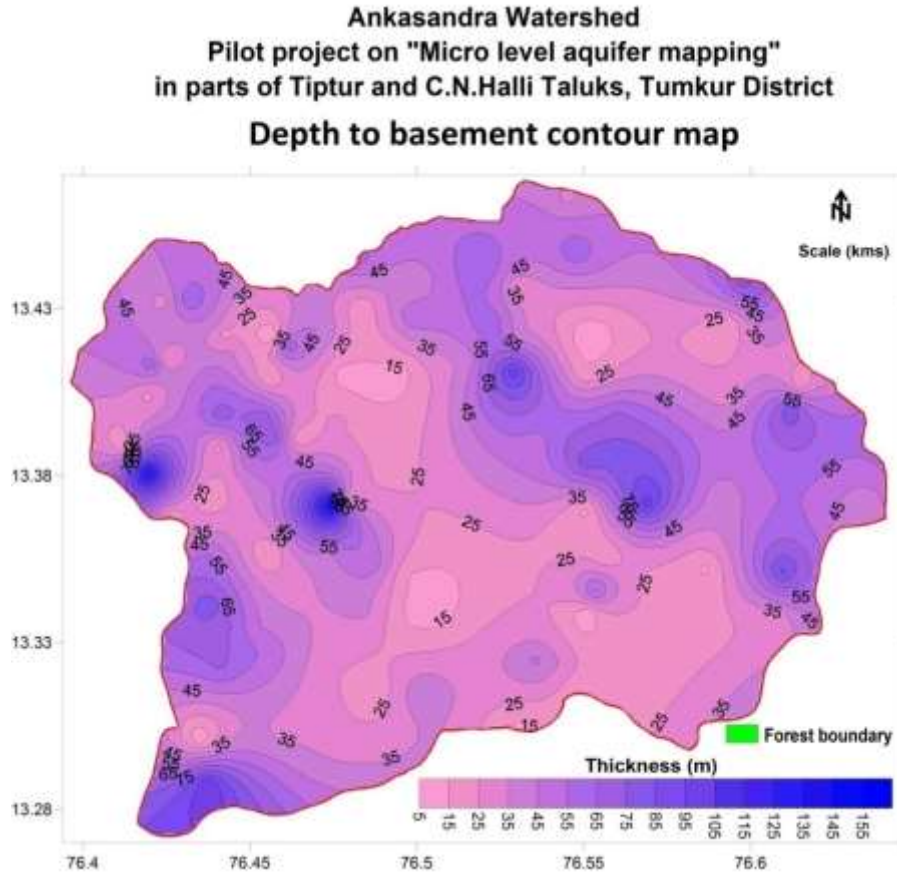
Fig. 3.17: Depth to basement contour map
