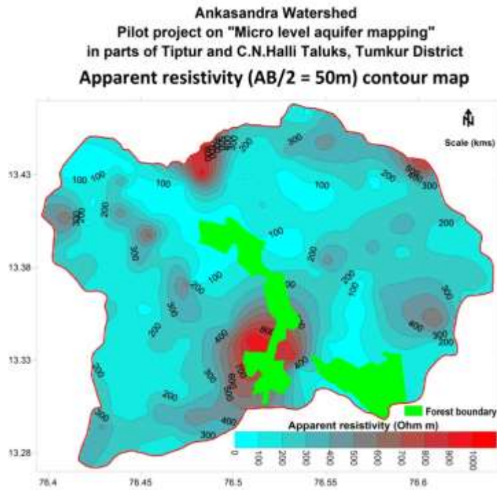
Fig. 3.19: Apparent Resistivity at AB/2=50 m
