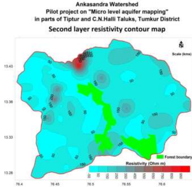
Fig. 3.23: Second layer resistivity map
