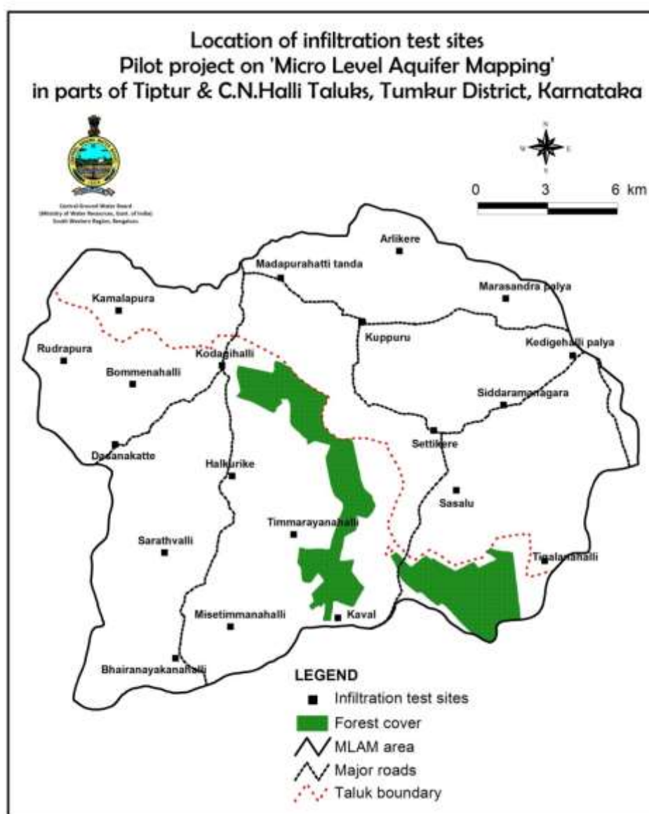
Fig. 3.6: Location of infiltration test sites
