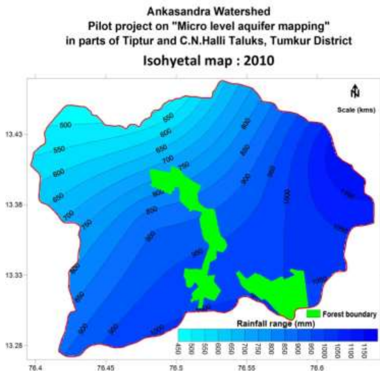
Fig. 3.1: Isohyets (2010)
