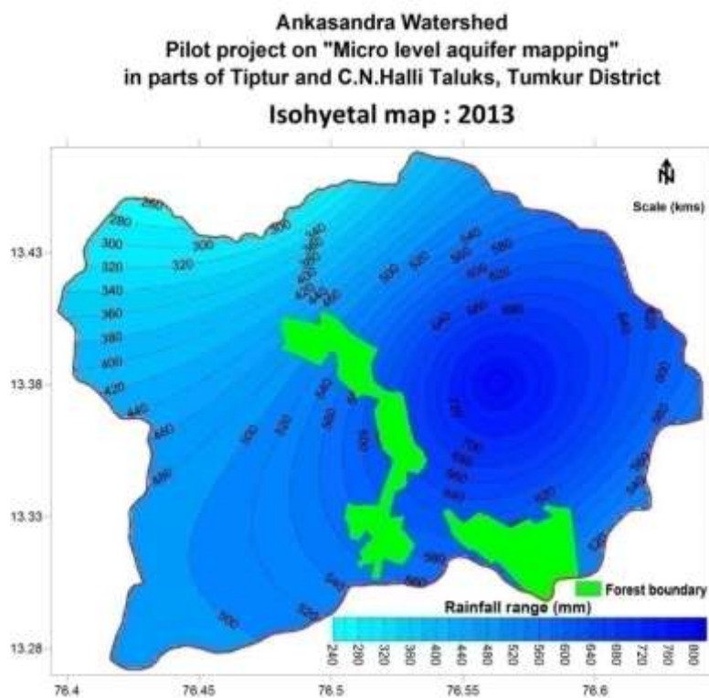
Fig. 3.4: Isohyets (2013)
