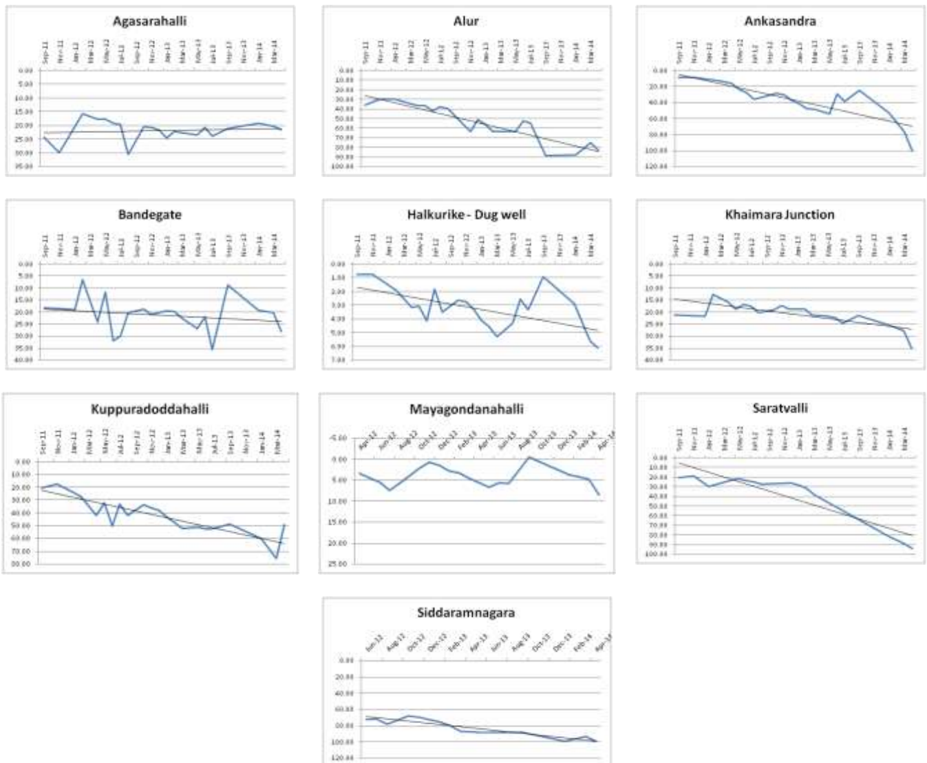
Fig. 3.63: Hydrographs of selected stations
