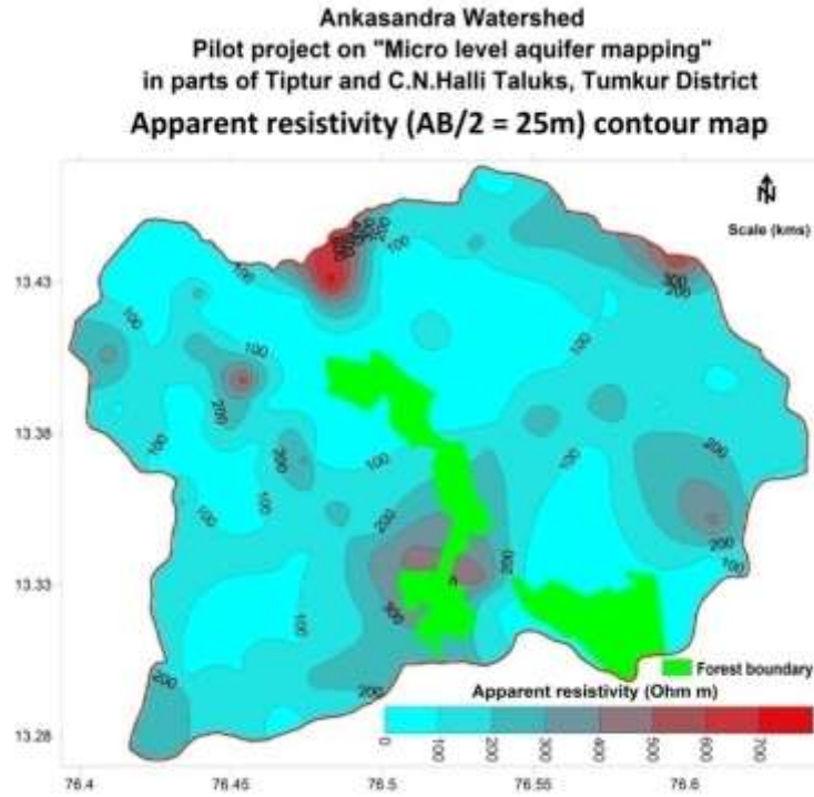
Fig. 3.18: Apparent Resistivity at AB/2=25 m
