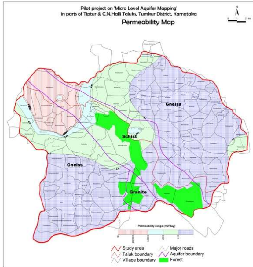
Fig. 5.19: Permeability map
