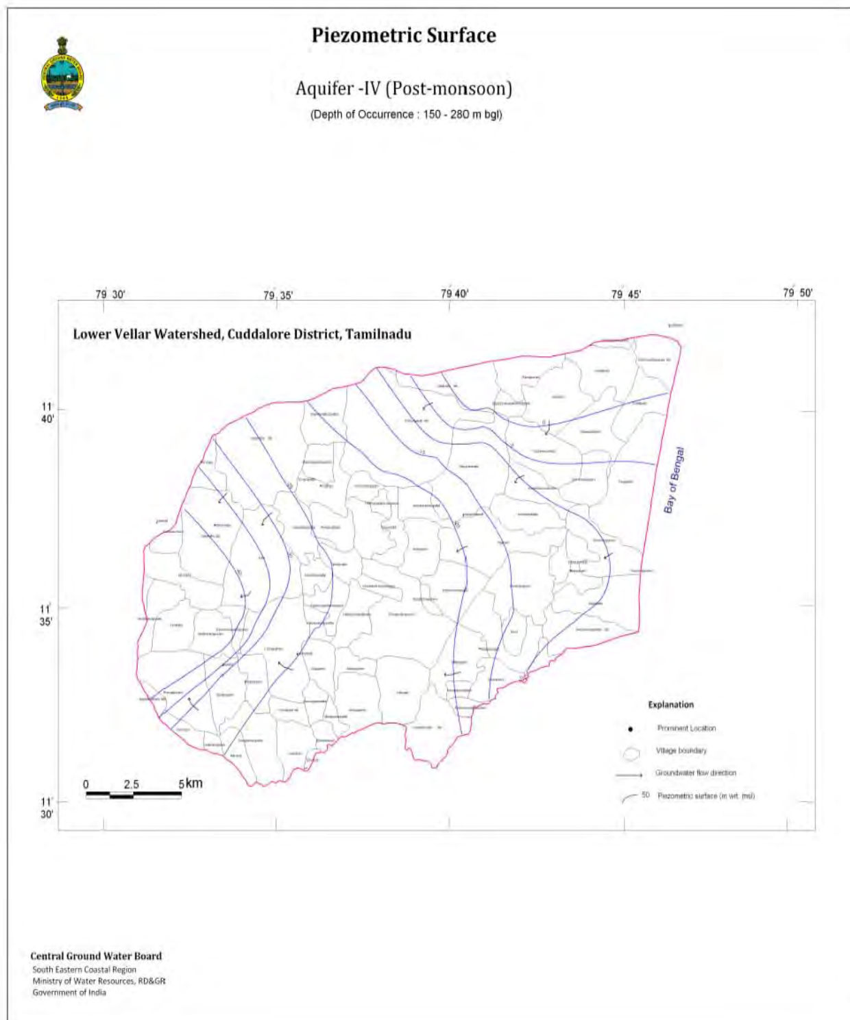
Figure: 5.29 Piezometric Surface-Post monsoon-Aquifer-IV
