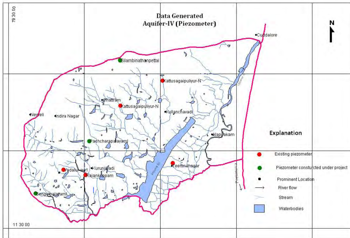
Figure 3.8 Data generated Aquifer-IV (Groundwater quality monitoring station)
