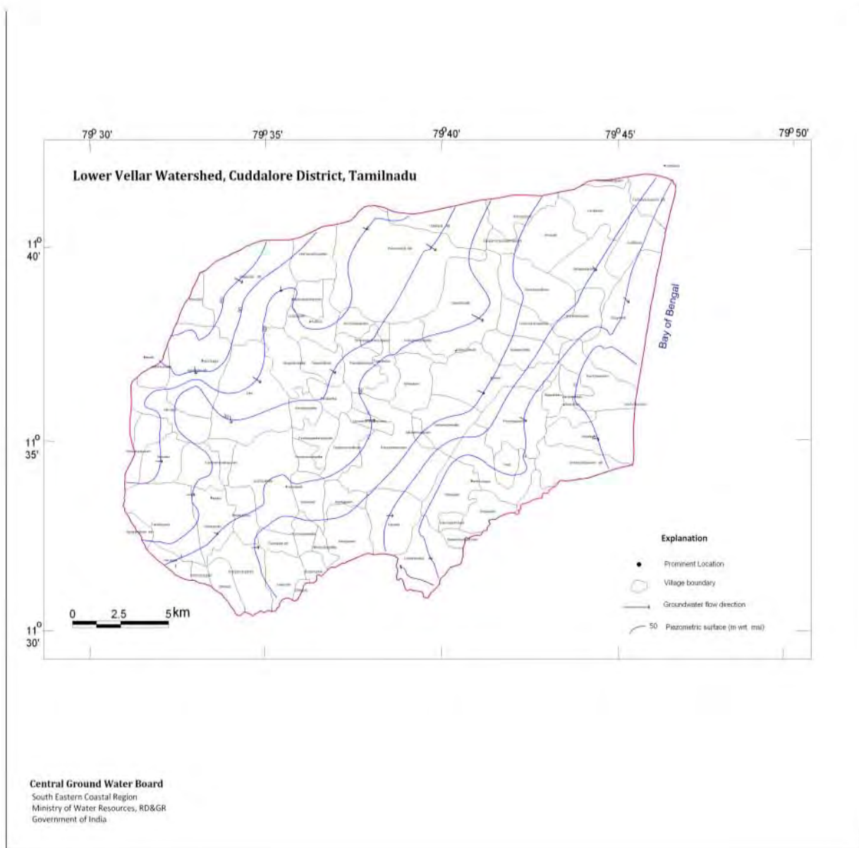
Figure: 5.22 Depth to Water table Elevation-Pre monsoon - Aquifer-I
