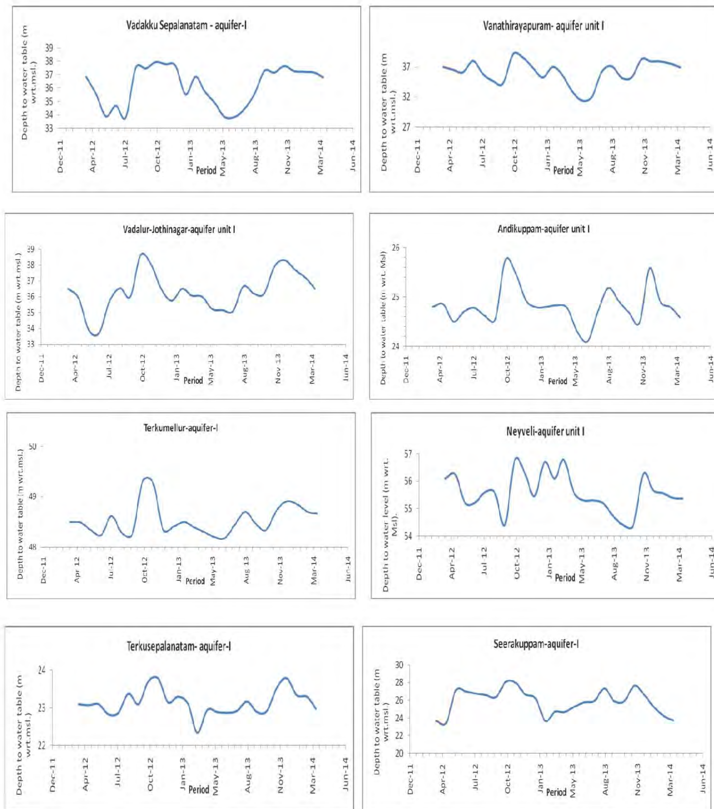
Figure 3.40 Hydrographs-Neyveli area
