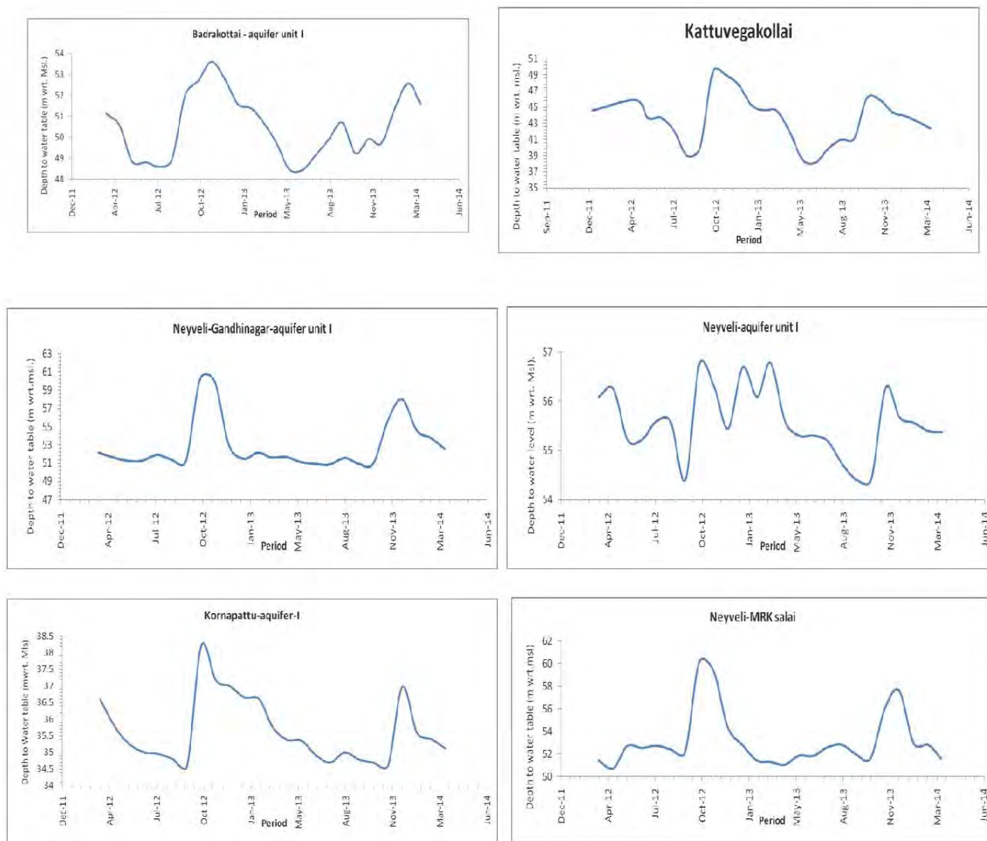
Figure 3.38 Hydrographs in the Recharge Zone
