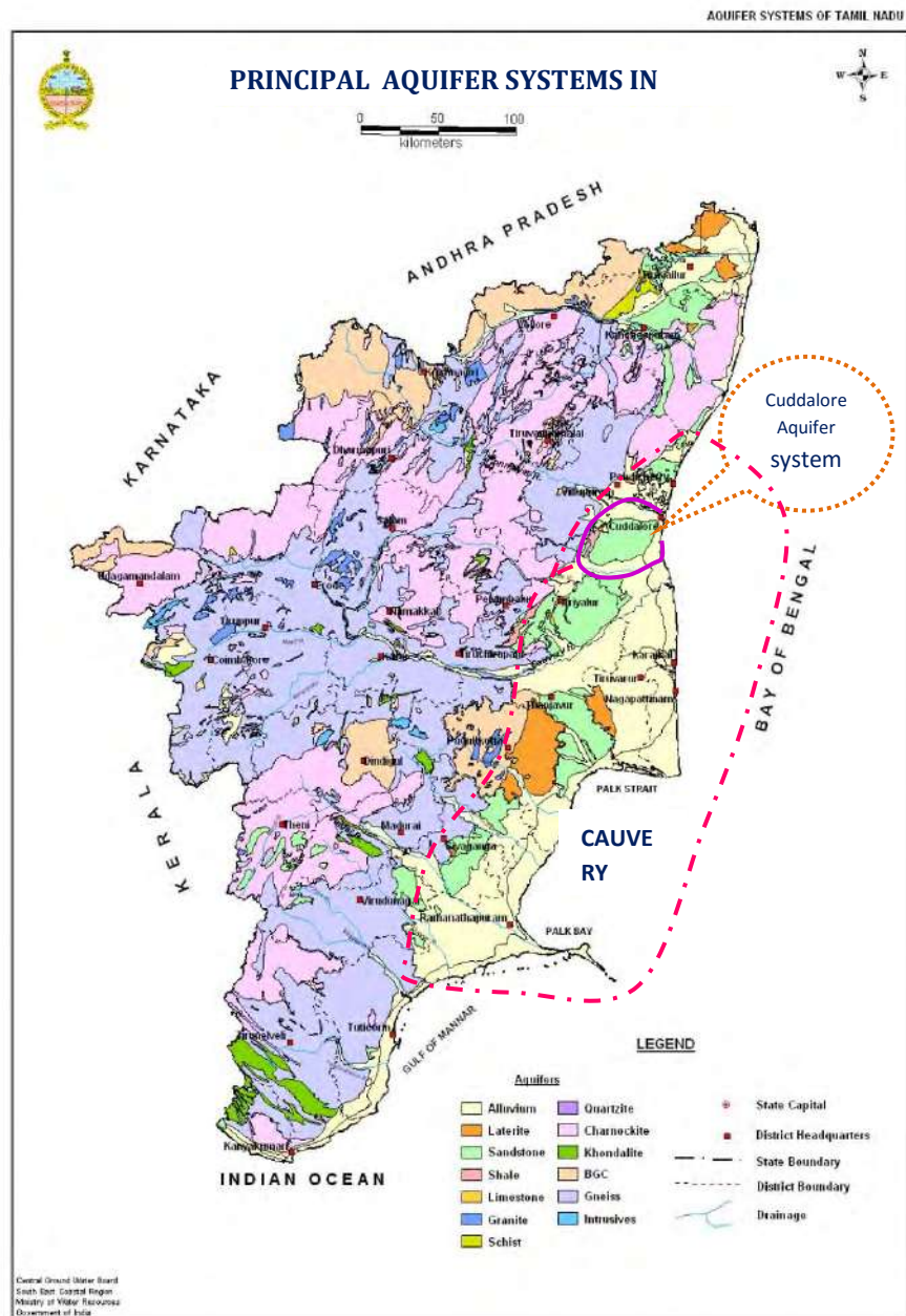
Figure6.2Map showing the Cauvery Basin and the location of Cuddalore aquifer system.
