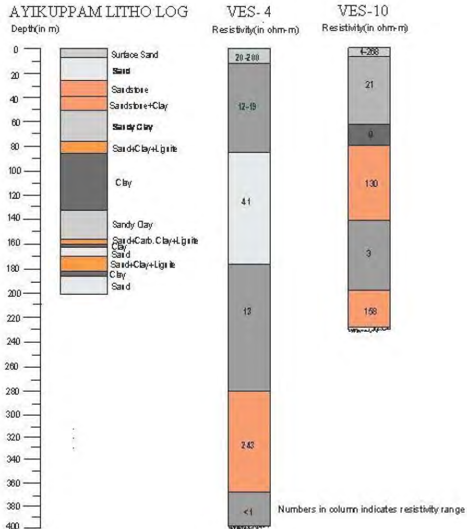
Fig. 3.20 Litholog of Aiykuppam exploratory well (CGWB) & interpreted layer Parameters of VES-2 and VES-10
