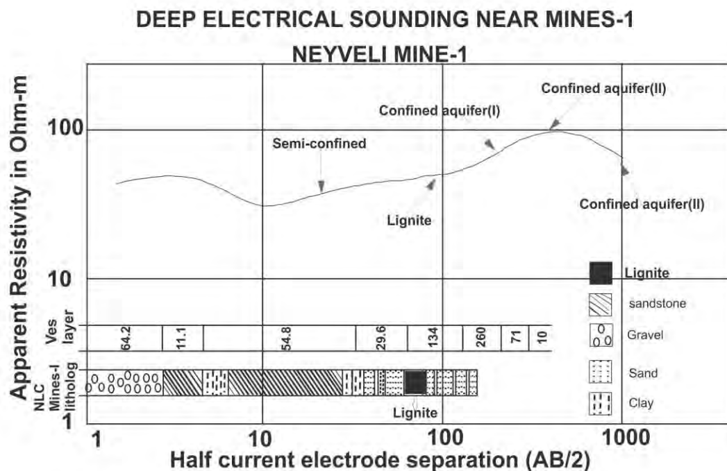
Fig. 3.18 VES-24curve near Neyveli mines-I
