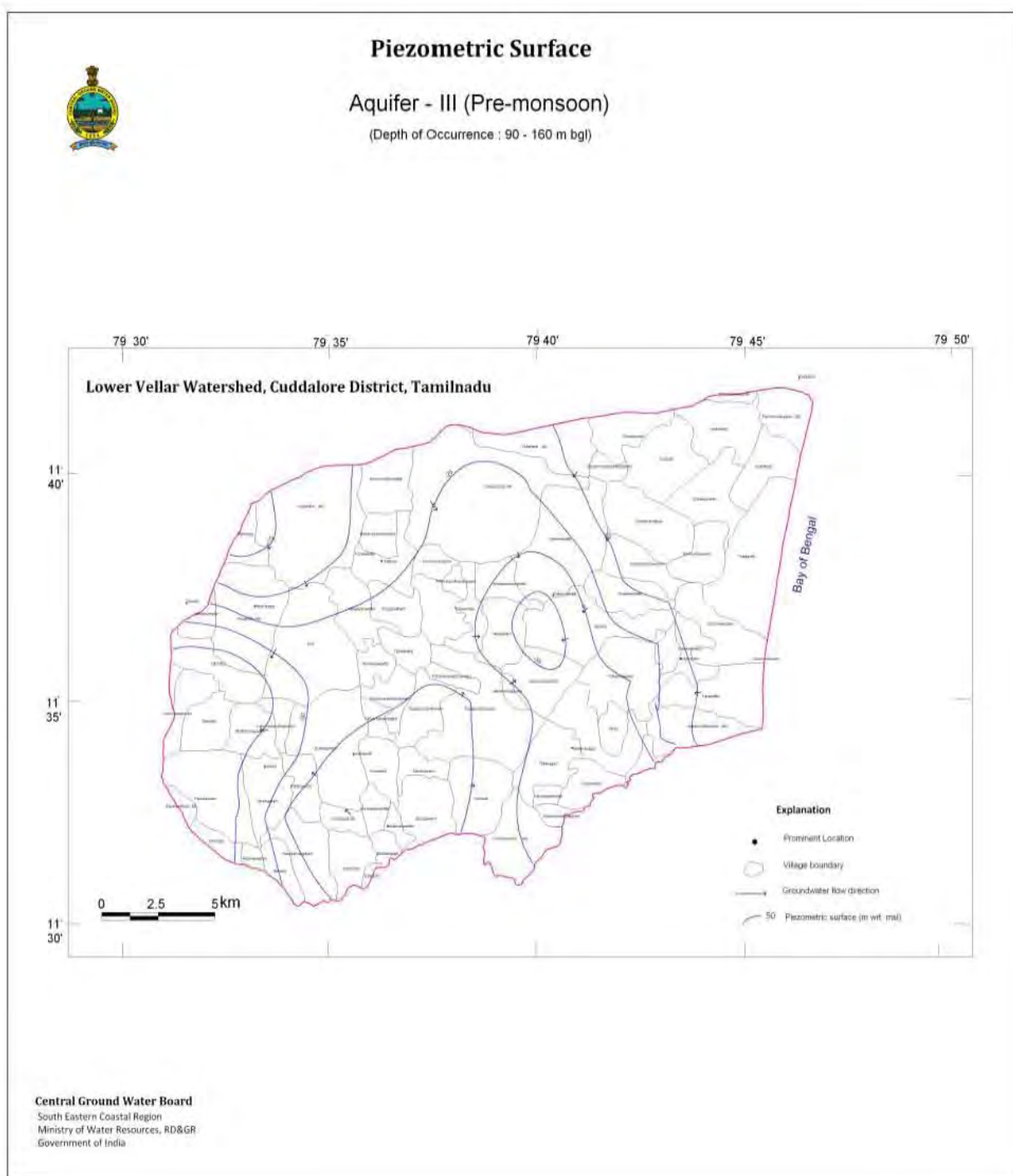
Figure: 5.26 Piezometric surface-Pre monsoon- Aquifer-III
