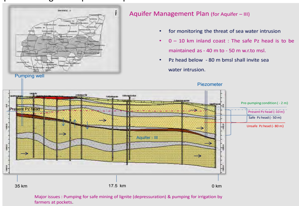
Figure 7.1: Aquifer management plan for Aquifer– III
