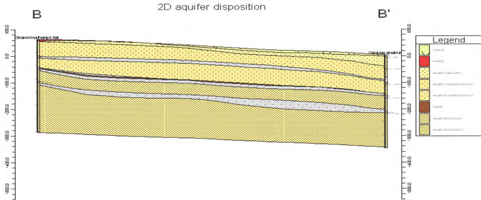
Figure: 5.2 2D Aquifer Disposition along Silambinathanpettai to Srinivasanallur
