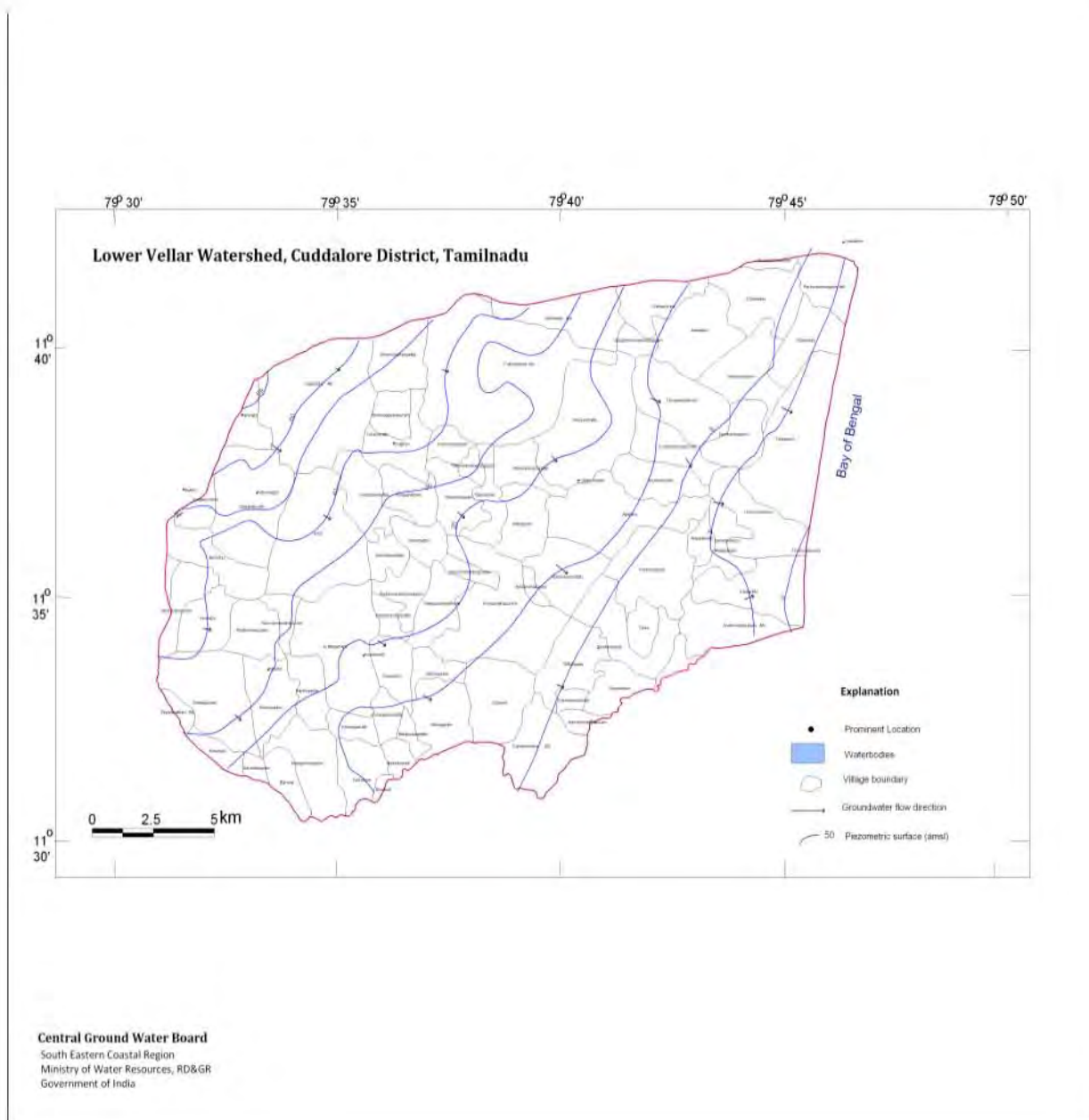
Figure: 5.23 Depth to Water level Elevation – Post monsoon-Aquifer-I
