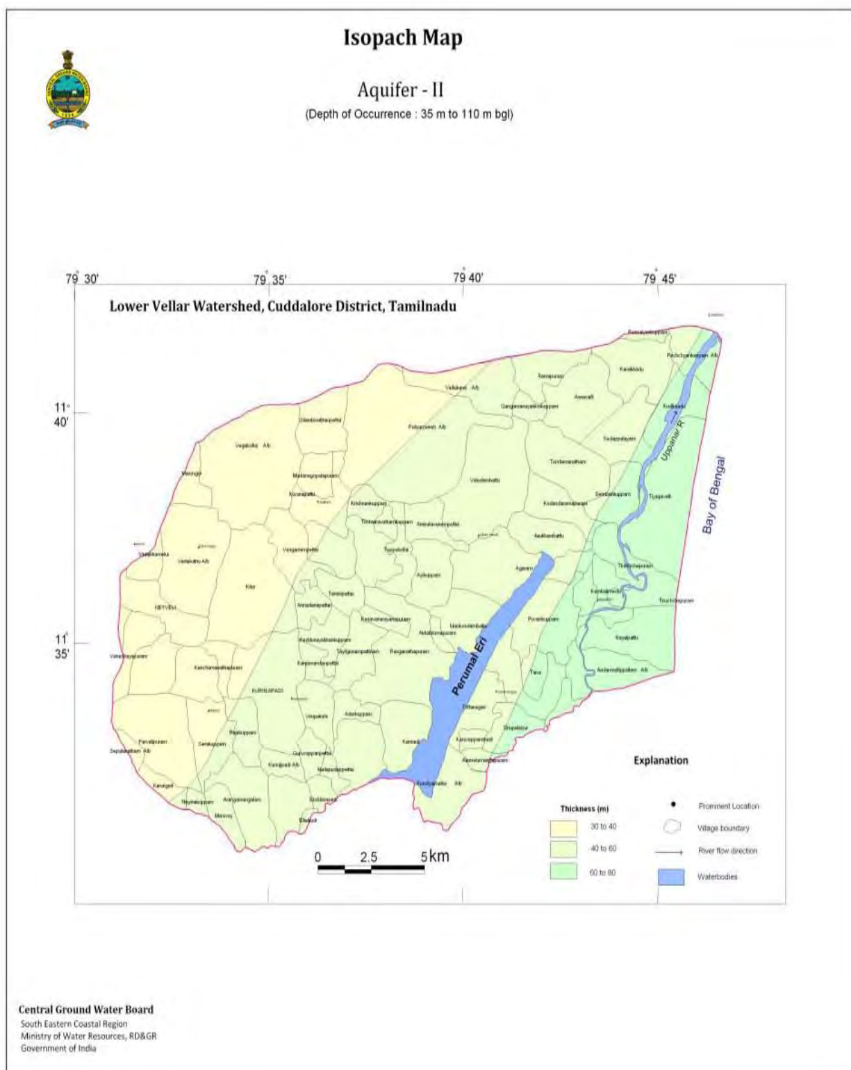
Figure: 5.16 Isopach Map-Aquifer-II
