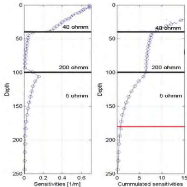
Figure 3.29. Sensitivities calculated for a rediscretized version of the model indicated by the black lines; resistivities of layers are written on the plot. The left plot is the
