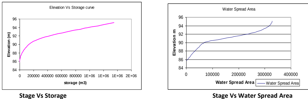
Figure 3 Stage vs Storage and Stage vs Water spread area of Annupankulam Tank
