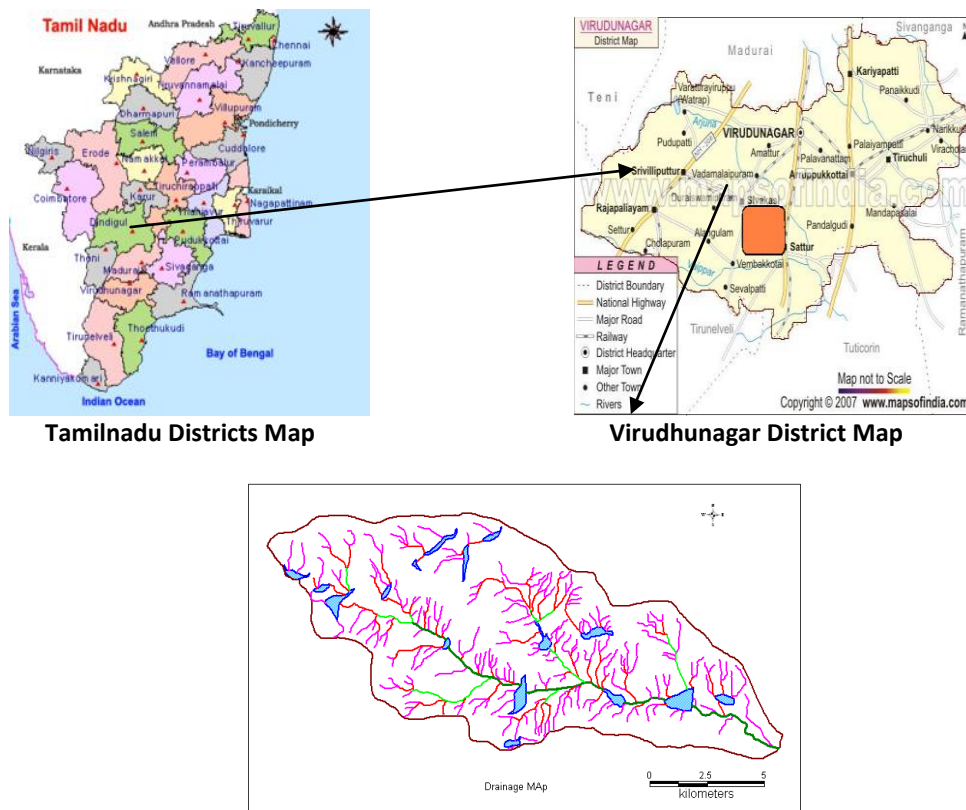
Sindapalli Uppodai Sub basin Drainage Map
