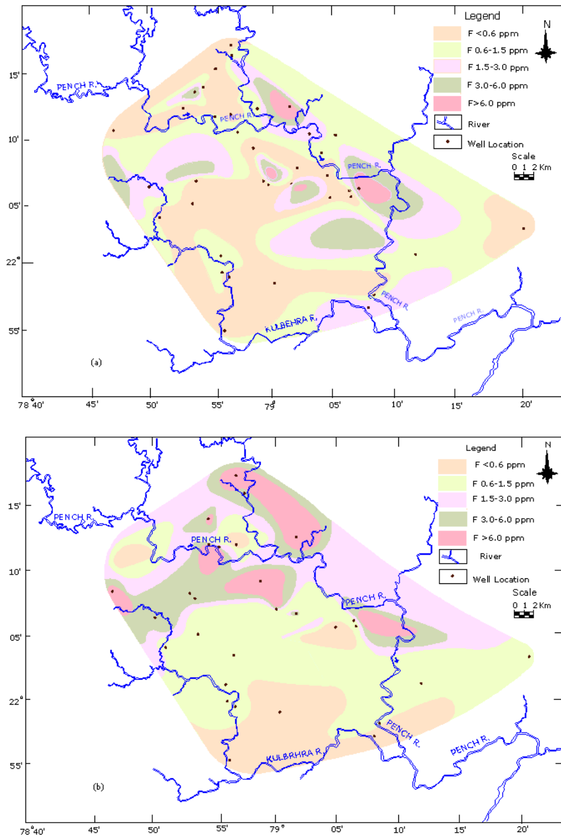
Fig.4. Spatial distribution of fluoride in ground water during (a) pre-monsoon period and (b) Post-monsoon period
