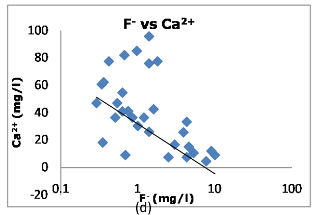
Fig.5. Relationship of fluoride and Ca 2+ : a & b in granitoids in the pre- and post-monsoon period, c & d in basalts in both the period
