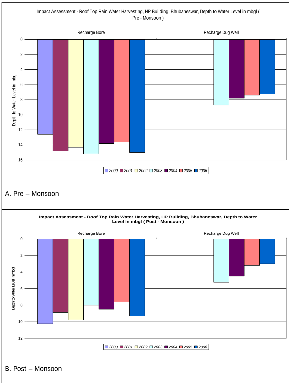
Figure 59 (A-B) : Impact Assessment – Roof Top Rain Water Harvesting, HP Administrative Building, Bhubaneswar
