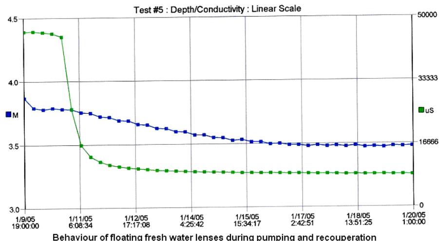
Figure – 53. Behaviour of floating fresh water lenses during pumping & recouperation
