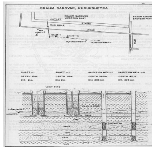
Figure 65: Artificial Recharge structure at Braham Sarovar, Kurukshetra city
