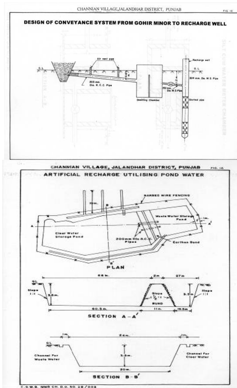
Figure 61: Artificial Recaharge Structure at Channian Nakodar Block, District Jalandhar
