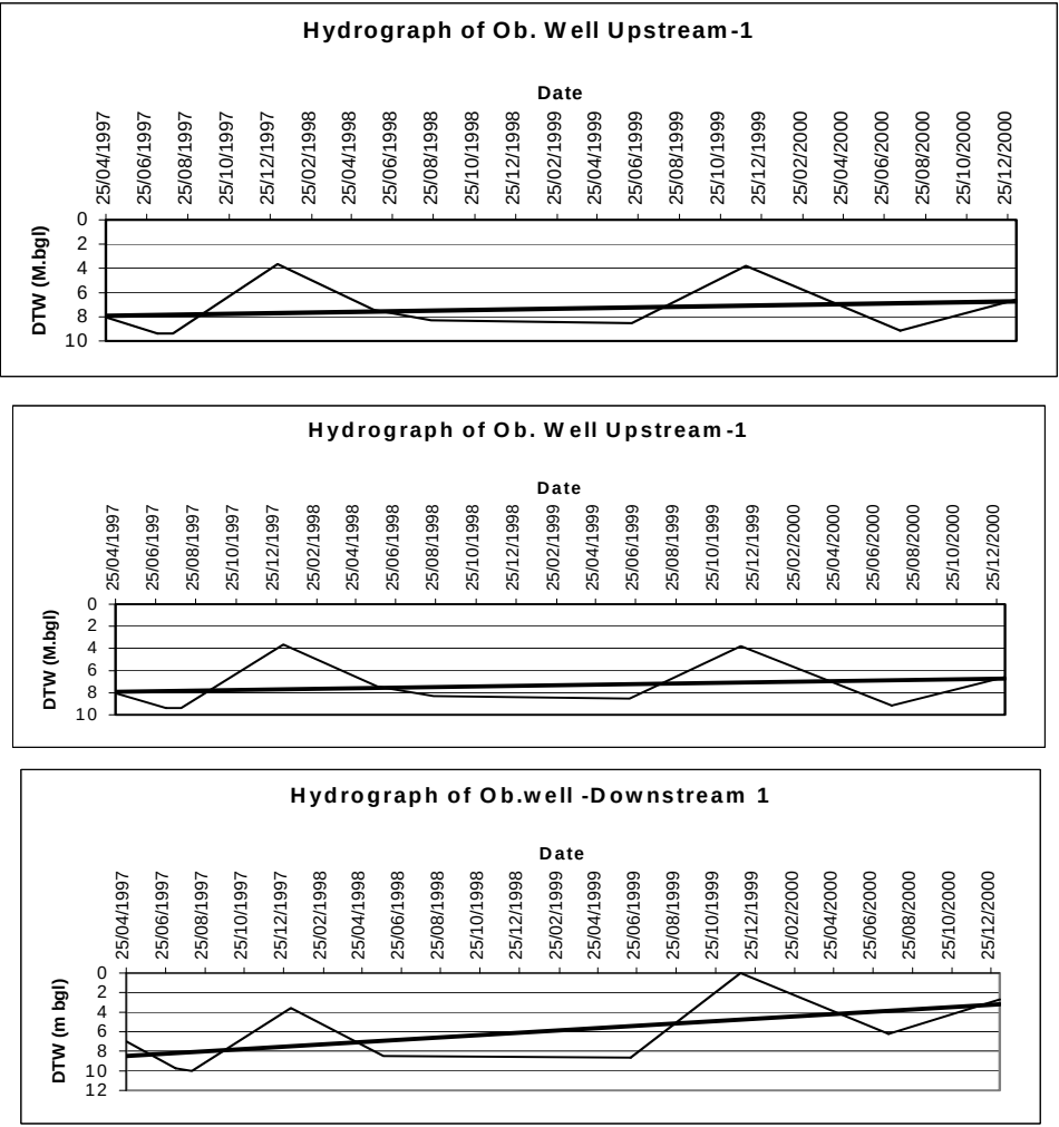
Figure 66: Hydrograph at Madam, Dharmapuri District
