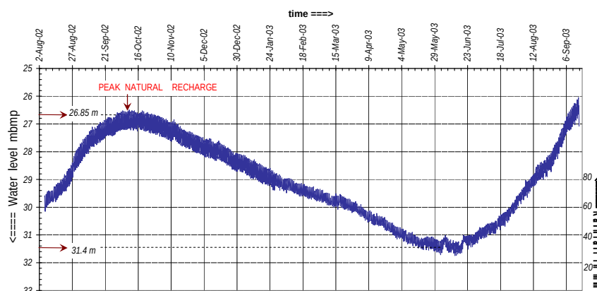
Figure 43 : Composite Hydrograph of Deeper Aquifer, Raj Bhawan Premises, Bhubaneswar
