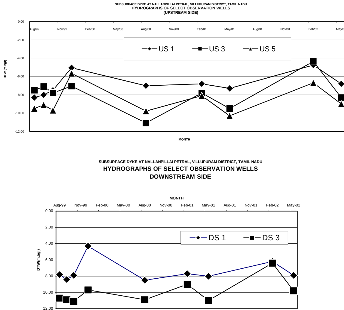
Figure 70: Hydrographs of OW on Upstream & downstream of dyke
