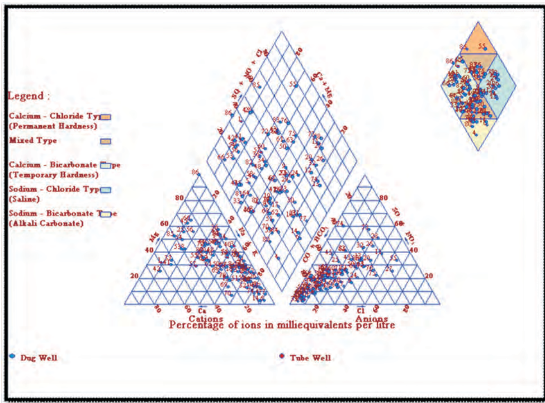
Fig 6.9, PIPER DIAGRAM -2007
