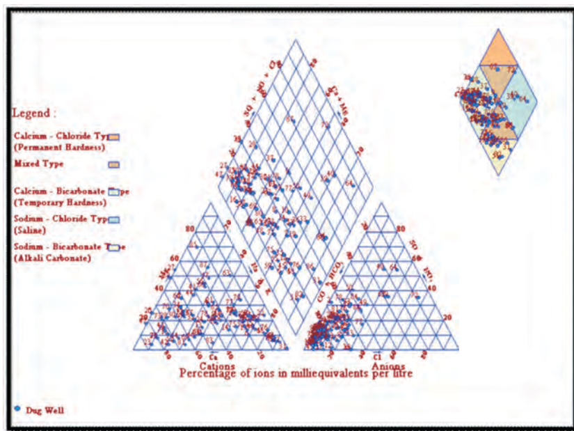
Fig 6.8, PIPER DIAGRAM -1978
