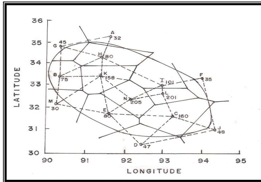
Fig. 4.4 Theissen Polygons
