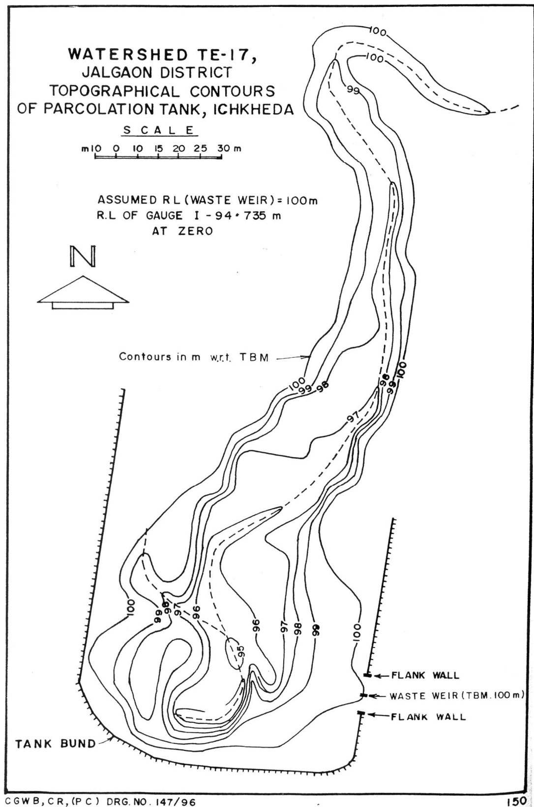
Fig. 8.1 Topographic Contours of Percolation Tank at Ichkheda.
