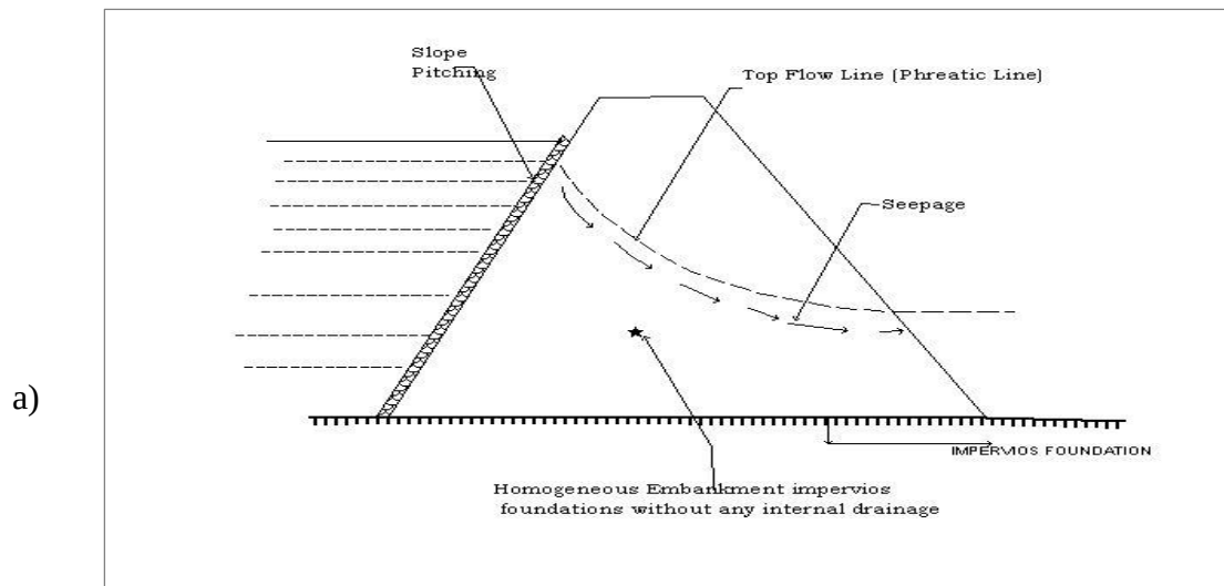
Homogeneous Type
