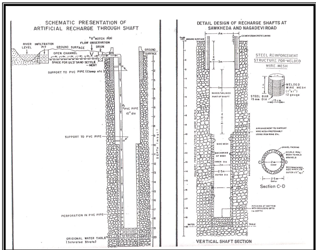
Fig.6.15 Schematics of Recharge Shafts
