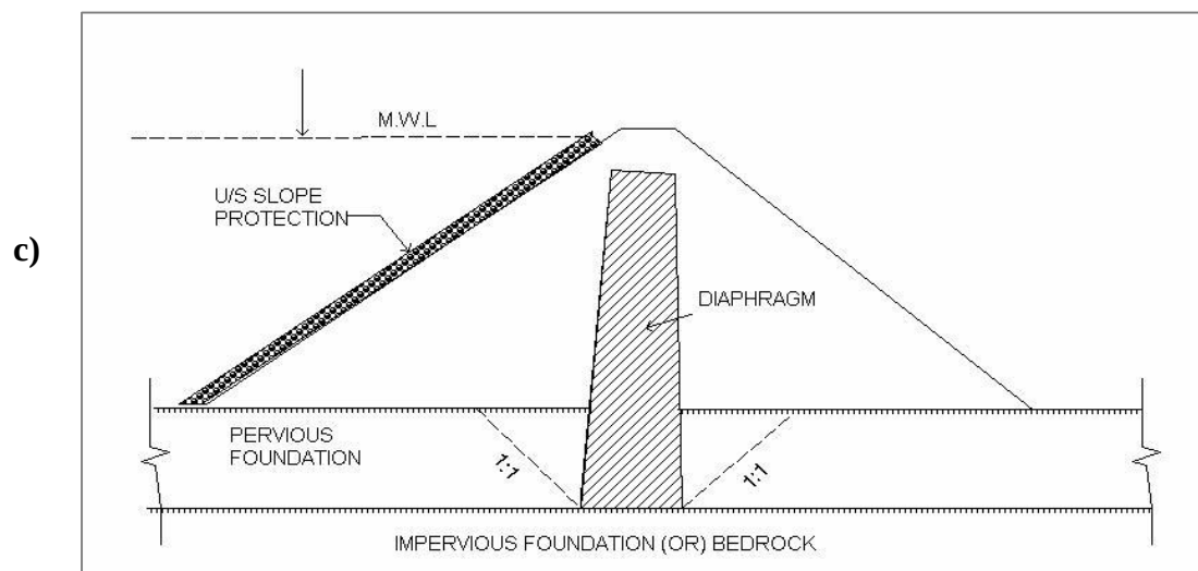
Diaphragm Type
