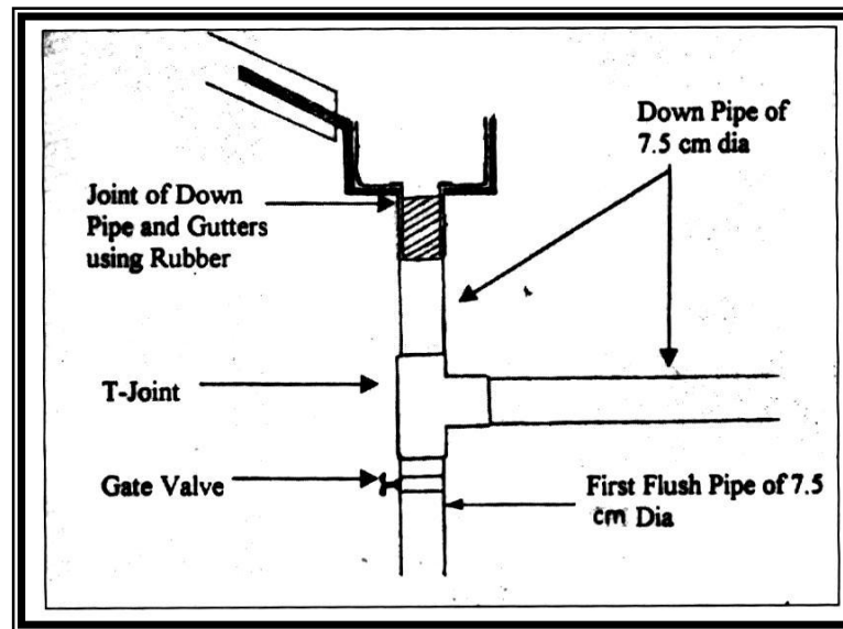
Fig. 7.4 Down Pipe
