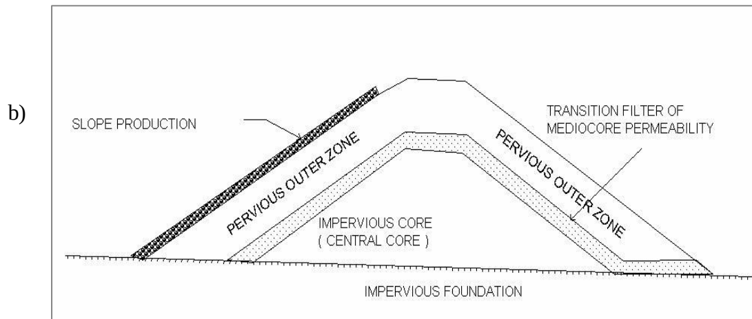
Zoned Type
