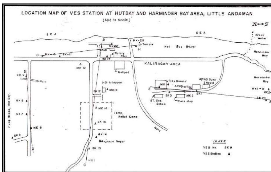
Figure-5.1.2.2: Location Map of VES at Hut Bay and Harminder Bay in Little Andaman Island Geoelectric cross-section along E - F:
