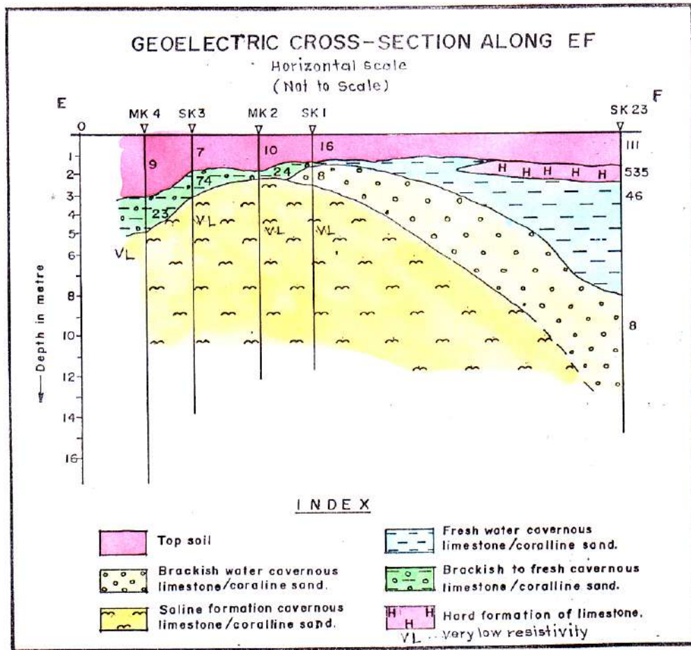
Figure-5.1.2.3: Geoelectric cross-section along E-F
