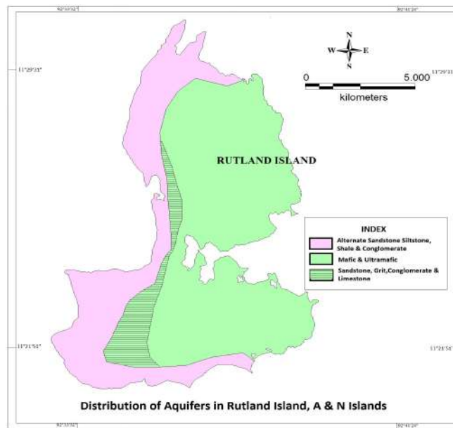
Figure 14.2.1: Distribution of Aquifers in Rutland Island
