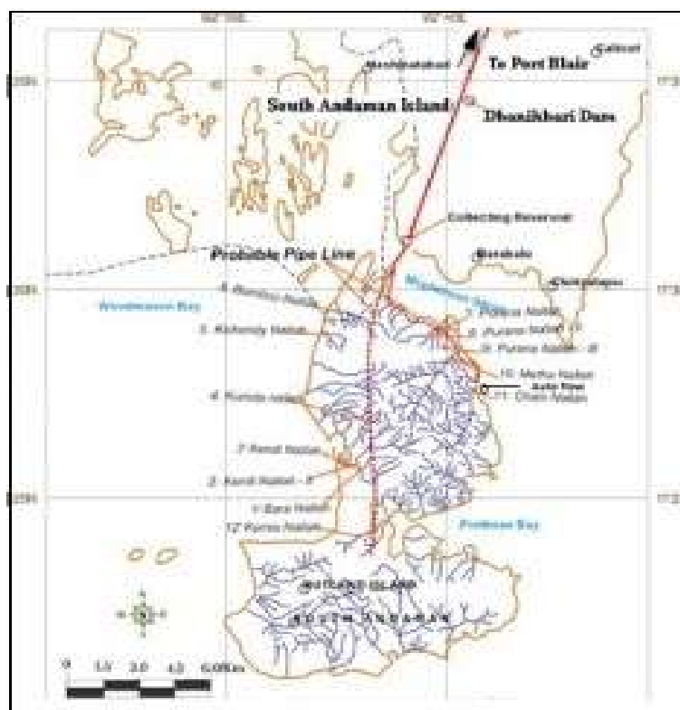
Figure-9.5.1 Plan of Interisland transfer of spring water from Rutland
