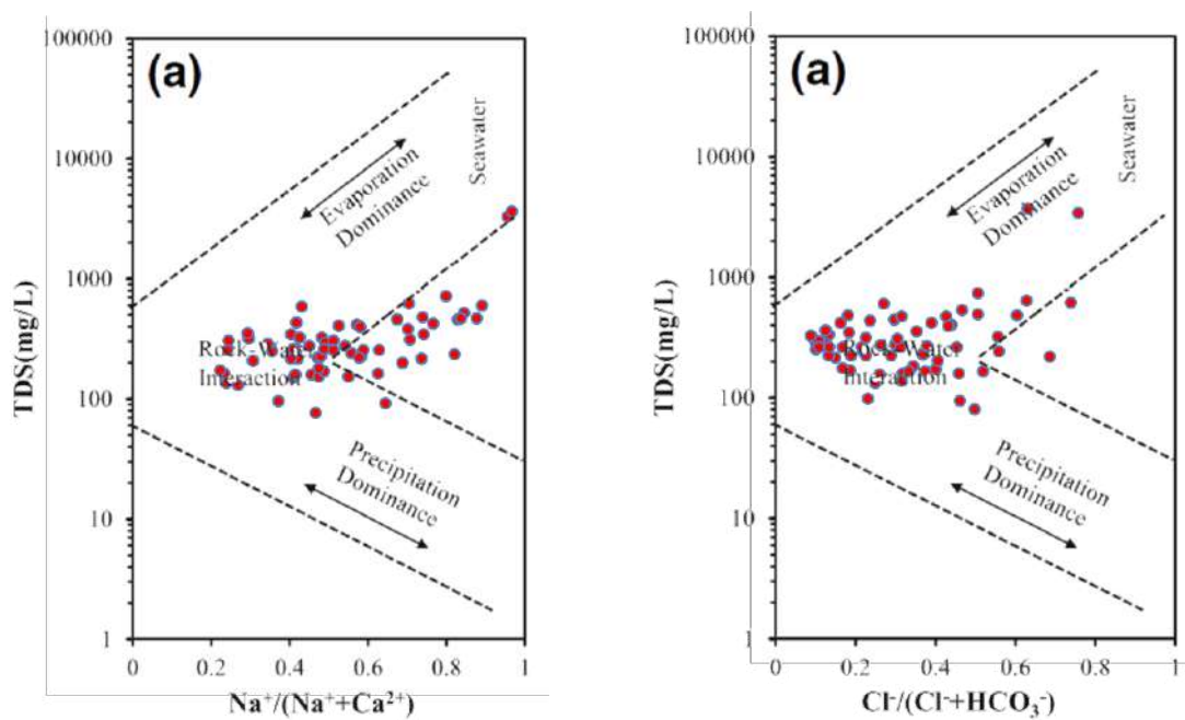
Figure 8.4.3 Gibbs Plot for South Andaman Island
