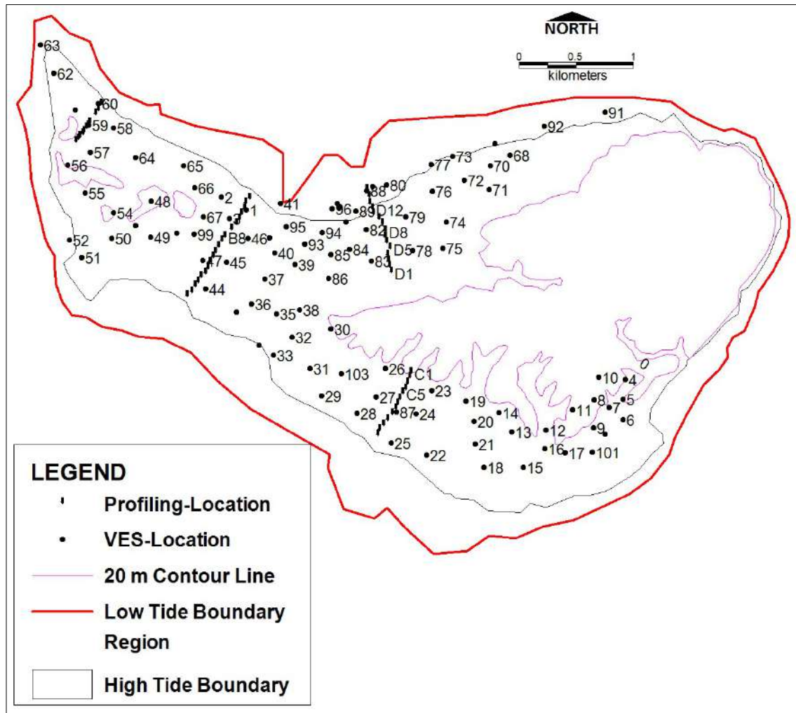
Figure-5.1.1.1 VES and Resistivity Mapping Locations of Neil Island
