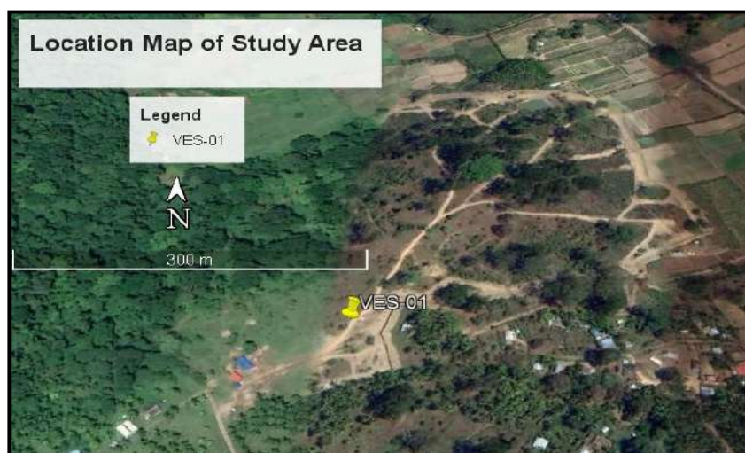
Figure-5.1.3.3: VES location in the premises of the Coast Guard, Namunaghar
