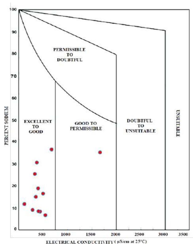
Figure 8.3.5 Wilcox diagram to assess the suitability of water for irrigation for Little Andaman
