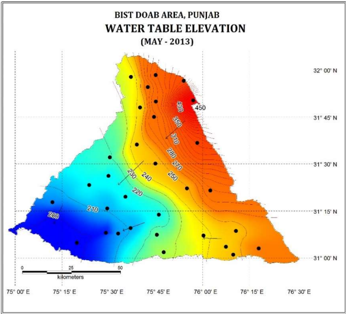
Fig.11-Water Table contour (Pre-monsoon 2013)
