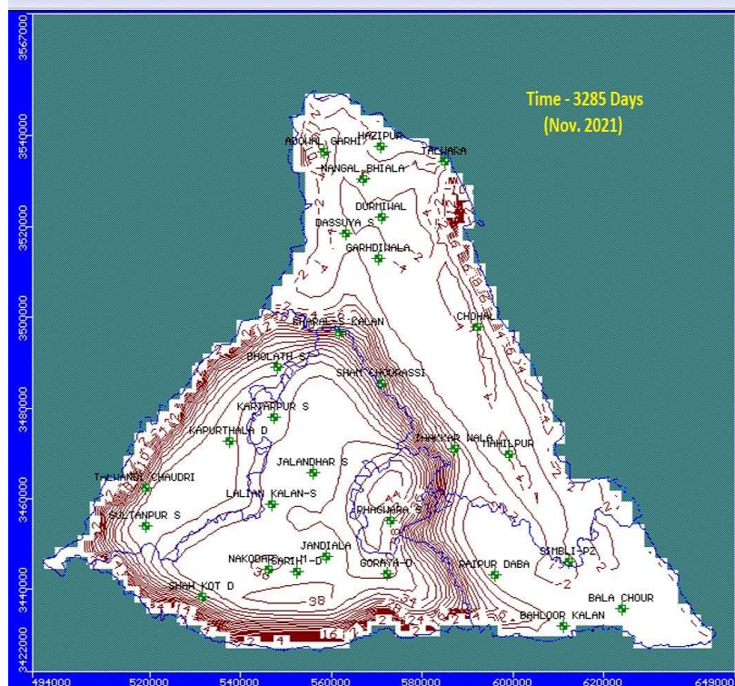
Fig.28-Drawdown Contours for Various Stress Period (Prediction-1)
