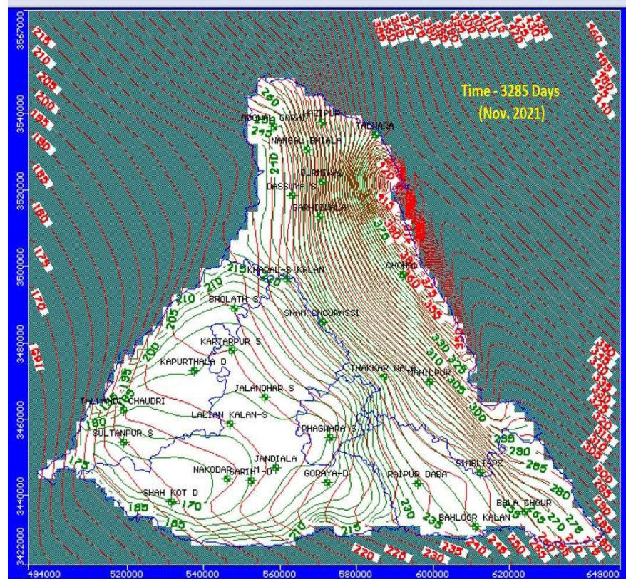
Fig.31-Head Contours for Various Stress Period (Prediction-2)
