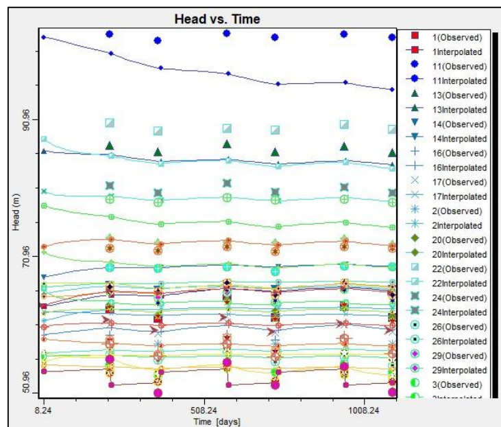
Fig 16: Hydrographs of Observation Points
