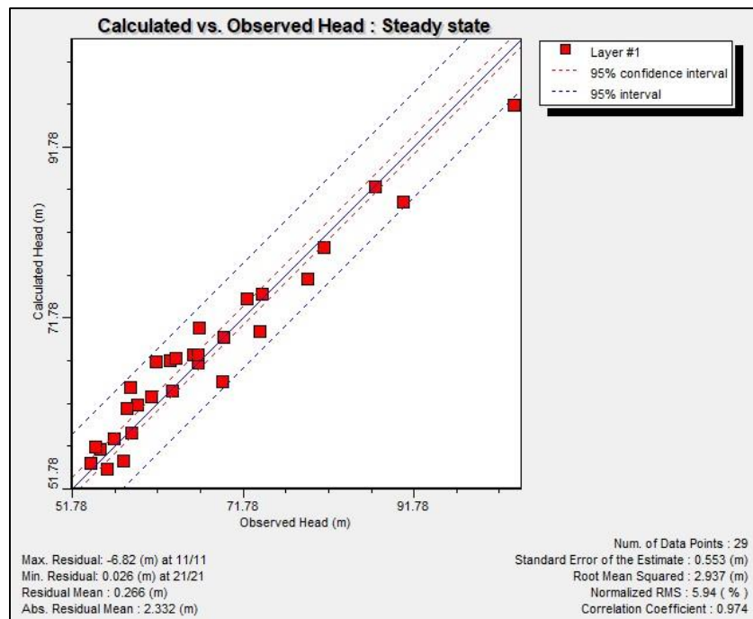
Fig 11: Head Scatter Graph for Steady State
