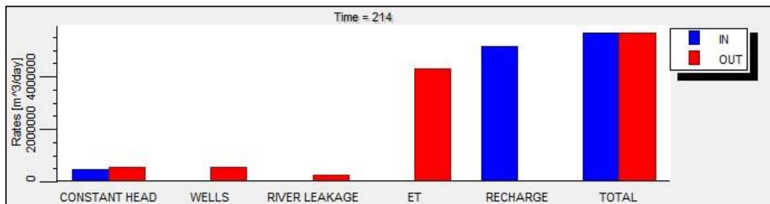
Fig 13: Zone budget for the Steady State
