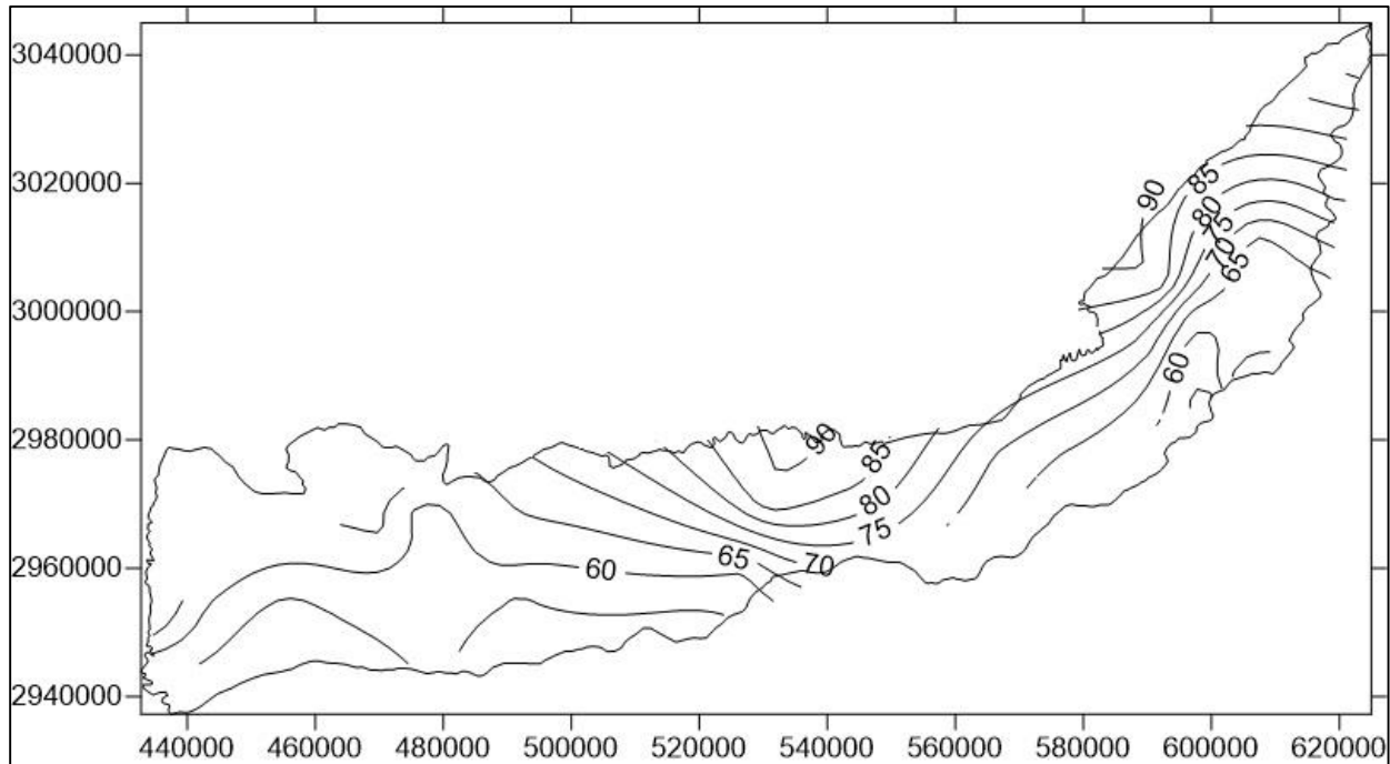
Fig3: Water Table Contour Map, Post-monsoon 2016
