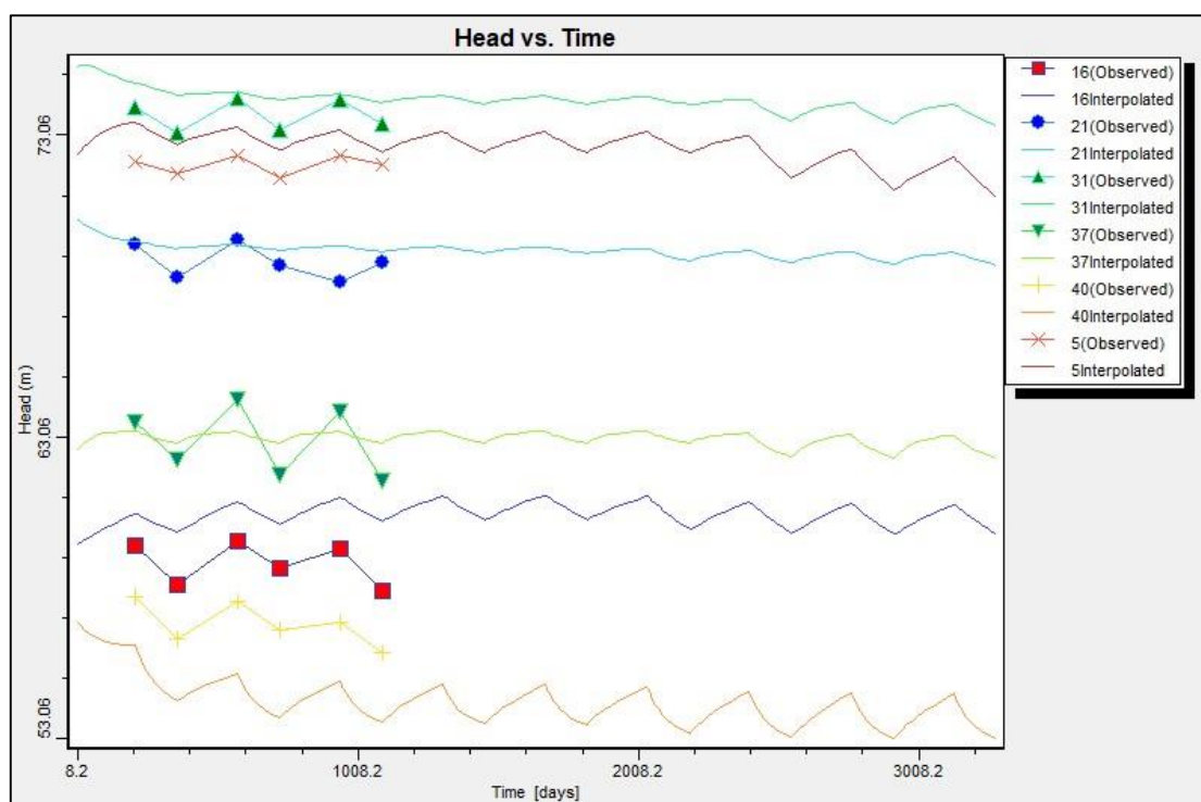
Fig 22: Behavior of well hydrographs up to 2025 under prediction scenario 2
