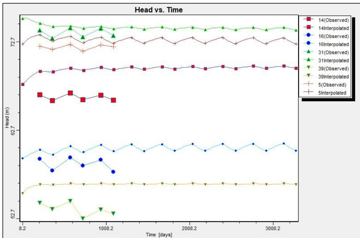
Fig 20: Behaviour of well hydrographs up to 2021 under prediction scenario 1.
