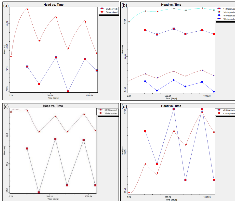
Fig 17: Head Vs Time (a) Well no.5, (b) Well No. 14 & 16, (c) Well no. 38 and (d) Well no. 42
