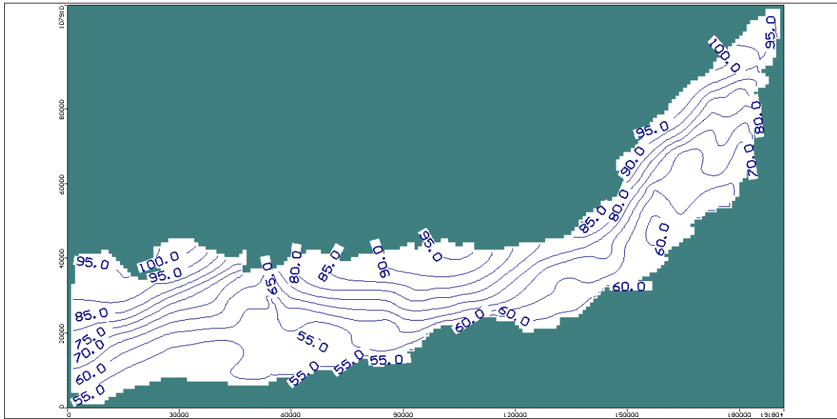
Fig12: Computed Head in Steady state.
