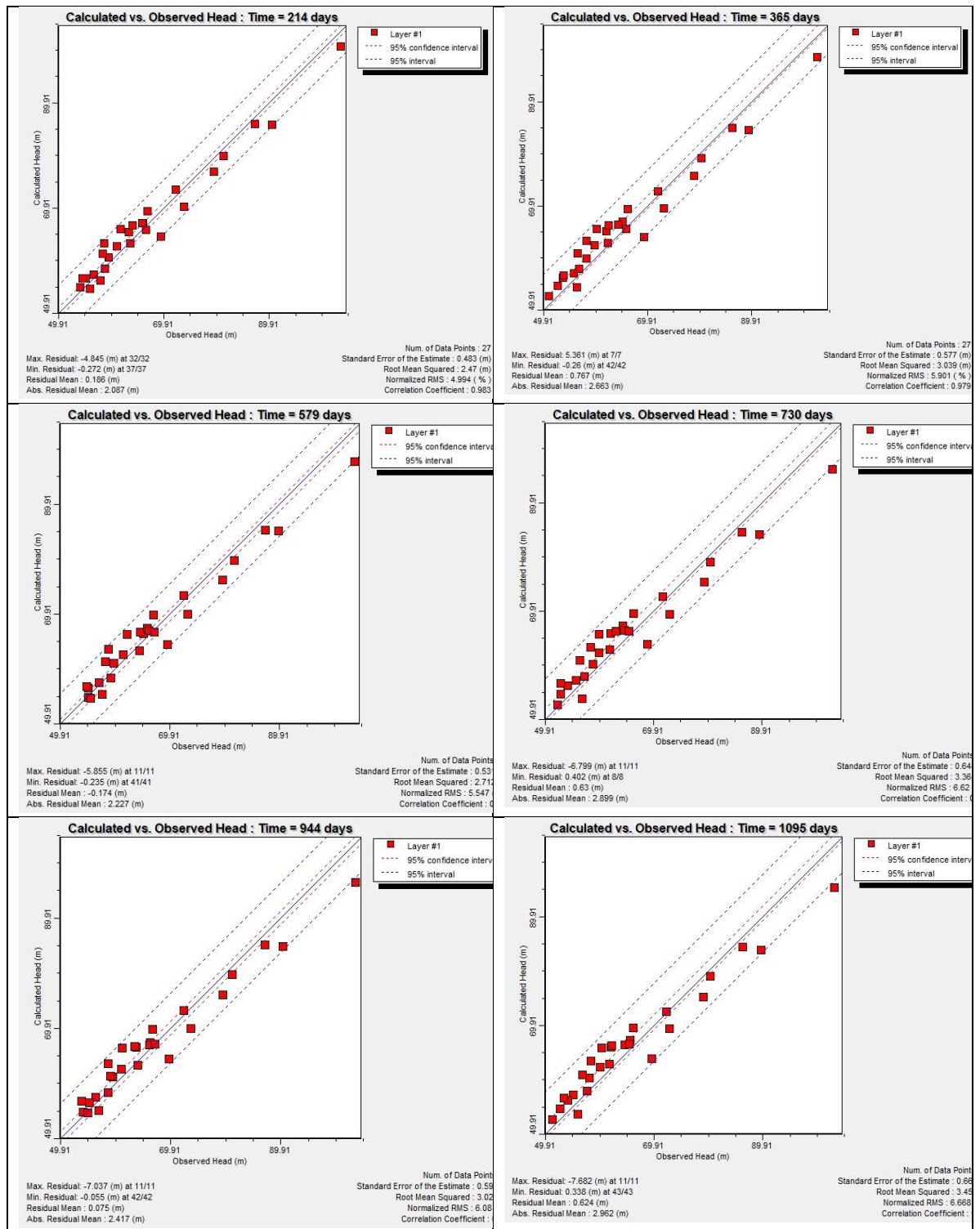
Fig 14: Head Scatter Graphs for Different Time Steps of Calibrated Model
