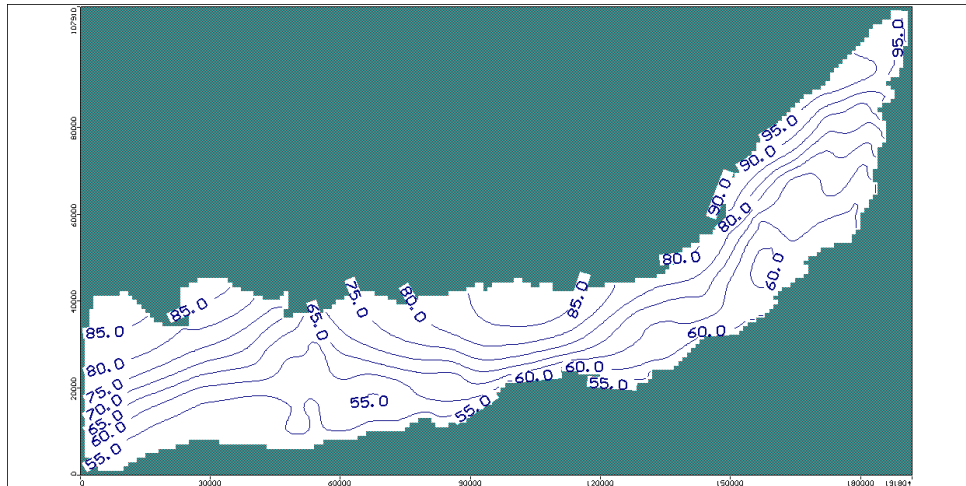
Fig15: Water level head generated after Transient Calibration
