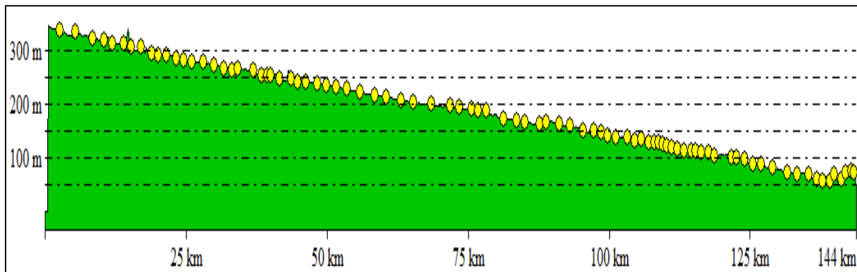
Fig-4.2: Musi River profile
