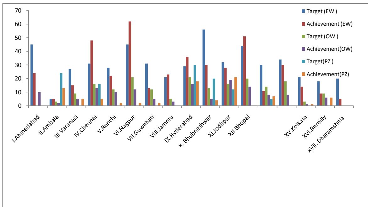
Fig 4.3 Showing Division wise status of Ground Water Exploration during 2013-14
