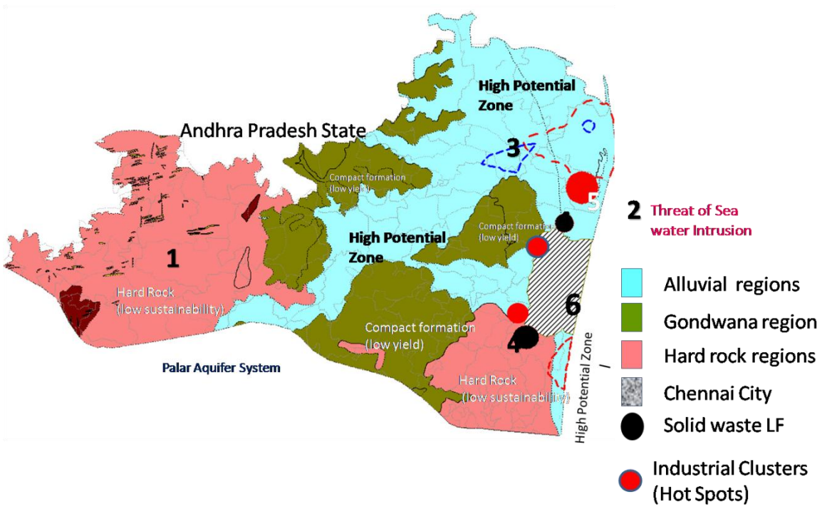
Figure 2: Regional hydrogeology of Chennai Aquifer System.
