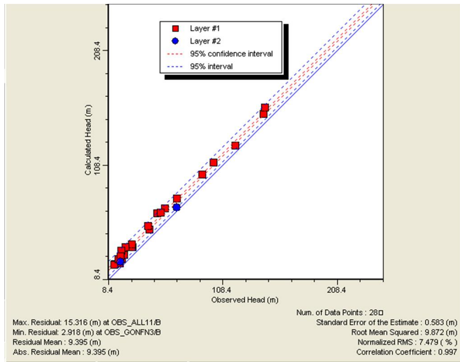
Figure 14a: Comparison of computed & observed GW head under steady state condition.
