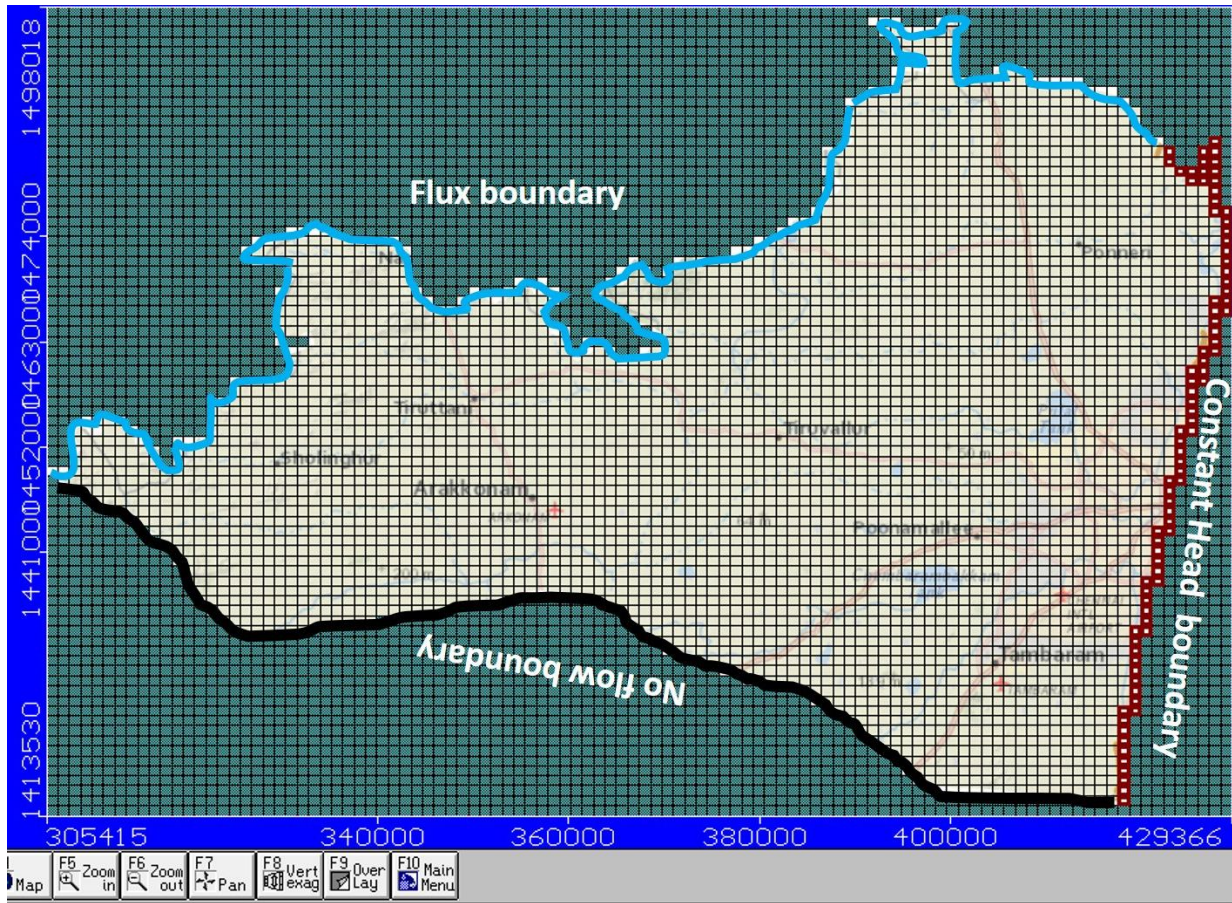
Figure 5 : Boundary conditions modeled for the Chennai aquifer system
