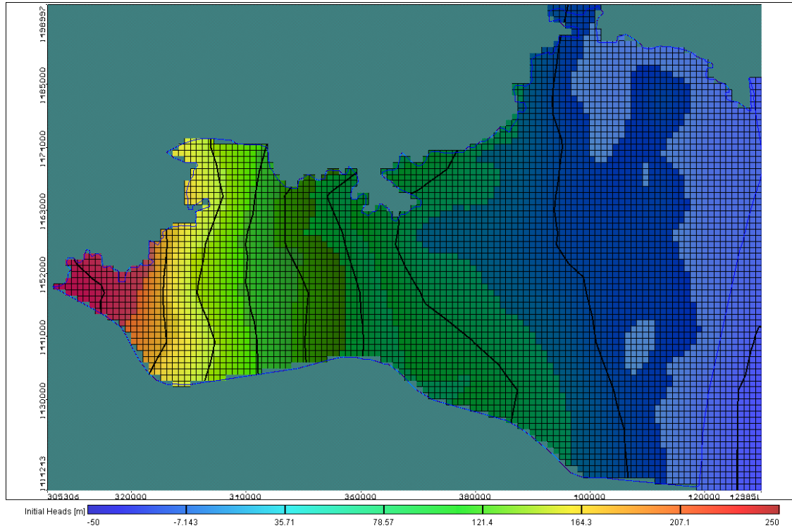
Figure 10: Initial groundwater head values used in the model for layer 1
