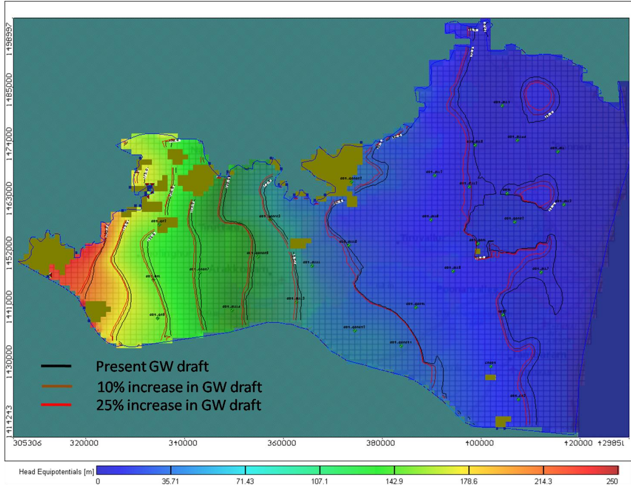
Figure18. Projected GW heads during 2025 with present and increase in GW draft.
