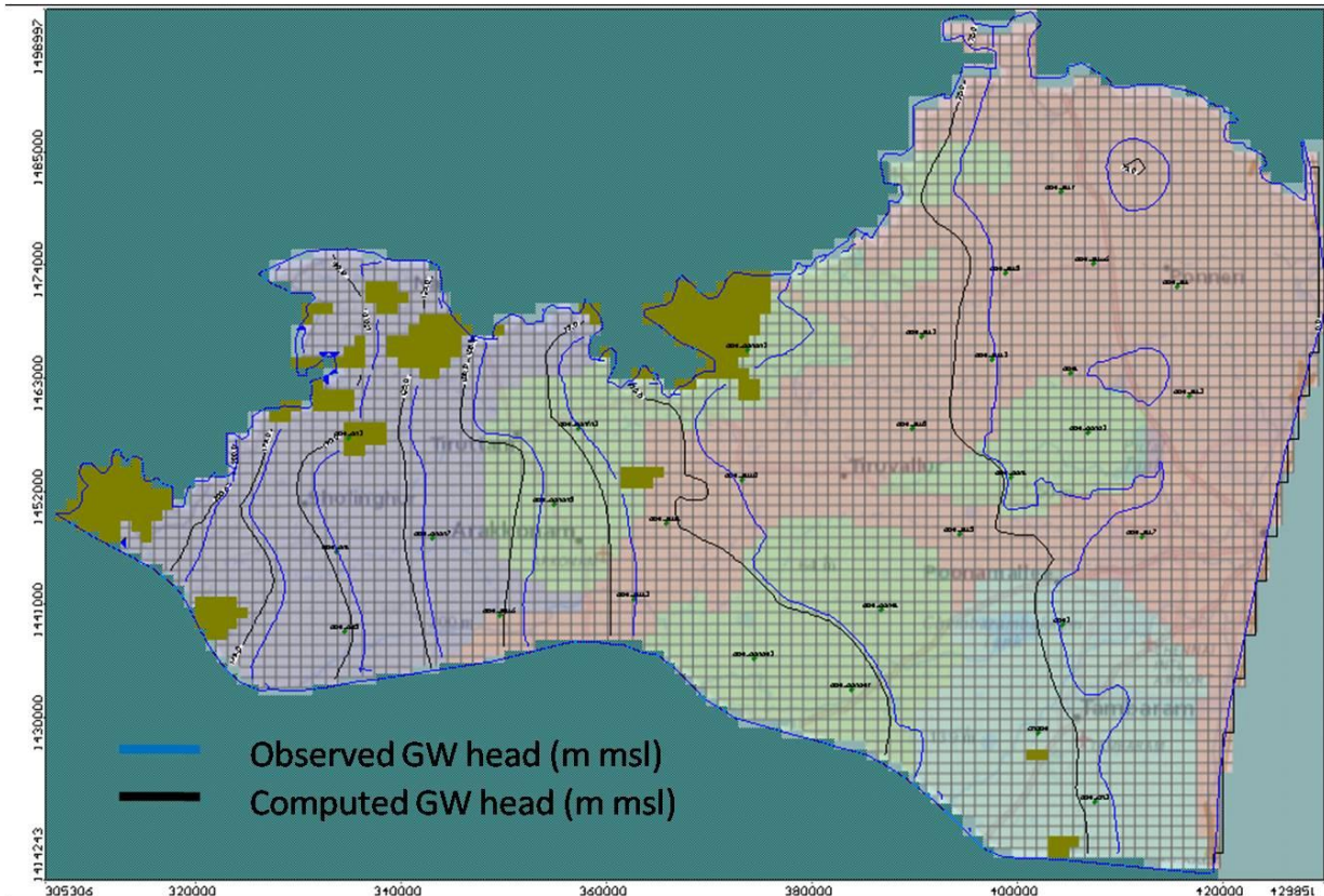
Figure15: Simulated and observed groundwater head during May 2014.
