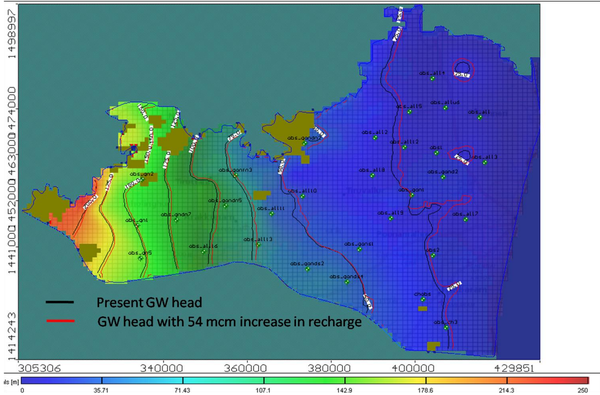
Figure 19. Projected GW heads with 54 mcm increase in recharge during 2025.
