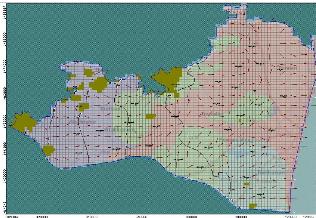
Figure16a: Groundwater flow vectors during May 2014.
