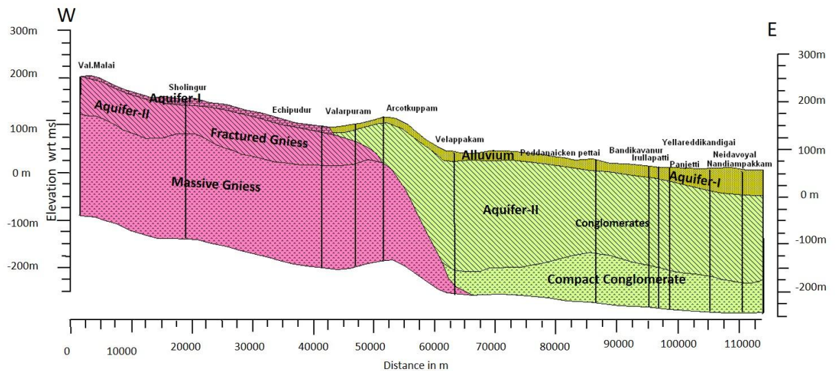
Figure 4a: Cross-section along West-East of Chennai aquifer system.
