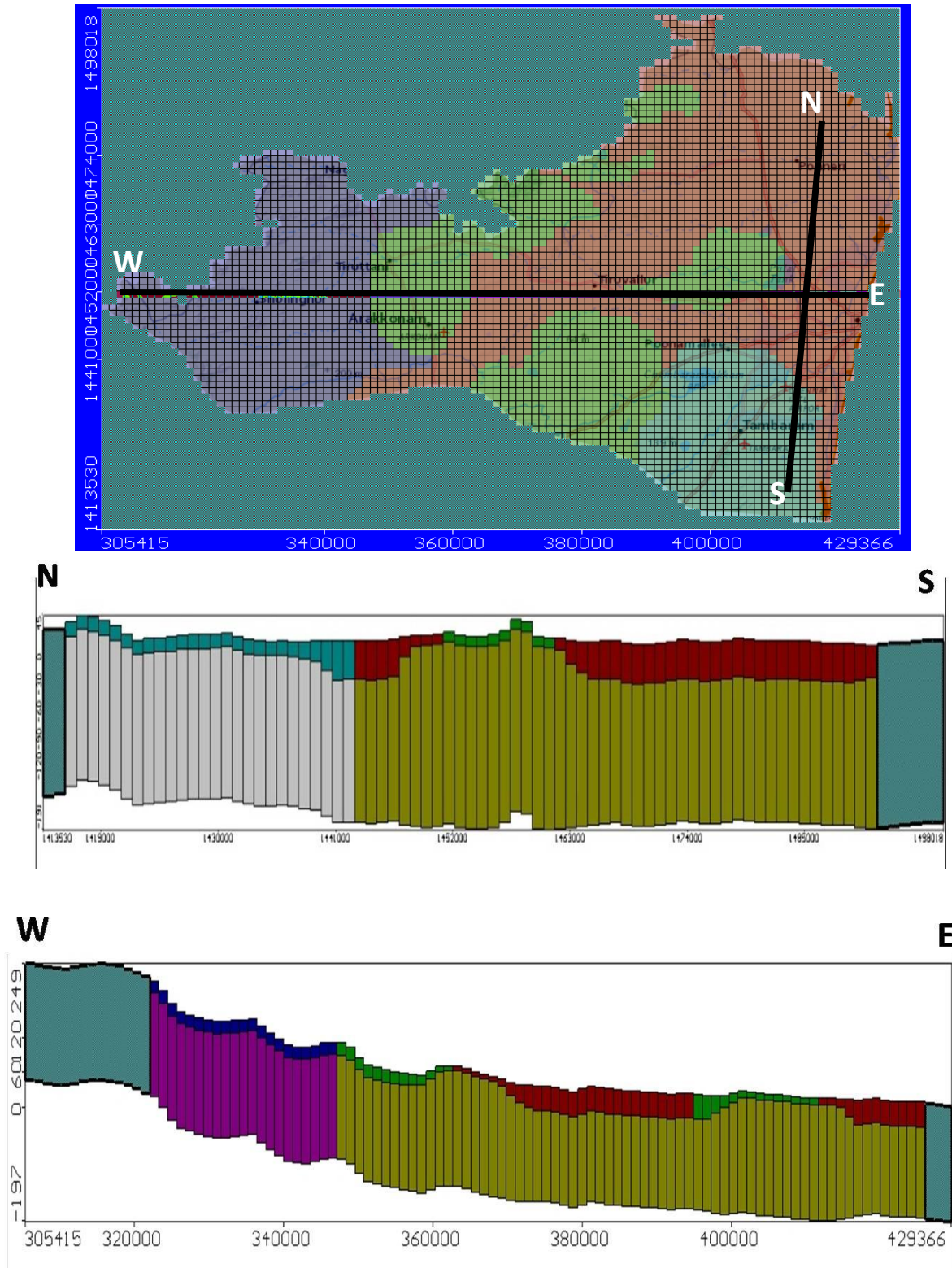
Figure 6: Grid Design of the Chennai aquifer system and vertical layer design along North South & West East direction
