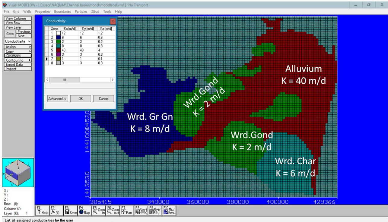
Figure 8a: Hydraulic conductivity values used in the model for layer 1.
