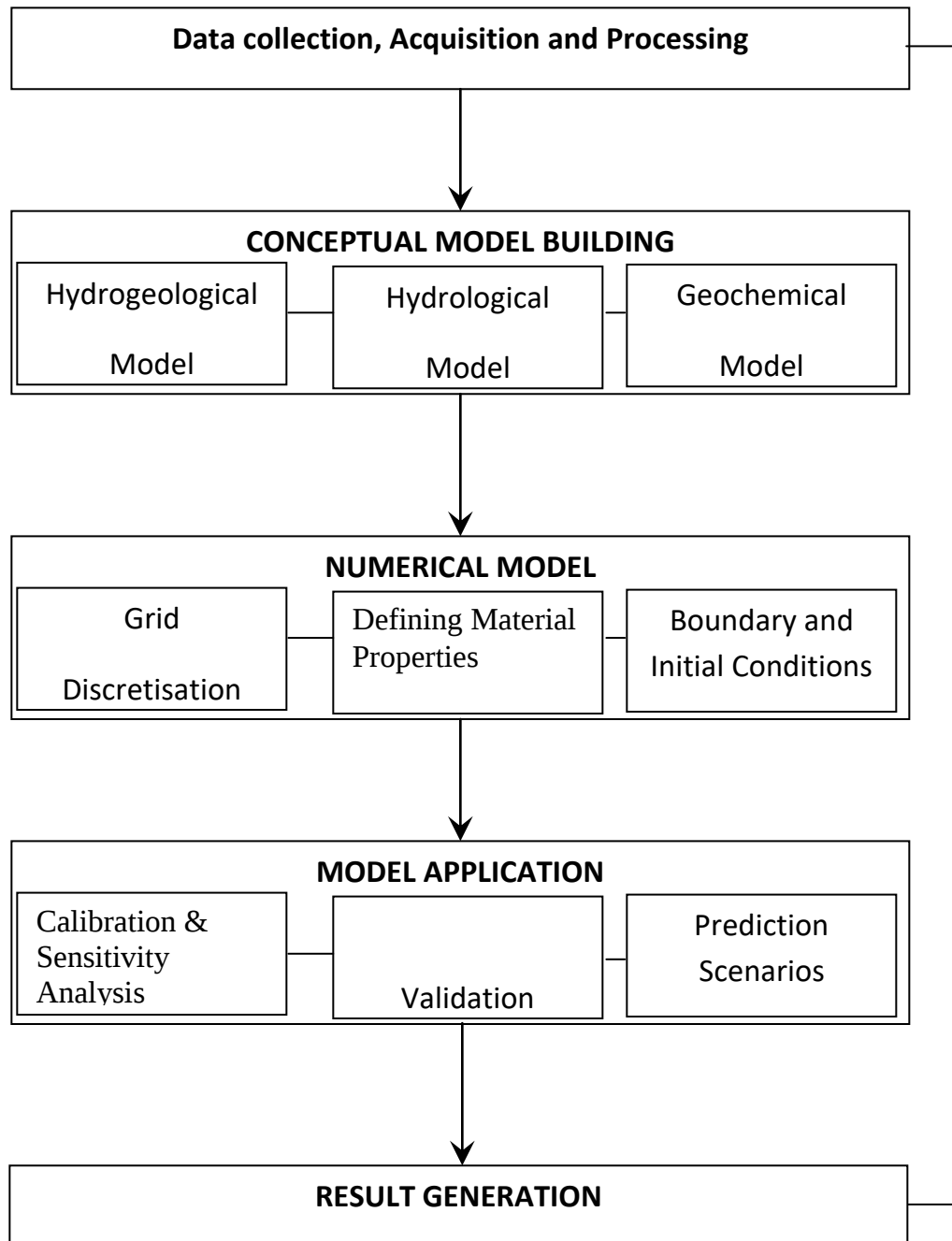
Figure13: Flowchart of the groundwater modeling of Chennai aquifer system
