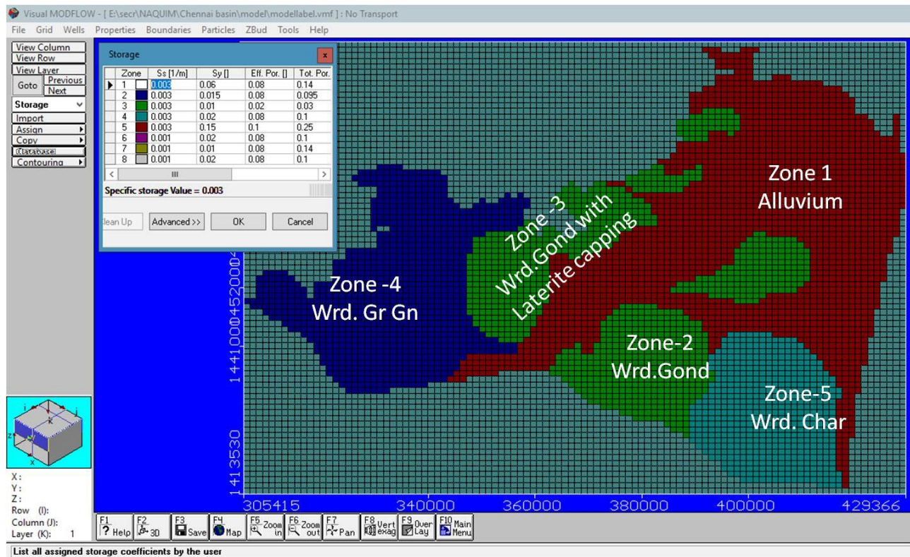
Figure12: Groundwater recharge zones of the model area
