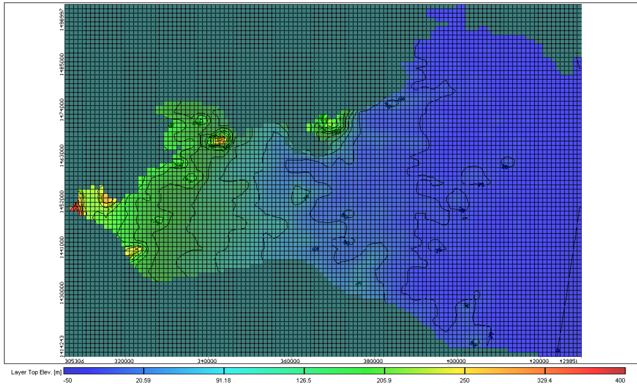
Figure 7a: Top elevation of the study area
