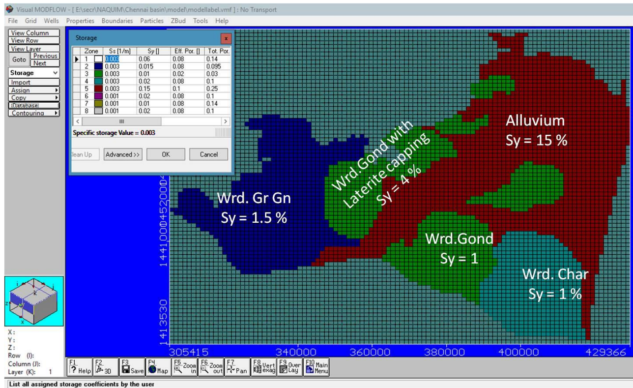
Figure 9: Specific yield values used in the model for layer 1
