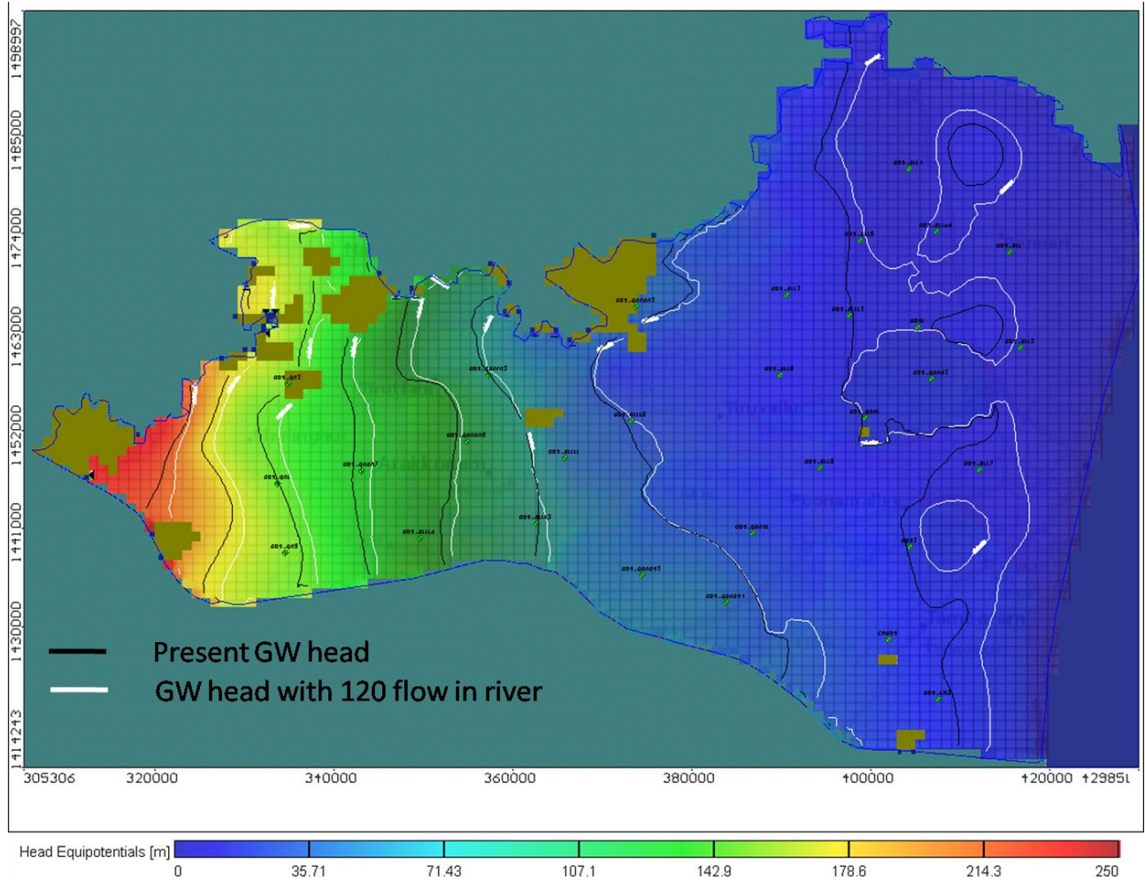
Figure 21: Projected GW heads with 120 days flow in rivers and construction of canal connecting Arani and Korratalaiyar river during 2025.
