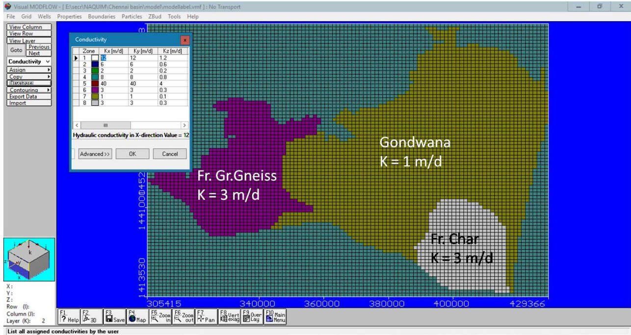
Figure 8b: Hydraulic conductivity values used in the model for layer 2
