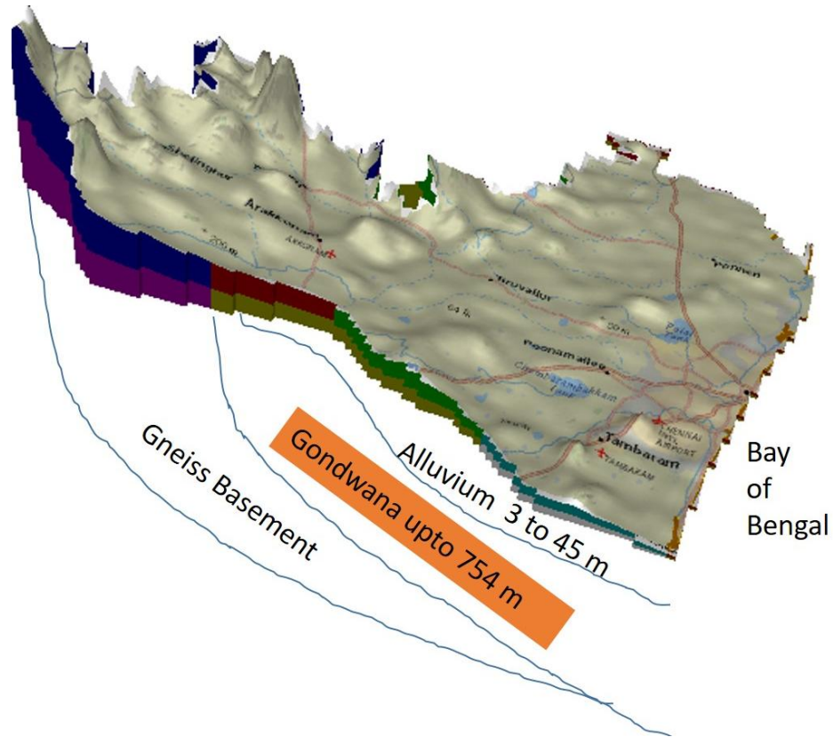
Figure 4 : Conceptual setup of Chennai Aquifer System.
