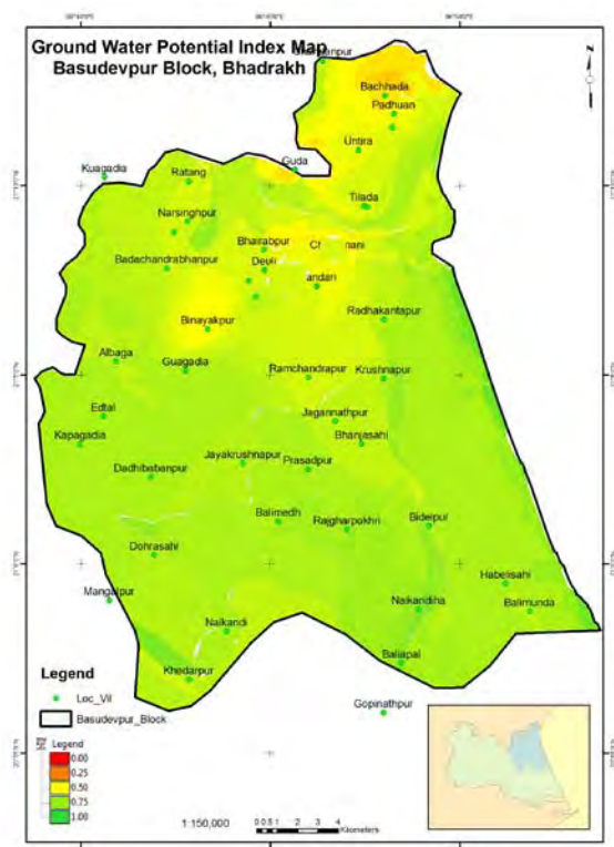
Figure-2: Ground Water Potential Map of Basudevpur Block, bhadrakh District, Orissa
