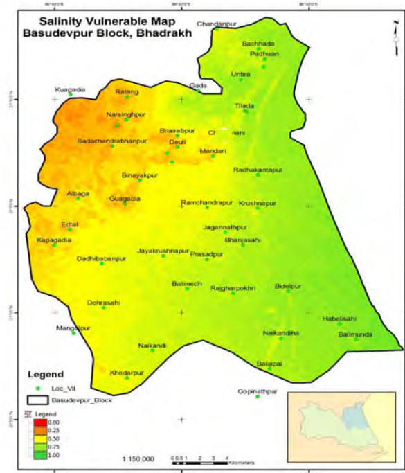
Figure-1: Salinity vulnerable Map of Basudevpur Block, Bhadrakh District, Orissa, Generated through spatial data analysis.
