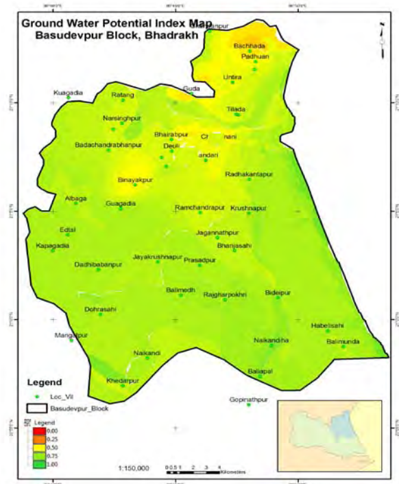
Figure-2: Ground Water Potential Map of Basudevpur Block, bhadrakh District, Orissa
