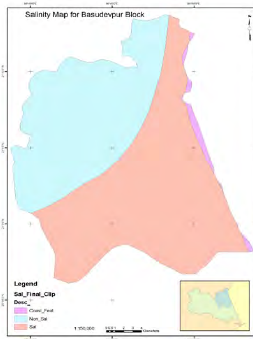
Figure-1(a) Existing Hydrogeological Map showing saline-non saline areas based on ground water exploration, Basudevpur Block, Bhadrakh District
