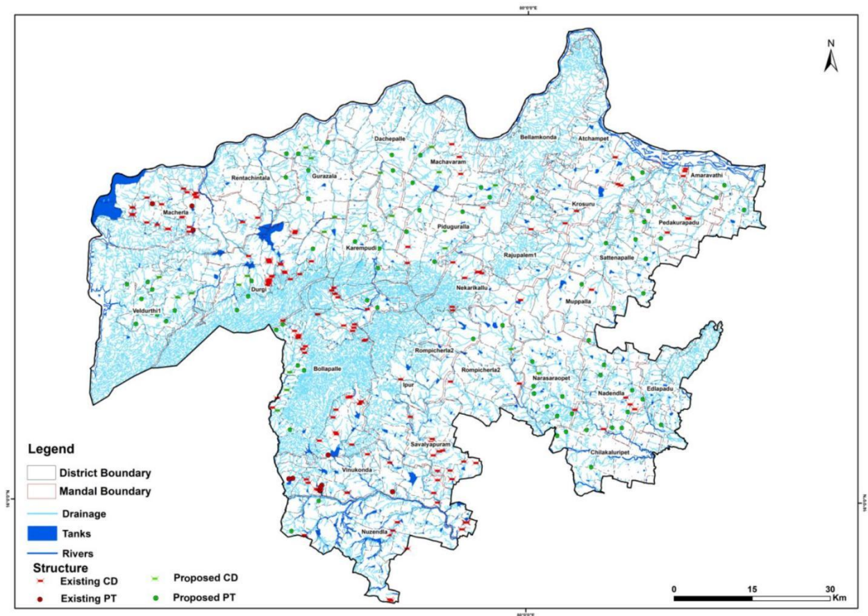
Fig 6.2: Existing and Proposed Artificial Recharge Structures
