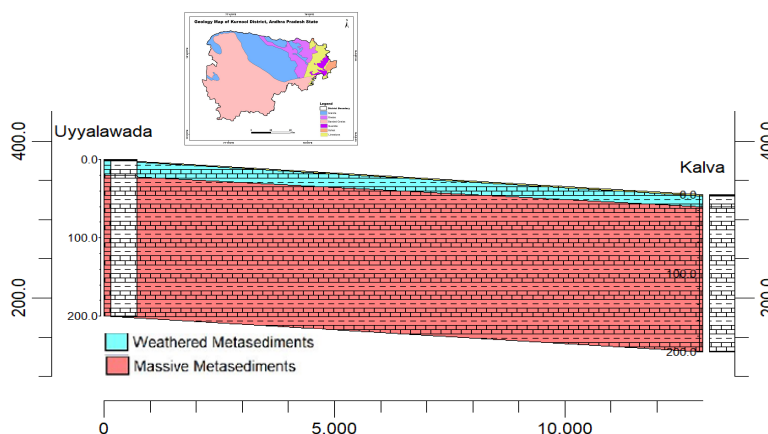
Figure 3.4 - Hydrogeological cross section across the meta sedimentary formation
