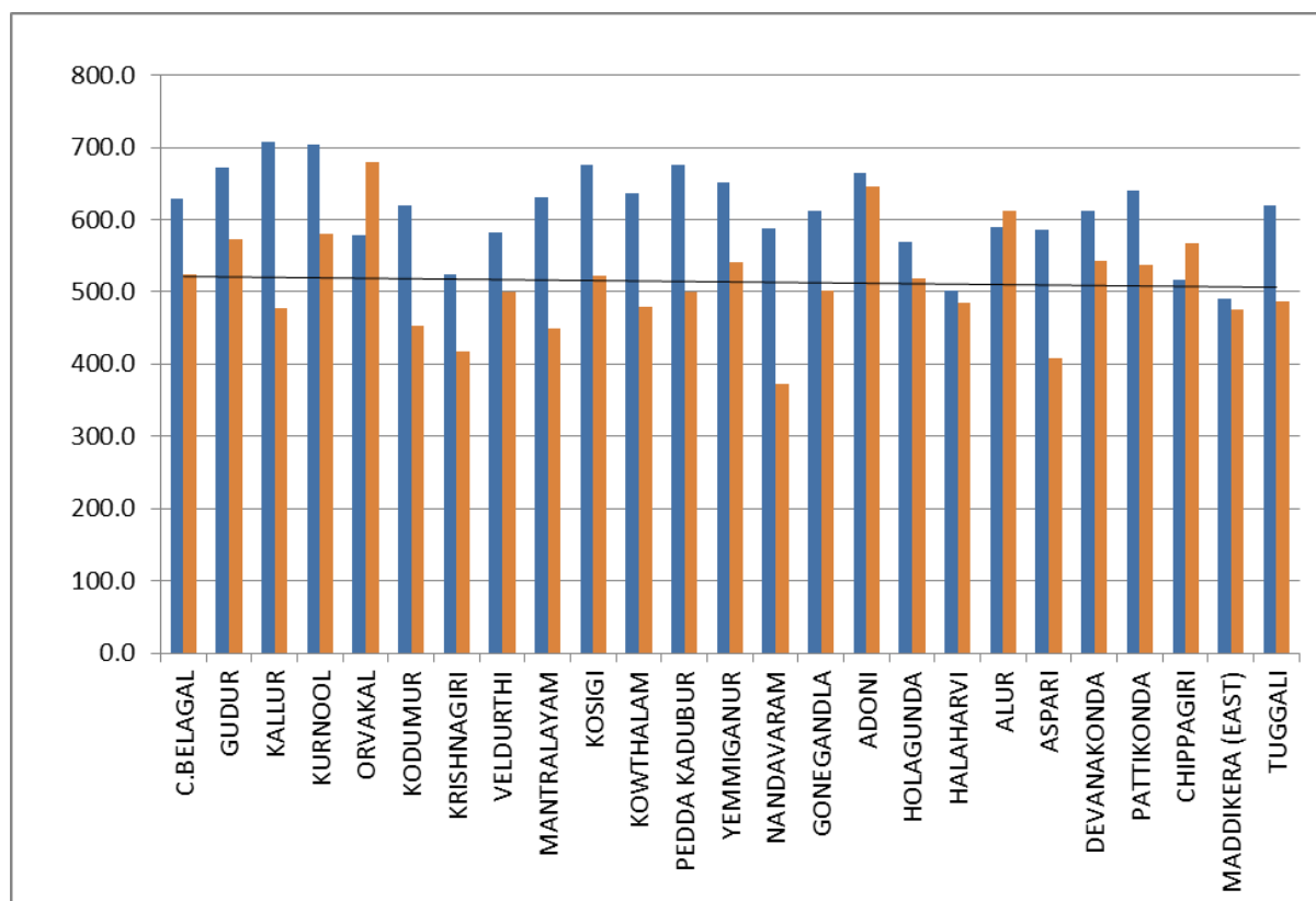
Figure 1.2 Normal Rainfall Vs Actual Rainfall (2019-20) in mm
