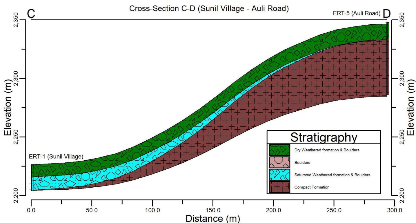
Figure – 12 D- Lithological section from Sunil Village to Auli Road, Joshimath, Chamoli District
