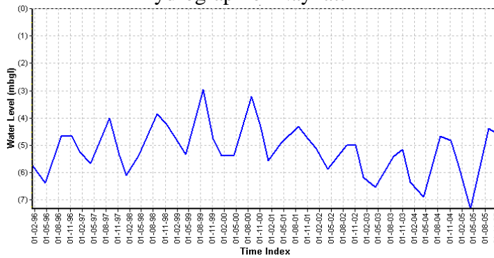
Hydrograph of Naykatti
