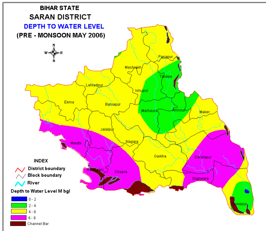
Fig 3. Pre-monsoon (May 2006) water level map of Saran district
