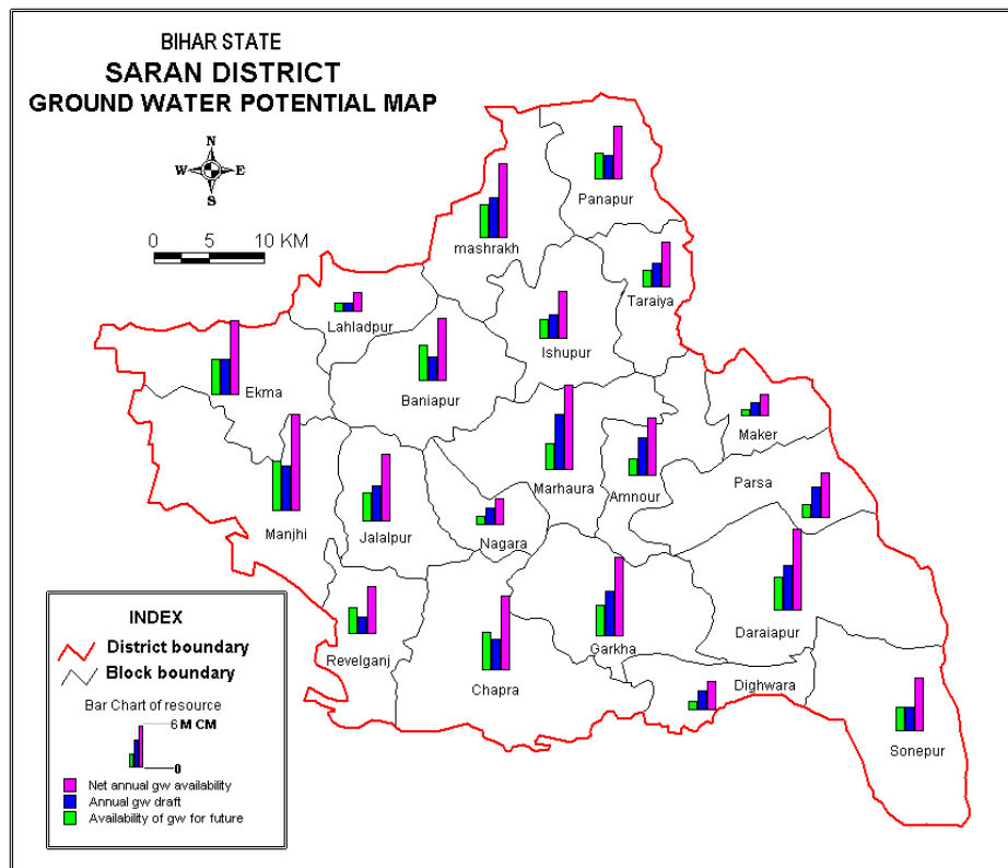
Fig 5. Ground water potential map of Saran district
