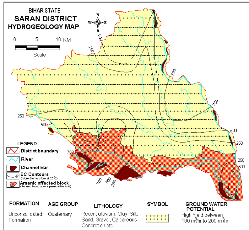
Fig 2. Hydrogeological map of Saran district Water Level Fluctuation
