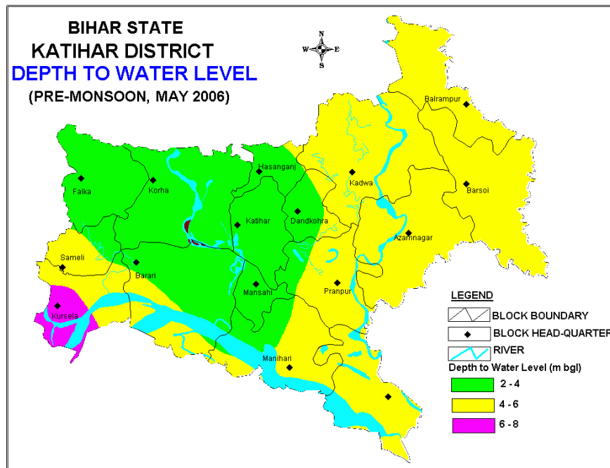
Fig 3: Pre-monsoon (May 2006) water level map of Katihar district
