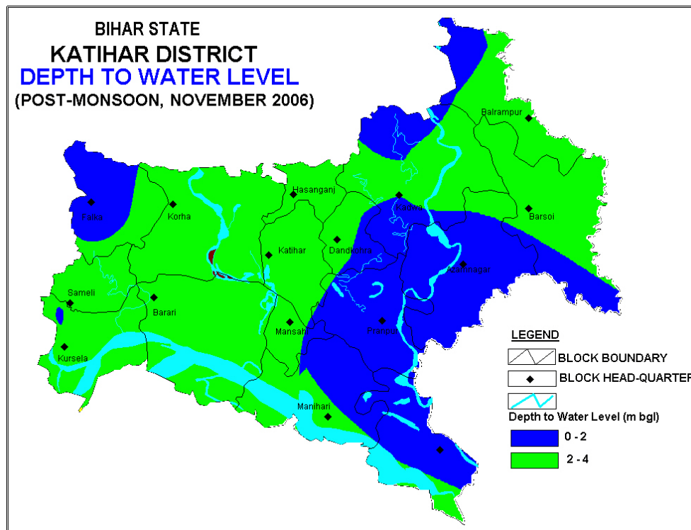
Fig 4: Post-monsoon (November 2006) water level map of Katihar district
