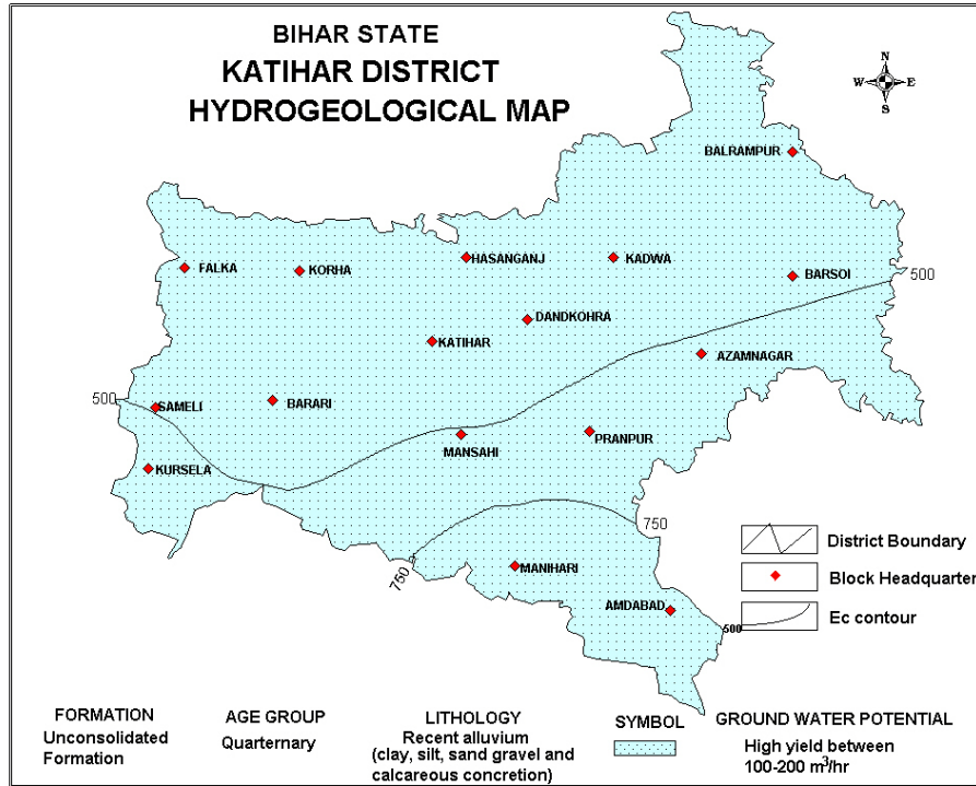
Fig 2: Hydrogeological map of Katihar district
