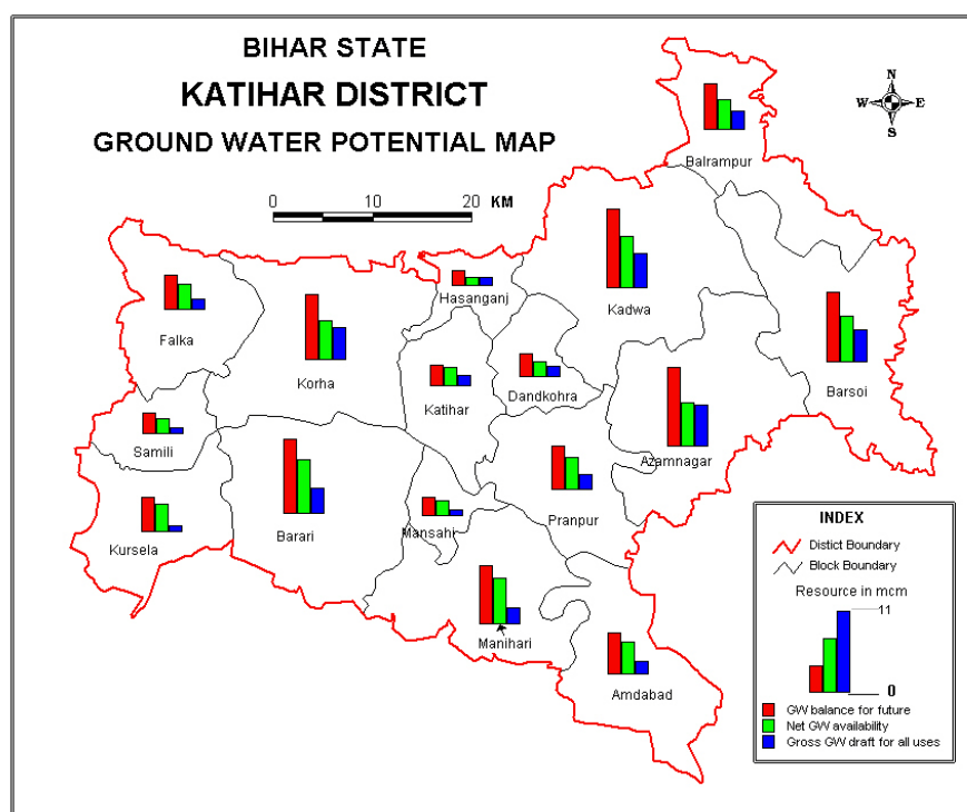
Fig 5: Ground Water potential Map of Katihar district
